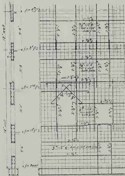
SECTION - TYPICAL WALL REINFORCING, \frac{1}{4} " Scale 1/4" = 1'-0"
