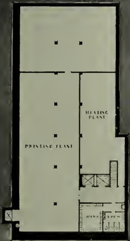
BASEMENT PLAN
