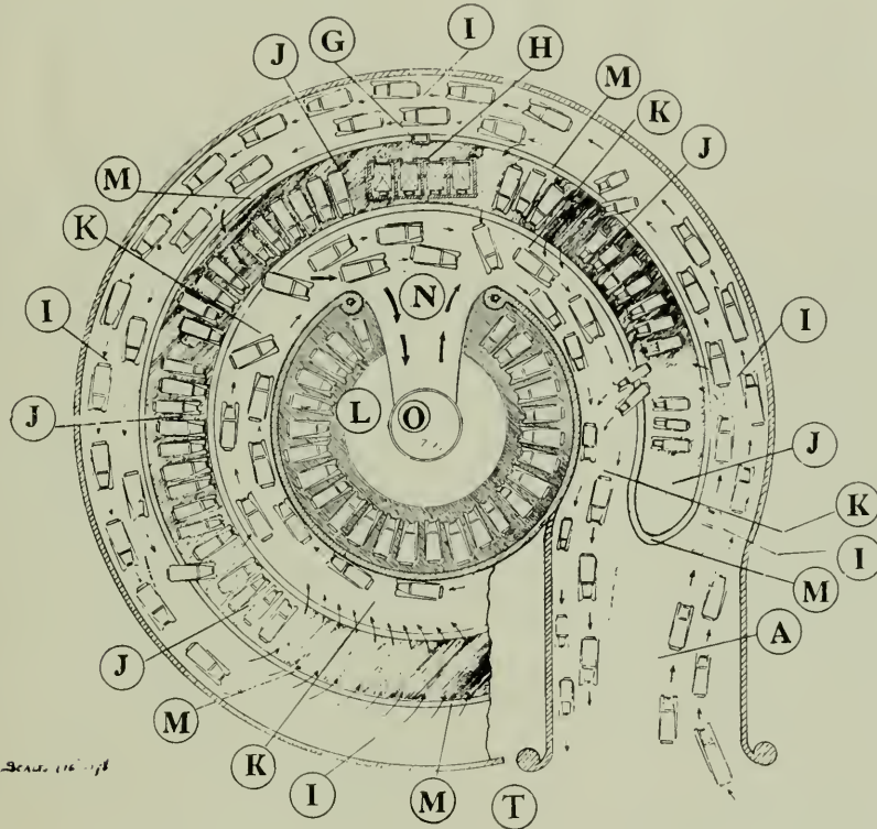
PLAN, PARKING SPIRAL
