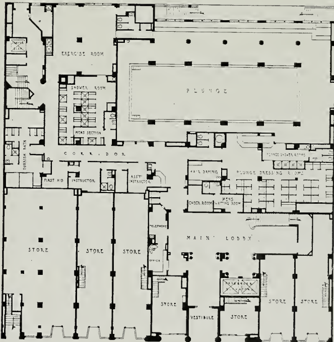
FIRST FLOOR PLAN, WOMEN'S ATHLETIC CLUB, LOS ANGELES Allison and Allison, Architects
