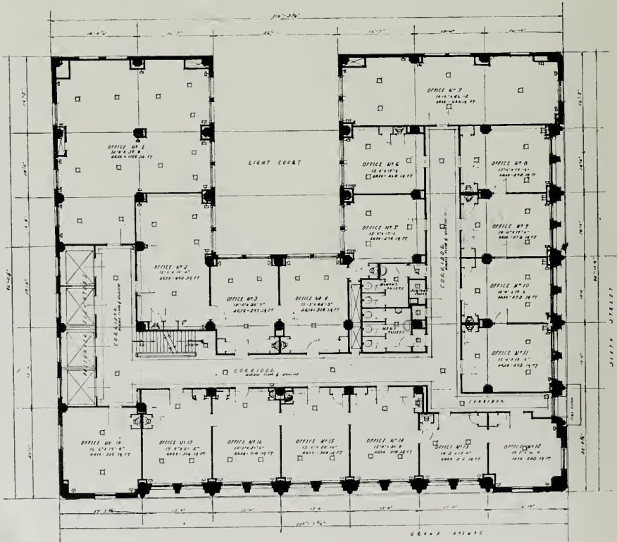
FIRST AND TYPICAL FLOOR PLANS, EDWARDS & WILDEY BUILDING, LOS ANGELES Walker and Eisen, Architects and Engineers
