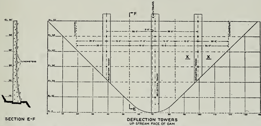
DRAWINGS SHOW PLANS FOR MAKING TESTS IN CONCRETE DAM TO BE BUILT IN FRESNO COUNTY FOR ENGINEERING FOUNDATION COMMITTEE ON ARCH DAM INVESTIGATION
