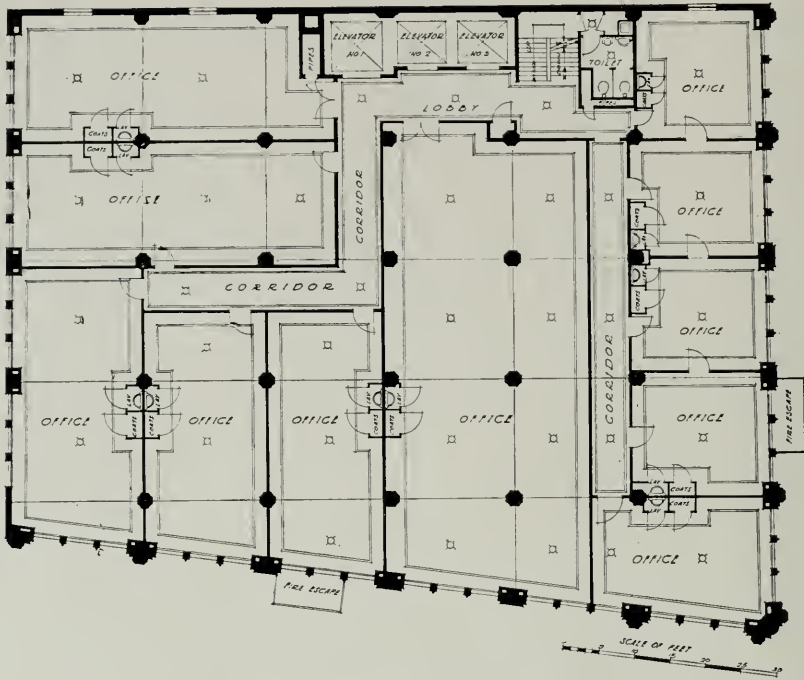
TYPICAL OFFICE PLAN, TRANSPORTATION BUILDING, LOS ANGELES Walker and Eisen, Architects and Engineers
