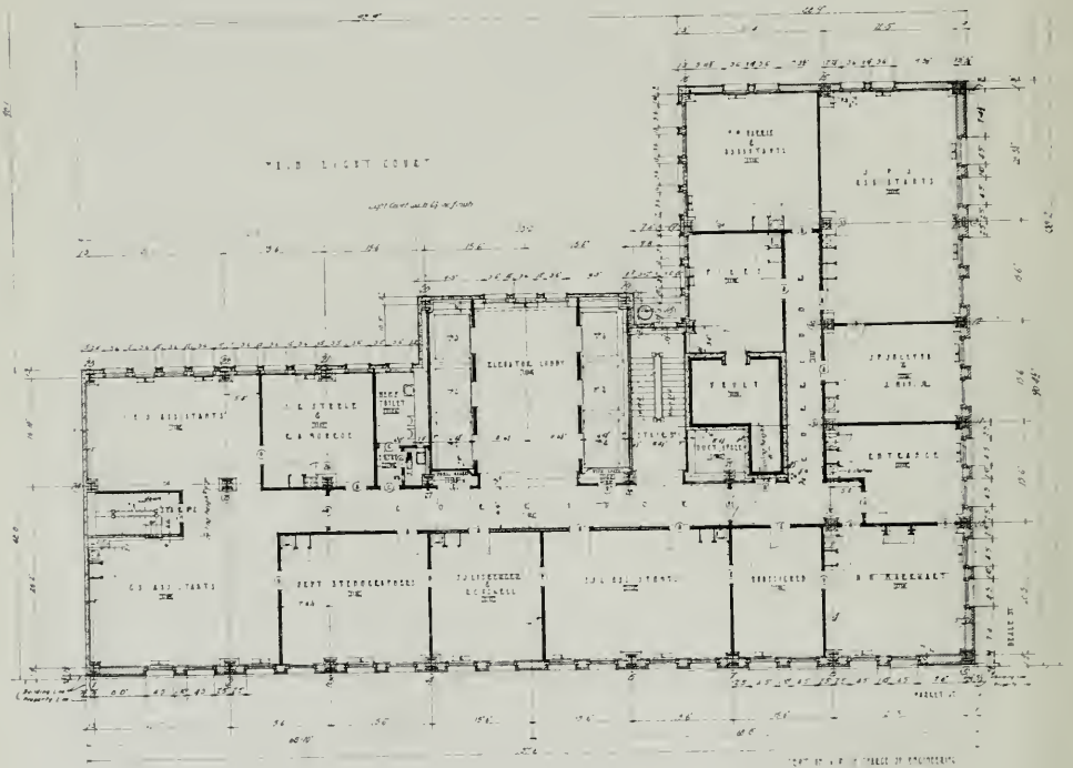
TYPICAL FLOOR PLAN, P. G. & E. BUILDING, SAN FRANCISCO Bakewell and Brown, Architects
