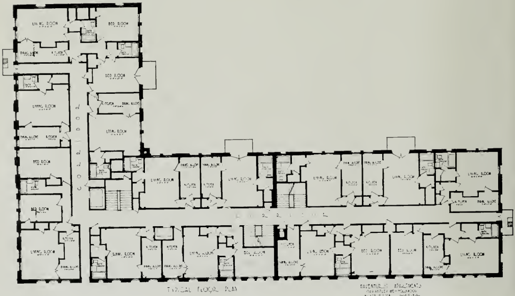
TYPICAL FLOOR PLAN, HAVENHURST APARTMENTS, HOLLYWOOD Walker and Eisen, Architects and Engineers
