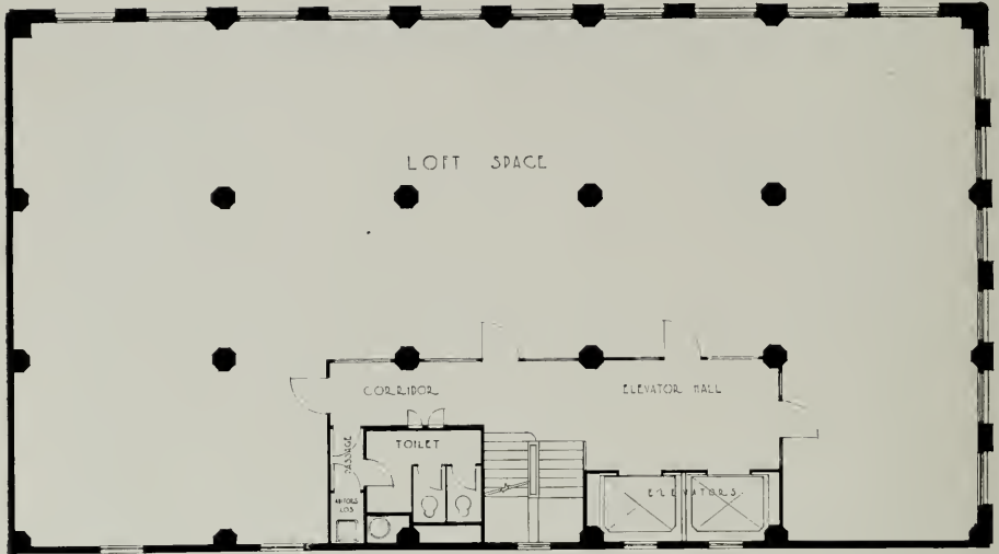
TYPICAL FLOOR PLAN, BUILDERS EXCHANGE BUILDING, LOS ANGELES Walker and Eisen, Architects and Engineers
