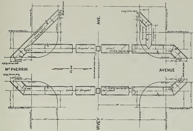
(Fig. 7) LAYOUT FOR MONTEREY PARK PART CIRCLE, SHOWING STREET INTERSECTION
