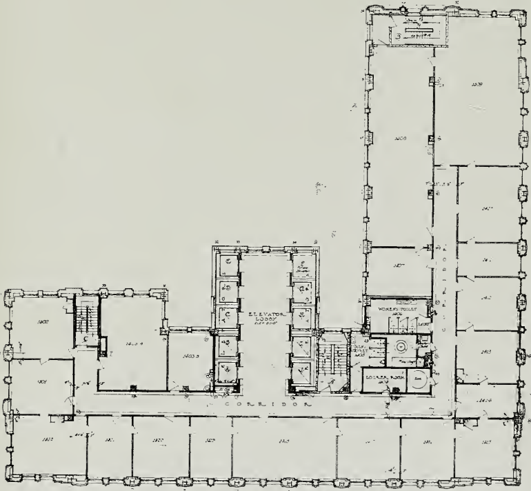
PLAN, FOURTEENTH FLOOR, TELEPHONE BUILDING, SAN FRANCISCO J. R. Miller and T. L. Pflueger, A. A. Cantin, Associated Architects
