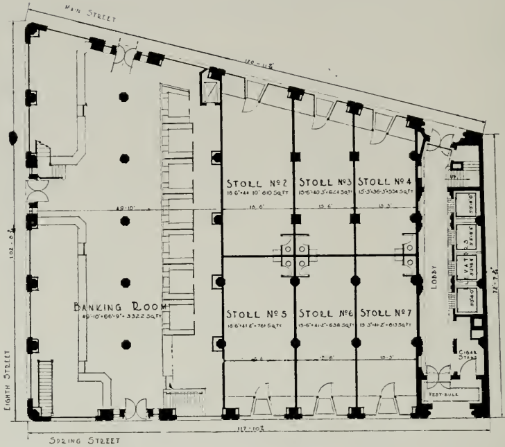
FIRST FLOOR PLAN, NATIONAL CITY BANK BUILDING, LOS ANGELES Walker and Eisen, Architects and Engineers
