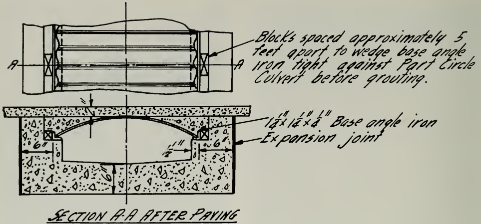
(Fig. 3) PART CIRCLE INSTALLATION DETAILS, SHOWING CROSS SECTION OF TYPICAL PART CIRCLE INSTALLATION
