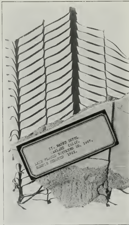
SPECIMEN OF LATH MADE OF ARMCO INGOT IRON, REMOVED FROM WALL OF ST. MARKS HOTEL, OAKLAND. NO EVIDENCE OF CORROSION AFTER SIXTEEN YEARS
