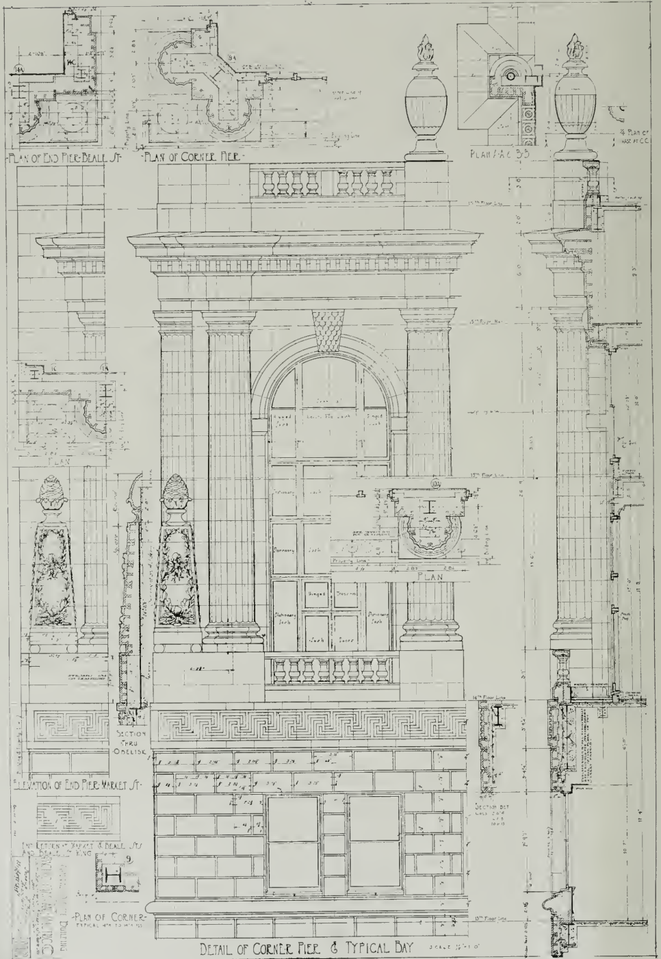
P. G. & E. BUILDING, SAN FRANCISCO BAKEWELL AND BROWN, ARCHITECTS
