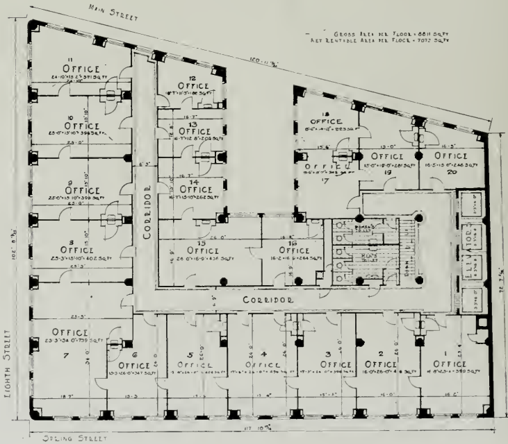
TYPICAL FLOOR PLAN, NATIONAL CITY BANK BUILDING, LOS ANGELES Walker and Eisen, Architects and Engineers
