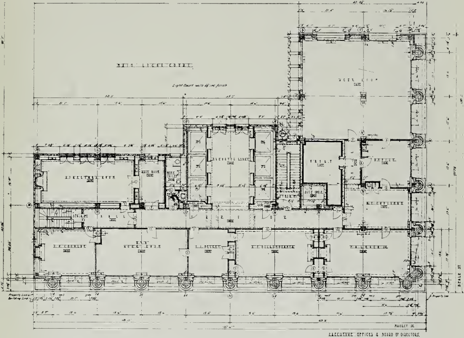
PLAN, EXECUTIVE OFFICES, P. G. & E. BUILDING
