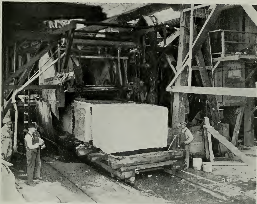
THIS GRANITE CUTTING MACHINE CUTS EIGHT FEET OR 160 SQUARE FEET AN HOUR. THE GRANITE BLOCKS SHOWN IN THE PICTURE ARE FIVE FEET HIGH
