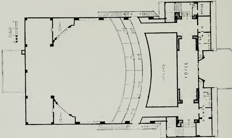
Mezzanine Floor
