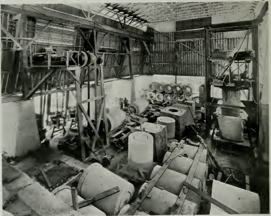
BORING AND CORING MILL. COLUMNS ARE CUT IN THIS ROOM BY HUGE MACHINES WHICH CUT AT THE AVERAGE SPEED OF ONE FOOT AN HOUR
