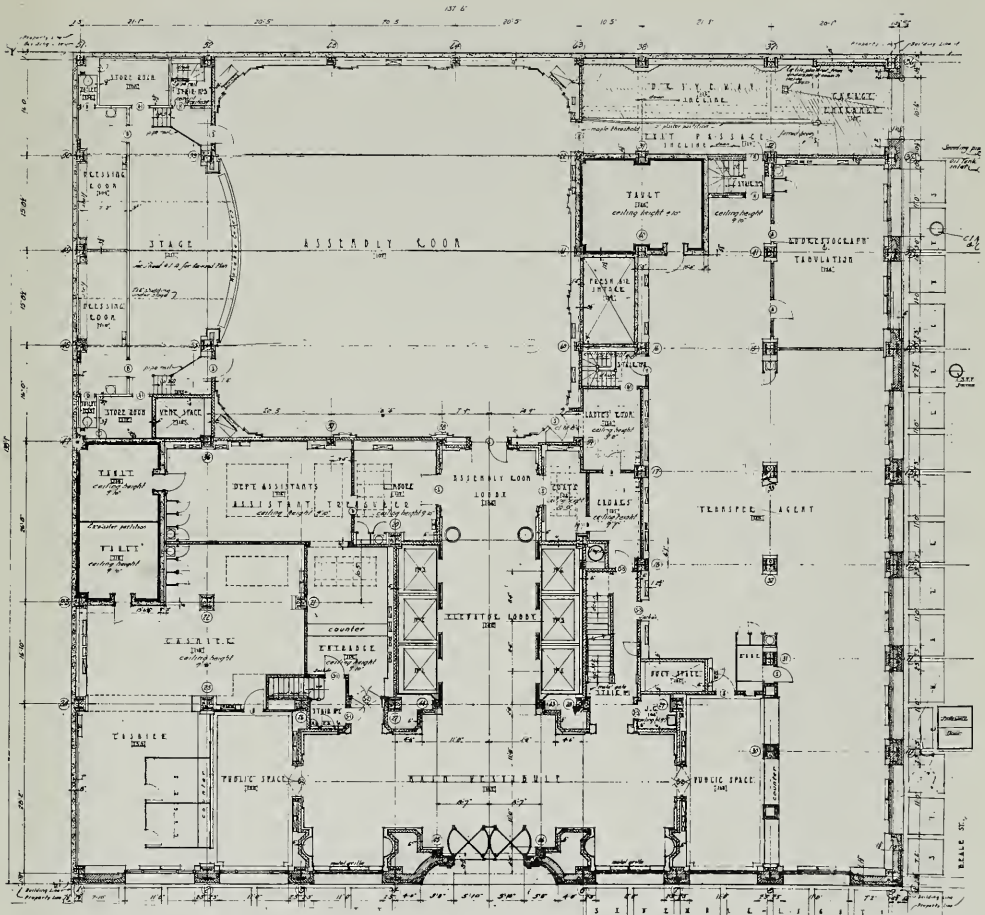
ASSEMBLY HALL FLOOR PLAN, P. G. & E. BUILDING Bakewell and Brown, Architects
