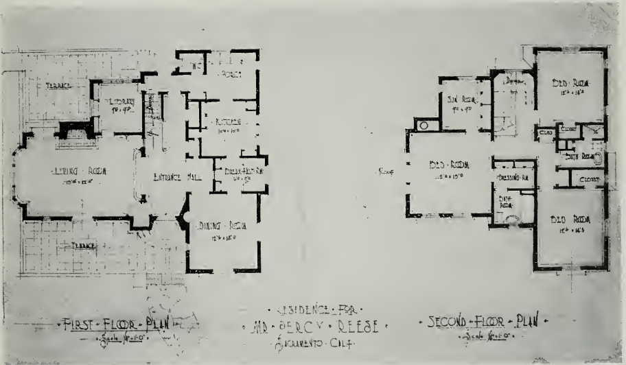
PLANS, HOUSE FOR MR. PERCY REESE, SACRAMENTO Leonard F. Starks & Co., Architects Edw. F. Flanders, Associate
