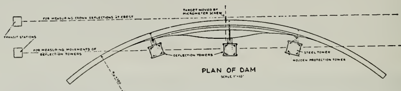
PLAN OF TEST ARCH DAM BEING BUILT IN FRESNO COUNTY
