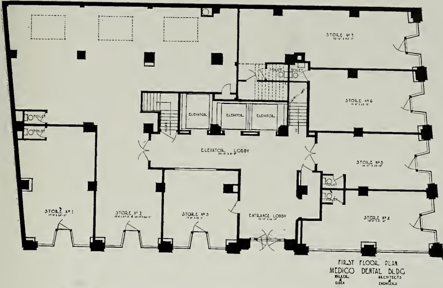
FIRST FLOOR PLAN, MEDICO-DENTAL BUILDING, LOS ANGELES Walker and Eisen, Architects and Engineers
