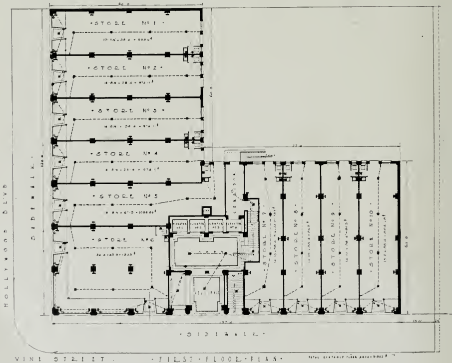
FIRST FLOOR PLAN, TAFT BUILDING, HOLLYWOOD Walker and Eisen, Architects and Engineers
