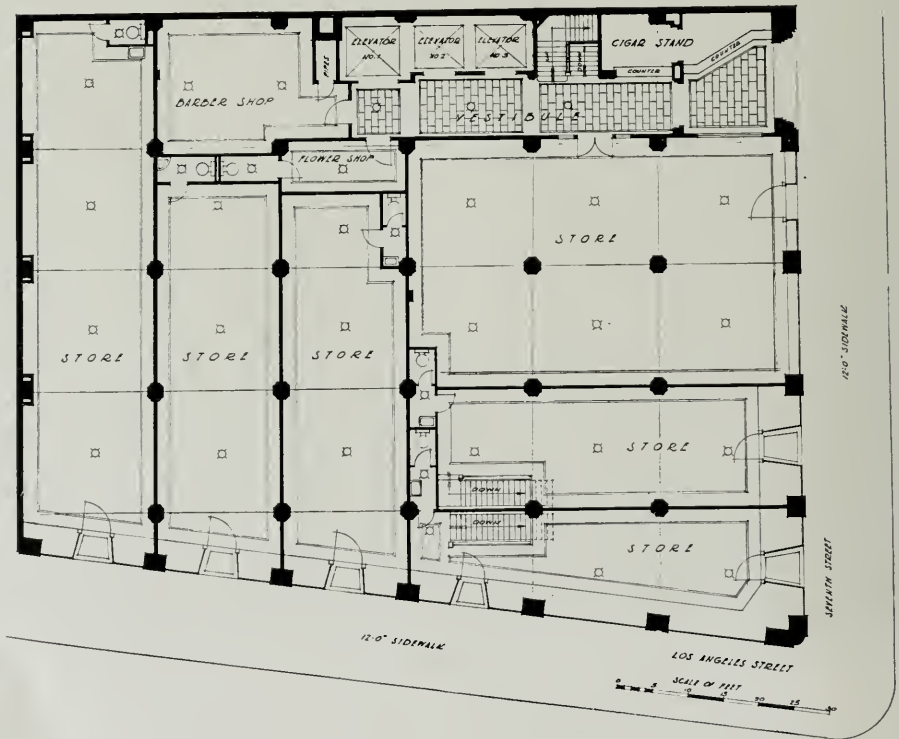
FIRST FLOOR PLAN, TRANSPORTATION BUILDING, LOS ANGELES Walker and Eisen, Architects and Engineers
