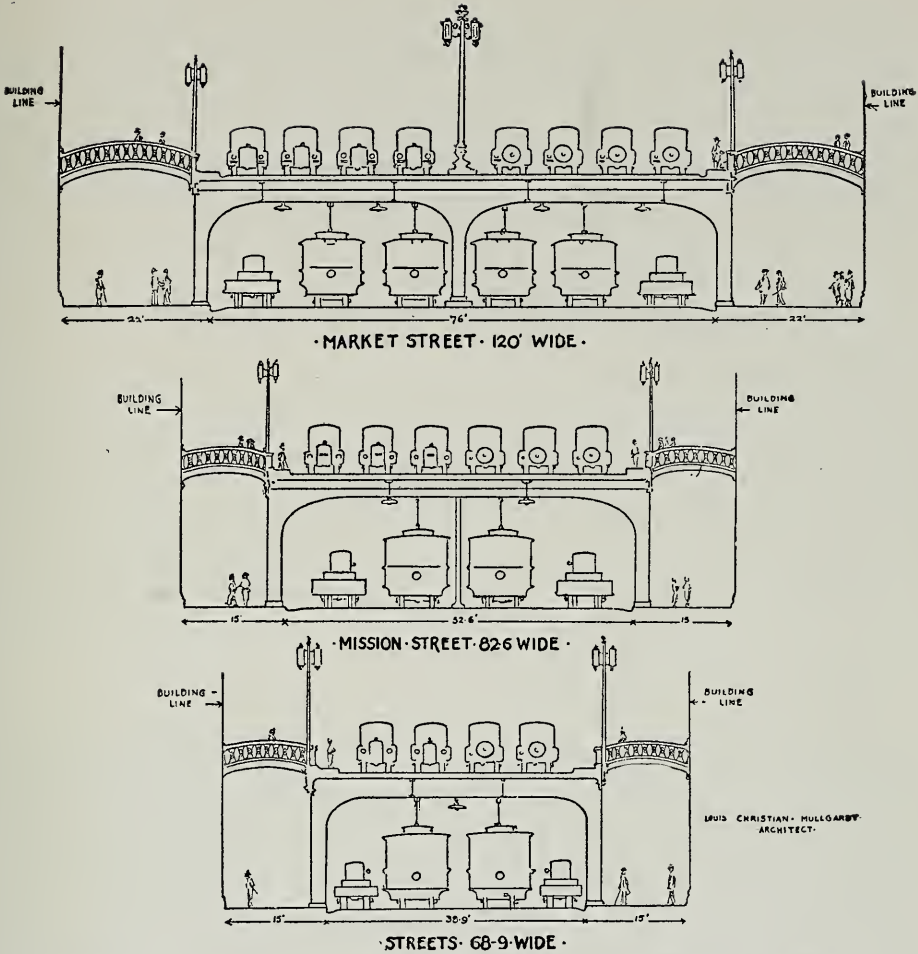
CROSS SECTION SHOWING NEW TRAFFIC PLAN FOR MARKET STREET, SAN FRANCISCO
