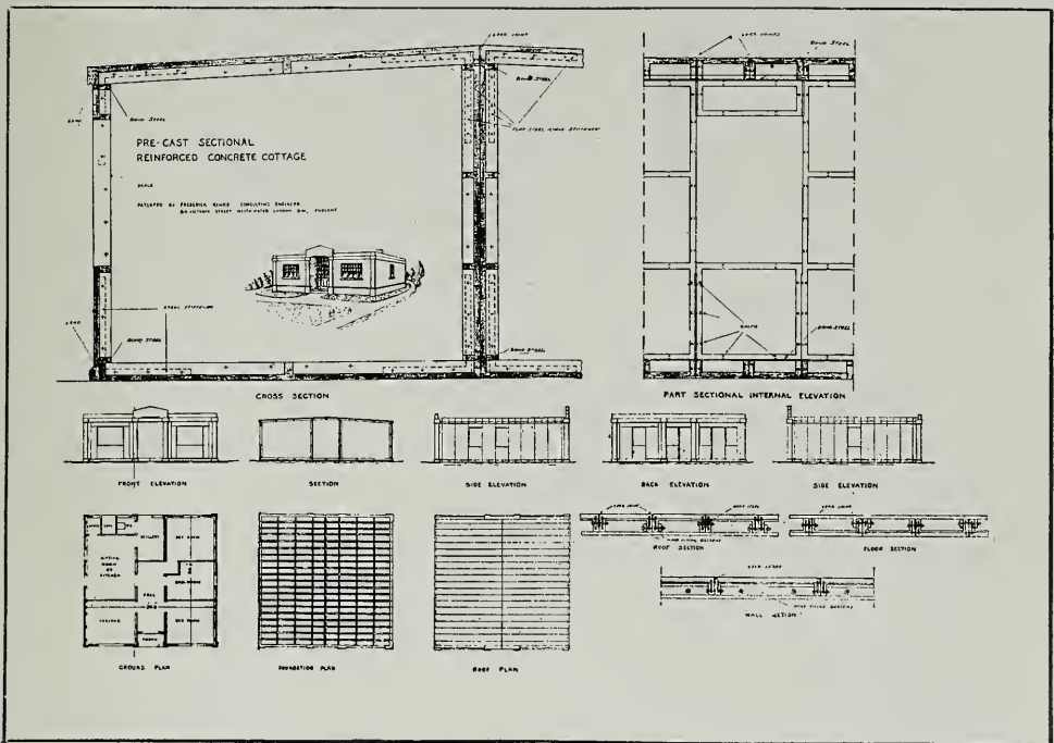
PLANS, SECTIONS AND DETAILS OF PRE-CAST SECTIONAL REINFORCED CONCRETE COTTAGE PATENTED IN ENGLAND
