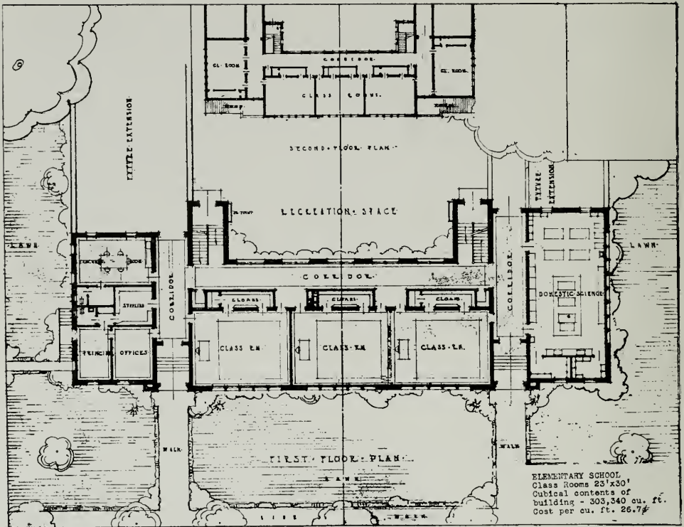
PLAN, FIFTY-SECOND STREET ELEMENTARY SCHOOL, LOS ANGELES A. M. Edelman and A. C. Zimmerman, Associate Architects Awarded Certificate of Honor by Southern California Chapter, A. I. A.
