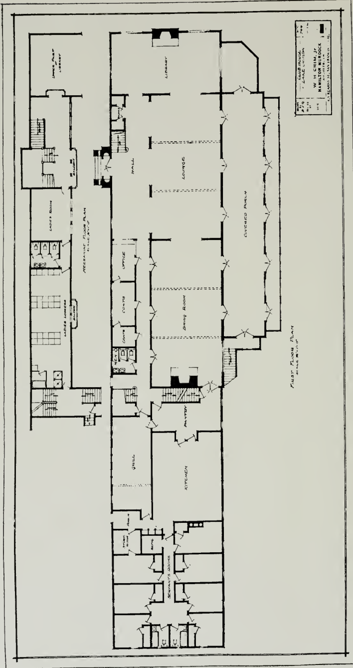
FIRST FLOOR PLAN, ORINDA COUNTRY CLUB, ALAMEDA COUNTY W. H. CRIM, JR., AND HAMILTON MURDOCK, ARCHITECTS
