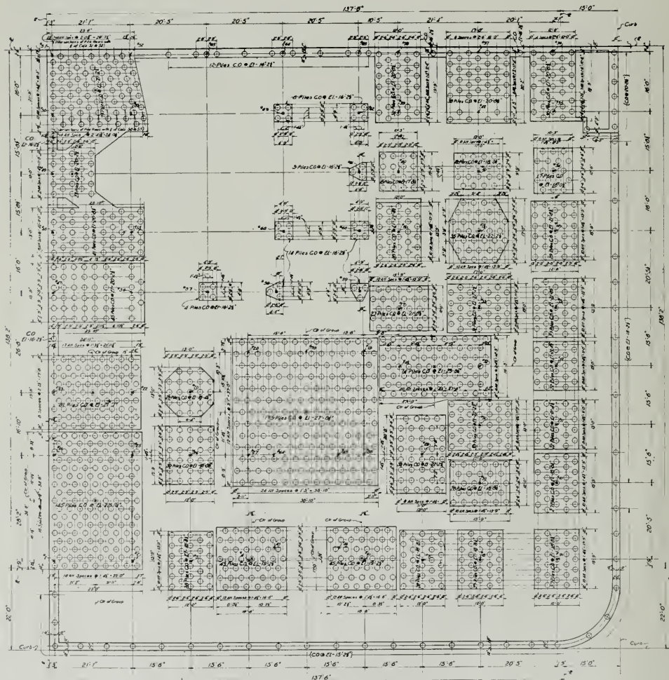
PLAN OF PILE FOUNDATIONS, P. G. & E. BUILDING C. H. Snyder, Engineer
