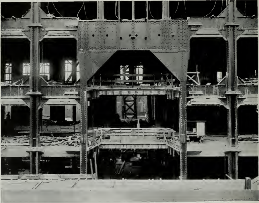
DETAIL OF STEEL GIRDER CONSTRUCTION OVER MAIN ENTRANCE T. Ronneberg and R. J. Fisher, Structural Engineers
