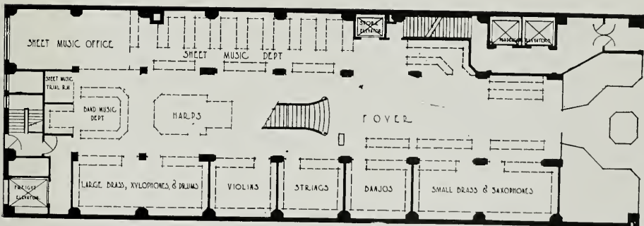
FIRST FLOOR PLAN, WURLITZER BUILDING, LOS ANGELES Walker and Eisen, Architects and Engineers
