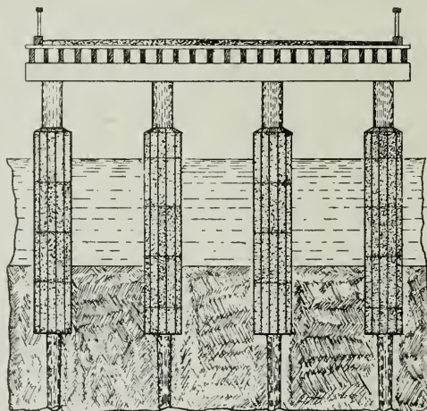
Bent of Wooden Piles Concreted by the Schlueter System.
