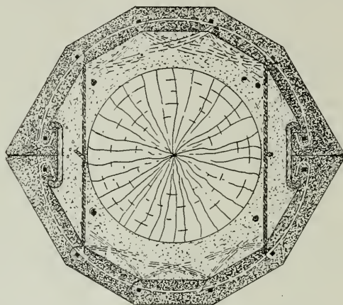
Cross Section of Wooden Pile Concreted by Schlueter System.
