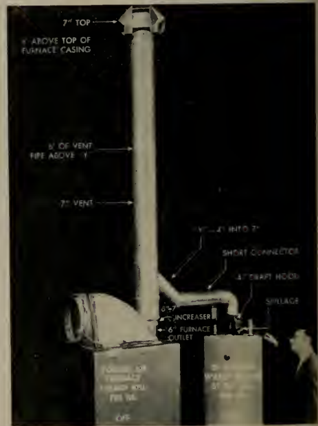
Fig. 3: Vent construction in accordance with building code.
