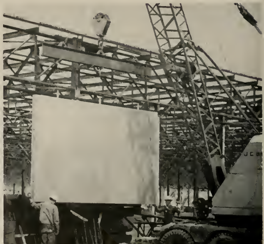
PANELS ARE LIFTED BY CRANE DIRECT FROM TRUCK FOR JOB SEQUENCE PLACE.
