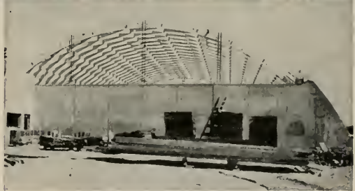
SUMMERBELL Lamella Roof Construction is easily adapted to fill-up wall construction, as illustrated above.
