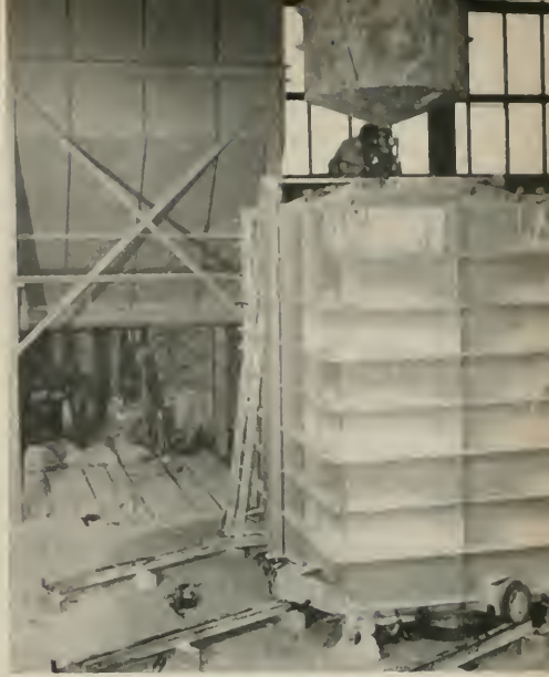
The bucket of mixed plaster is hoisted above aperture left by steel sections at the top of the mold, and material poured over domed concrete.
