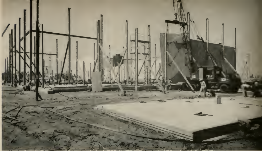
Precast concrete wall panels are poured on special "casting platforms" near their intended erection area—above illustration shows how site looked at the start of one four-day push.
