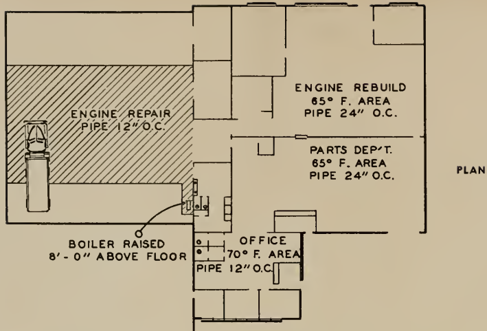
HEATING DESIGN FOR CUMMINS SERVICE AND SALES.
