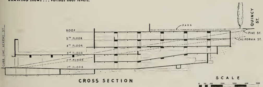
DRAWING shows . . . various floor levels.
