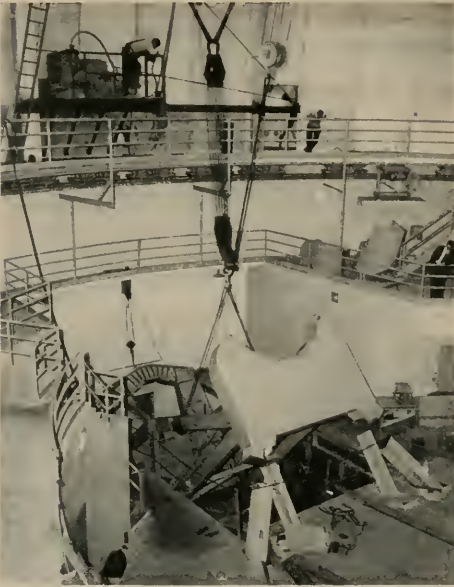
BASE FRAME being set in place inside Observatory. This base frame weldment had to be stress-relieved in its entirety by heating in a huge oven to a temperature of 1150 degrees fahrenheit.
