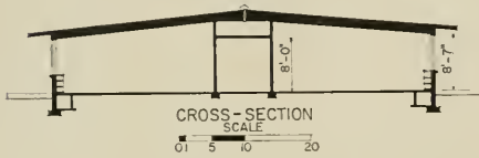
Detail of Cross Section of End Elevation.
