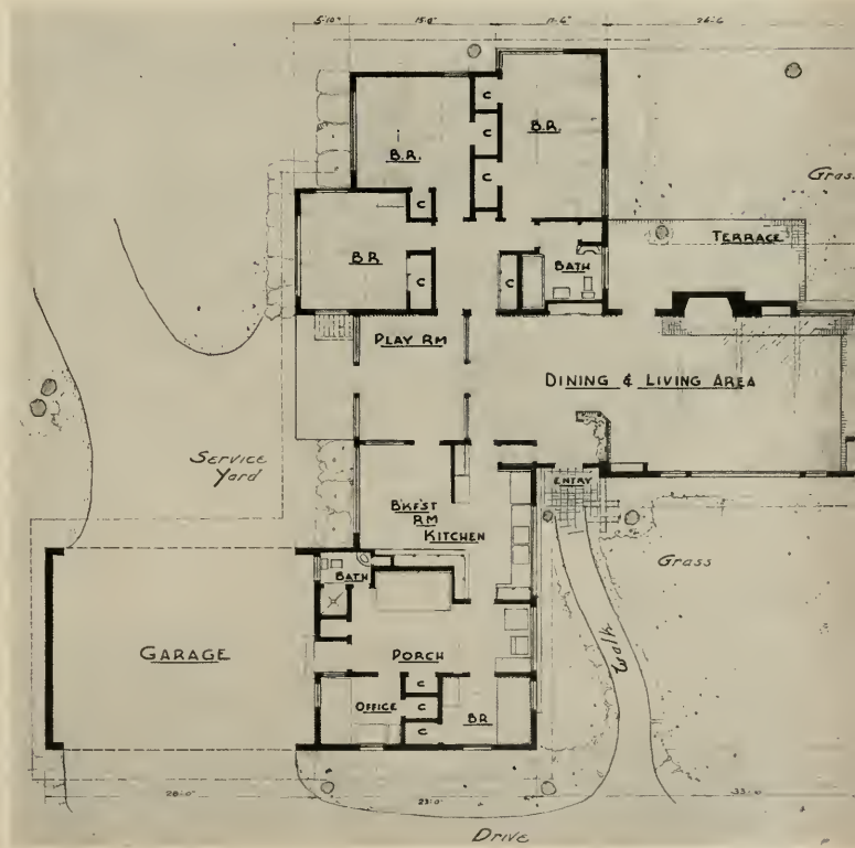
FLOOR PLAN and PLOT AREA
