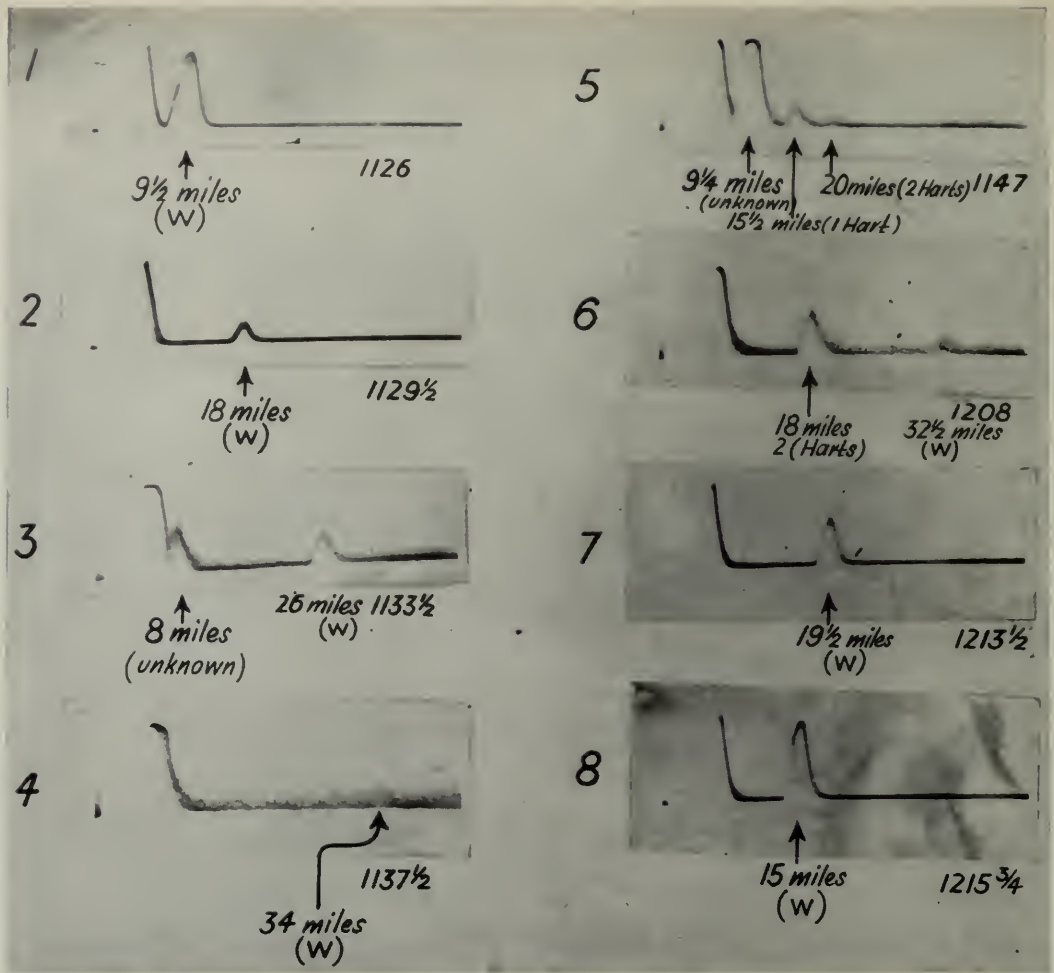
Copy of original British photographic radar record made on a cathode ray tube trace. The time of each photographic exposure is given on the right-hand side. The "echa" caused by a Wallace aircraft (W) on its outward journey is clearly visible (at increasing distances) in 1 to 4, and on its return journey (at decreasing distances) in 6 to 8. Nos. 5 and 6 indicate a formation of three Hawker Hart aircraft which came into the radar view uninvited.
