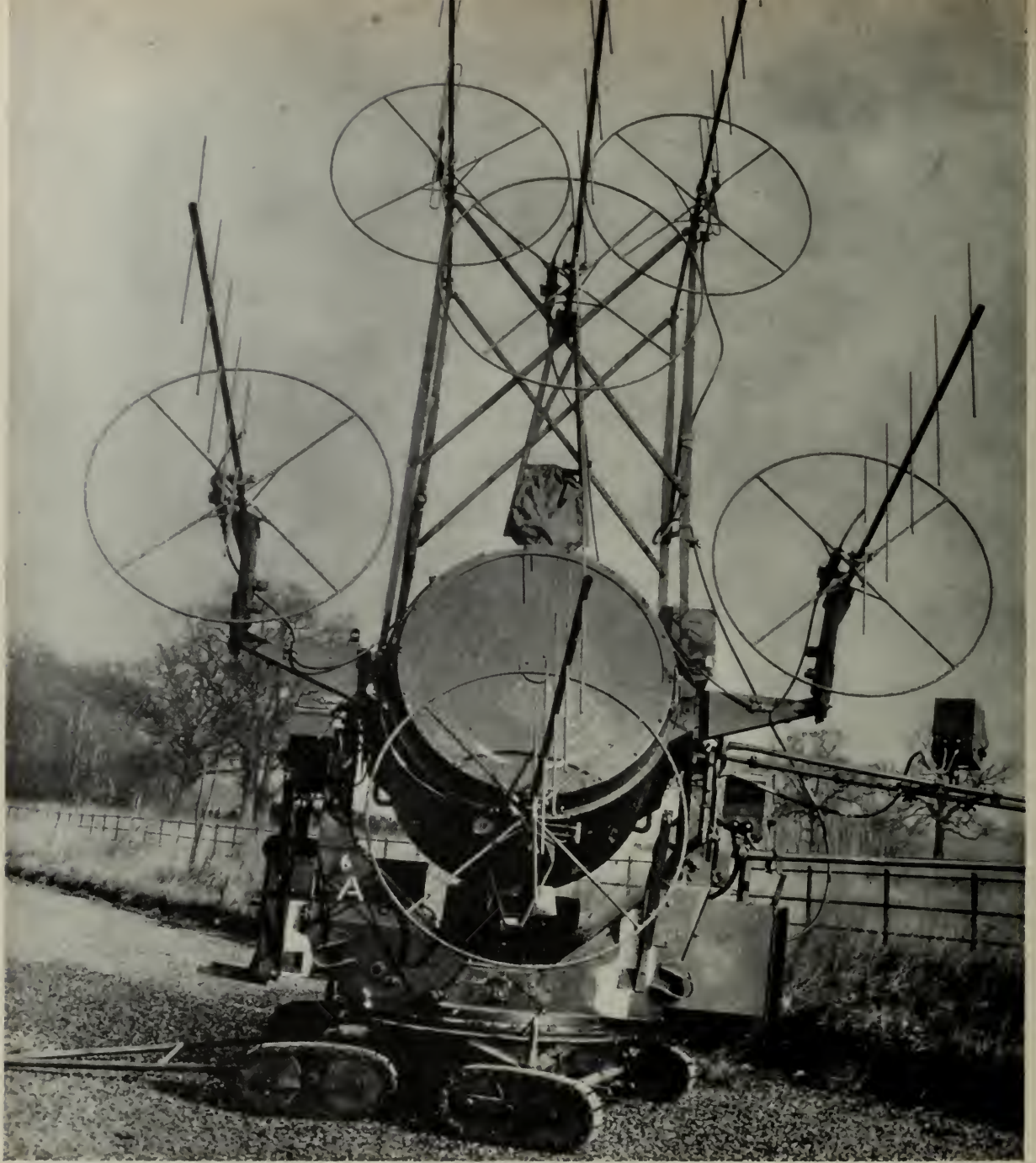
GIANT SEARCHLIGHT CONTROLLER very effective in England during the War.
