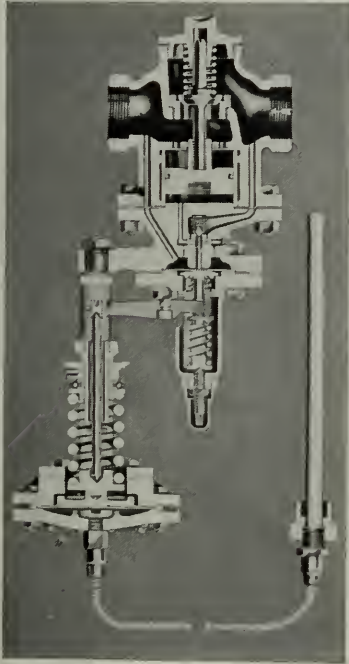
Self-contained Steam Regulator
