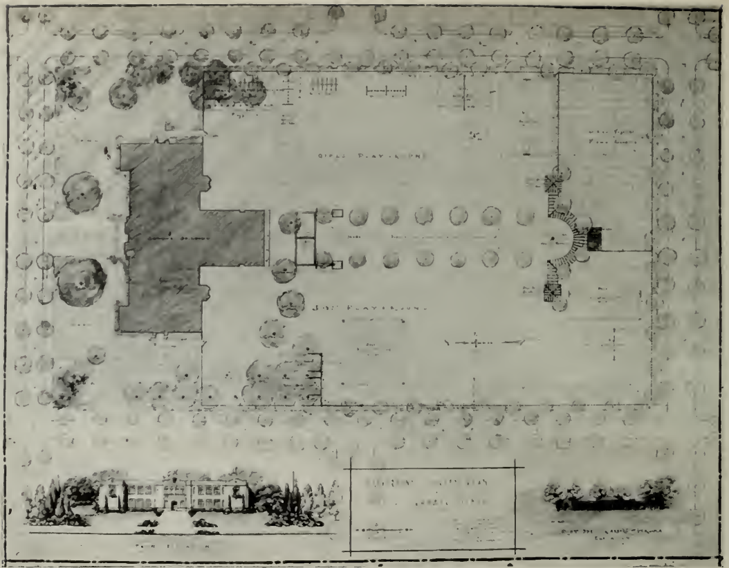
Playground and Garden Plan of Colusa, California Grammar School
