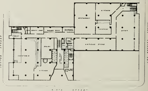
4' X 12' SCALE FIRST FLOOR PLAN TEXTILE DOLL DICK LOS ANGELES RISLEY & GOULD ARCHITECTS
