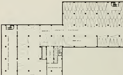
Sub-Basement Floor Plan
