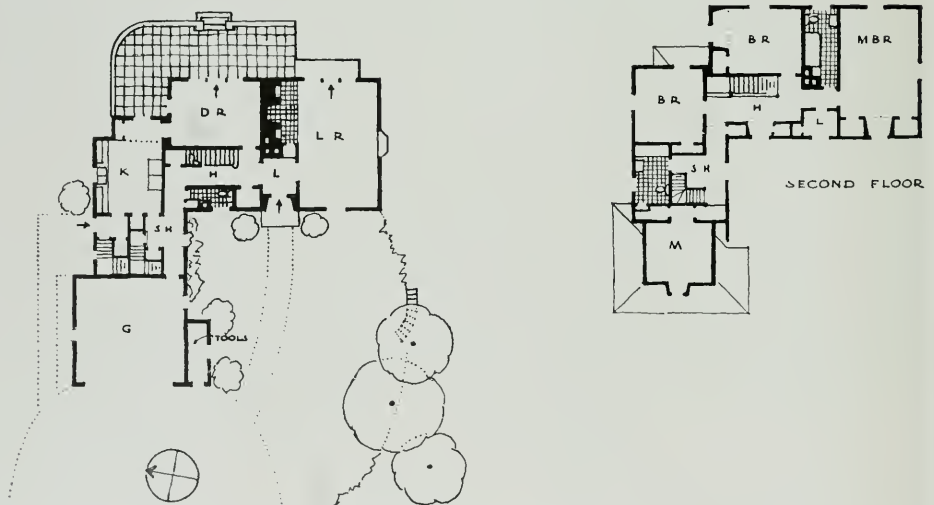
PLANS, RESIDENCE OF DR. MILTON STEINER, PORTLAND, OREGON
