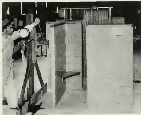
Snapshot of test for structure and seismic resistance of partitions for school shower and dressing compartments. Krafftile Terra Cotta Wall Units, reinforced by steel bars and concrete, resulted in a practical monolith.
