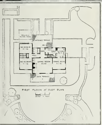
Left — Unique in its combination of compactness and flexibility (with provision for future addition of a room), this floor plan matches exterior charm and simplicity.
