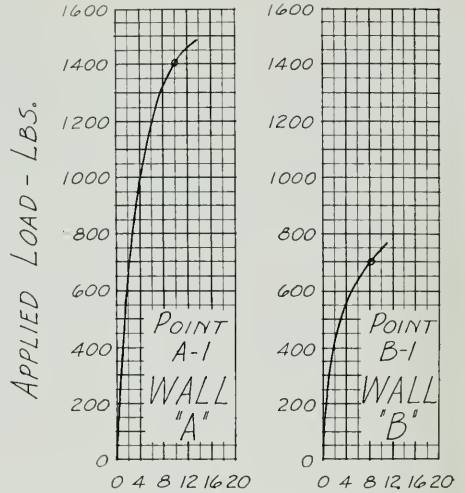
DEFLECTION by \frac{1}{64} inches Gauge readings on tests
