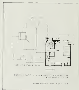
PLANS, HOUSE FOR CARL W. REBMANN, BELVEDERE Henry H. Gutterson Architect
