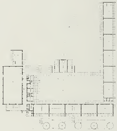
PLANS, FOWLER ELEMENTARY SCHOOL, FOWLER, CALIFORNIA Chas. H. Franklin and Ernest J. Kump, Jr., Architects
