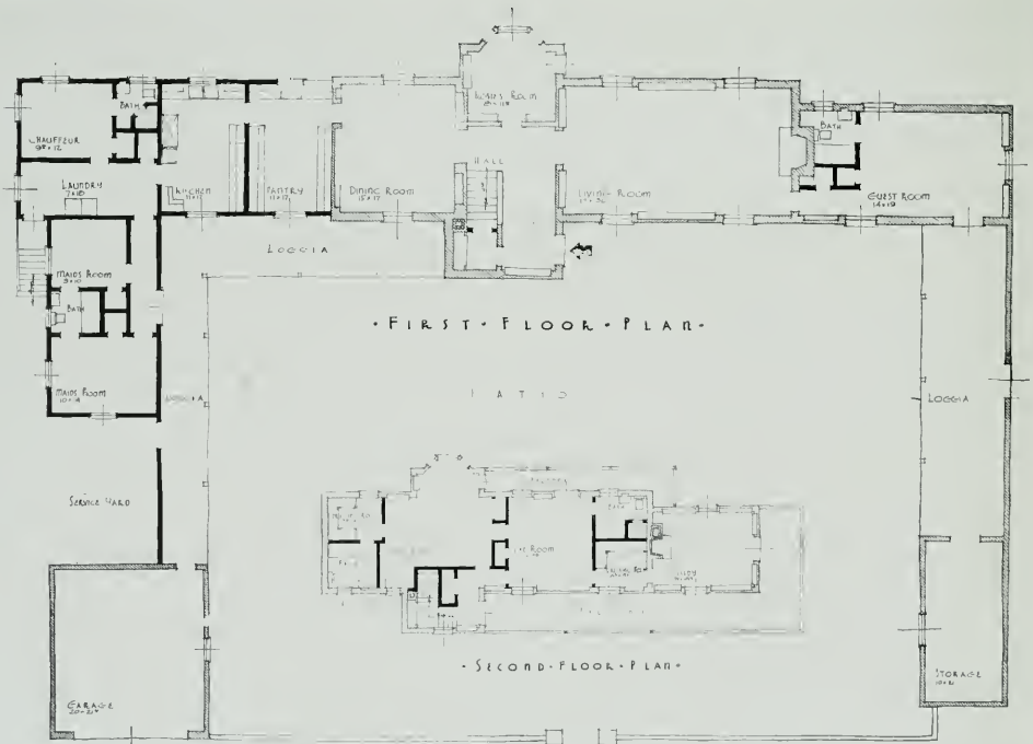
PLANS, HOUSE FOR EUGENE AND CARLOTTA MONTEREY O'NEILL, SAN RAMON VALLEY, CALIFORNIA Frederick L. Confer, Architect
