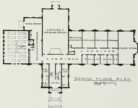
LIBRARY, PACIFIC LUTHERAN COLLEGE, PARKLAND, WASHINGTON E. J. Breseman and Heath, Gove & Bell, Associate Architects
