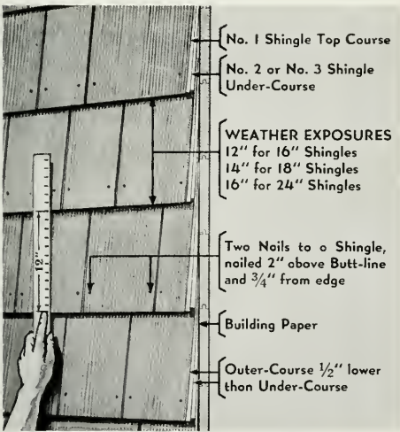
CONSTRUCTION DETAILS OF DOUBLE COURSING
