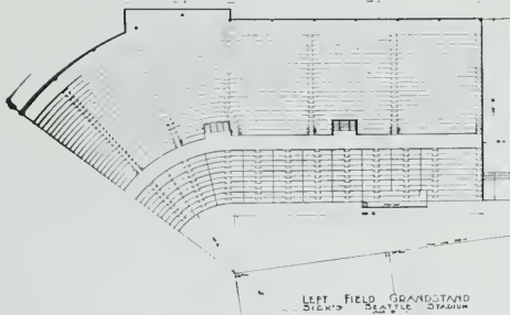
PLANS AND SECTION OF GRANDSTAND, SEATTLE BASEBALL PARK
