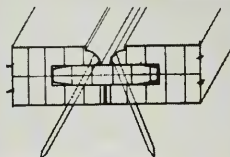
Nail heads are hidden in the depth and shadow of the joint, getting a good grip on the material and studs. Large spans require intermediate nailing.
