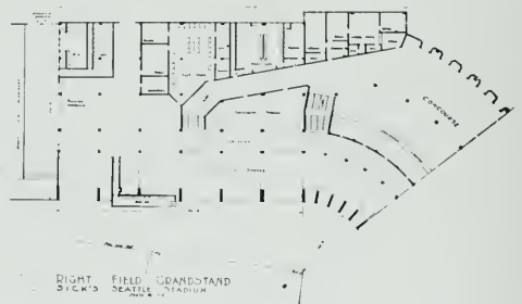
PLANS AND SECTION OF GRANDSTAND, SEATTLE BASEBALL PARK
