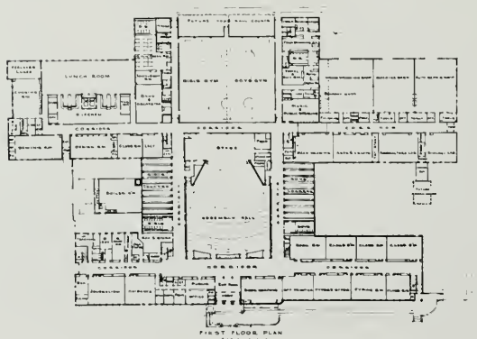
PLAN, HIGH SCHOOL, BELLINGHAM
