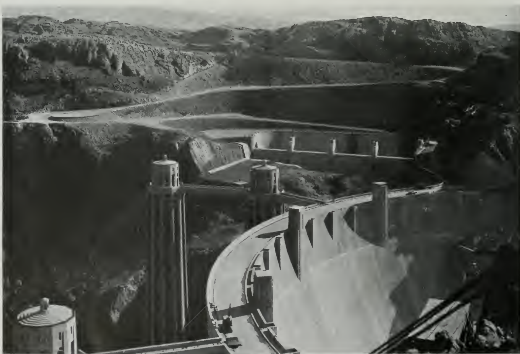
TOWERS AND PLATFORMS, BOULDER DAM
