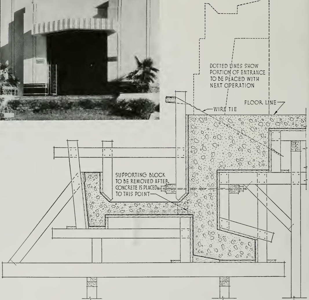
NARROW CANOPY WITH FASCIA BEAM
