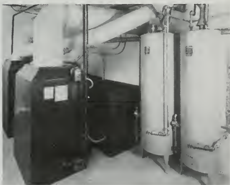
SHOWING FORCED AIR GAS FURNACE AND AUTOMATIC WATER HEATING IN- STALLATION IN BASEMENT
