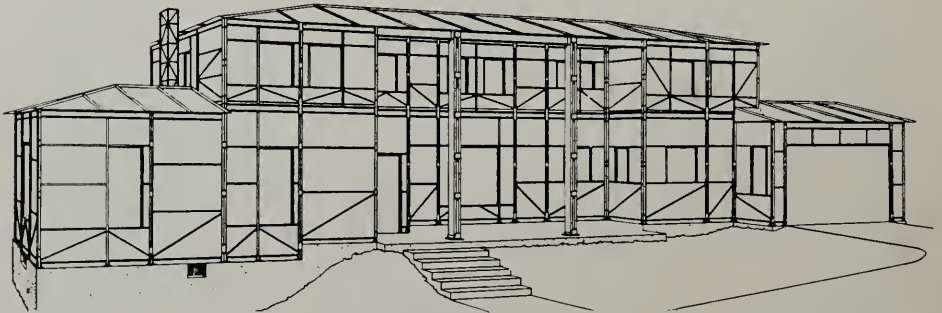
DESIGN OF STEEL FRAME, HOUSE FOR TUDOR GAIRDNER, HOLLYWOOD, CALIFORNIA
