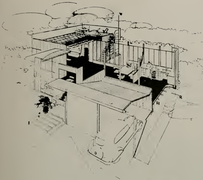
RESIDENCE OF PROF. WM. BEARD. ALTADENA, CALIFORNIA Richard J. Neutra, Architect Gregory Ain, Associate
