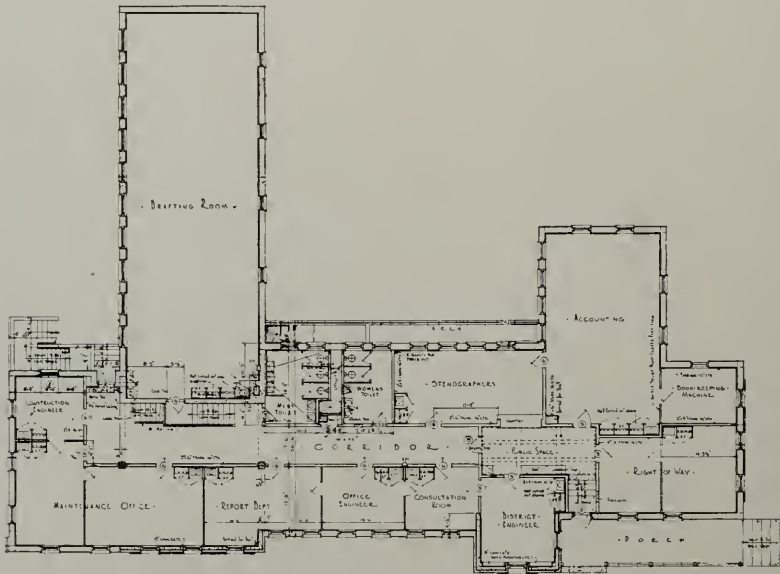
PLAN, DISTRICT HEADQUARTERS, CALIFORNIA STATE DEPARTMENT OF HIGHWAYS, MARYSVILLE
