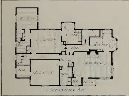
TYPICAL TWO-APARTMENT PLAN, BUILDING FOR J. E. PATTERSON Chester H. Treichel, Architect
