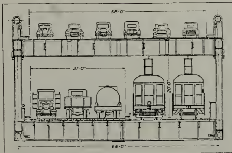
SECTION VIEW OF SAN FRANCISCO-OAKLAND BAY BRIDGE, SHOWING TRAFFIC LANES
