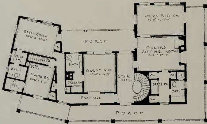
PLANS, RESIDENCE OF JAMES M. IRVINE, ALTADENA, CALIFORNIA H. ROY KELLEY, ARCHITECT
