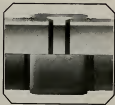
Section of National DUROLINE Pipe coupling and joint. (Note special highly corrosion-resistant joint compound on end of pipe and on threads.)
