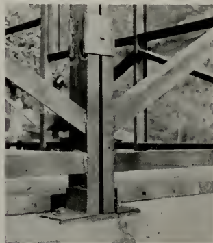
STEEL FRAME HOUSE—Steel anchor bolts are imbedded in concrete foundation to secure column members of the steel wall framing units.
