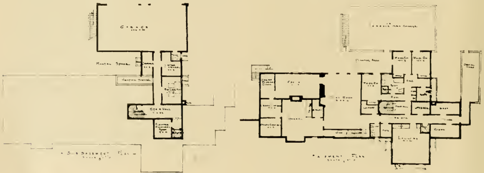
PLANS, RESIDENCE OF C. B. PIPER, PASADENA, CALIFORNIA Robert H. Ainsworth, Architect
