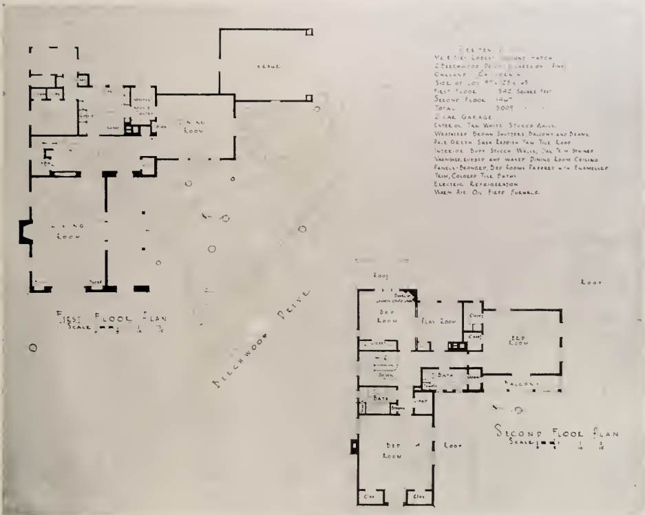
PLANS, RESIDENCE OF ROBERT E. HATCH, OAKLAND ARTHUR F. DUDMAN, ARCHITECT
