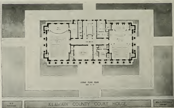
SECOND FLOOR PLAN, KLAMATH COUNTY COURT HOUSE Benj. G. McDougall, Architect
