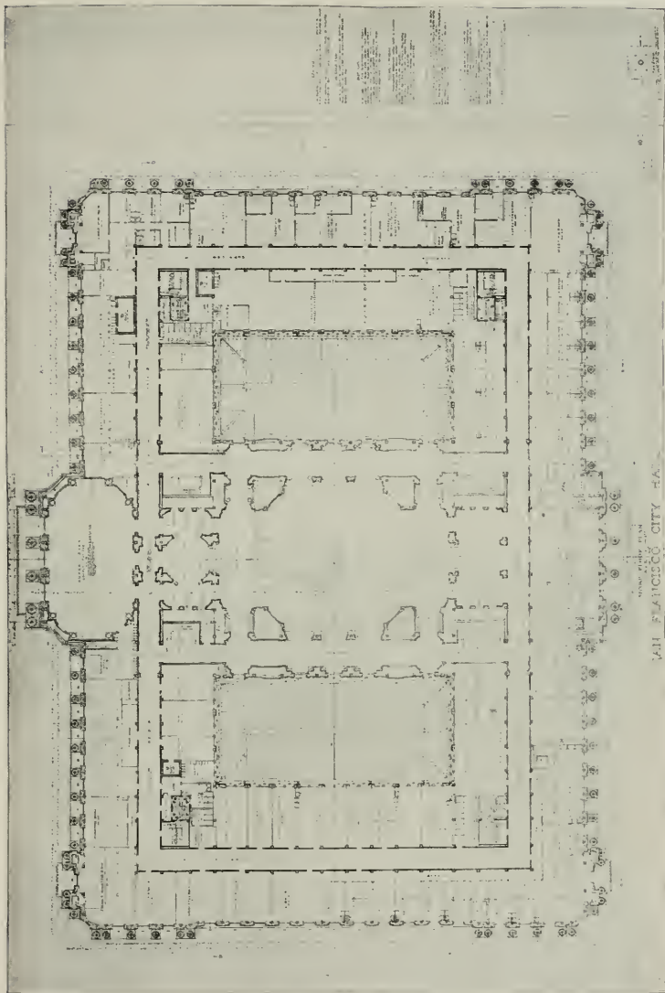
SAN FRANCISCO CITY HALL, SECOND FLOOR PLAN "TYPICAL" BAKERELL & BRODY, ARCHITECTS
