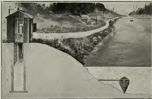
TYPICAL GAGING STATION WITH WELL AND REGISTER HOUSED
