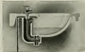
This is the Hajoca No. 10 Basin Waste, similar in construction and operation to the Hajoca No. 10 Bath Waste, and having the same unique and health-protecting advantages
