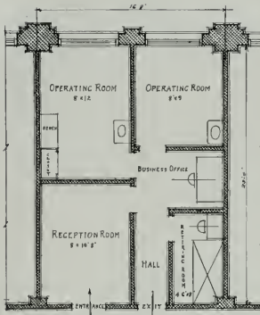
PLAN No. 1
