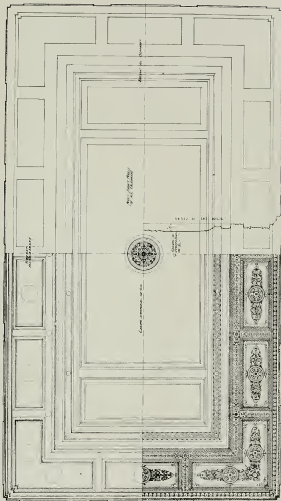
DETAIL OF CEILING, STOCKTON BANK, CHAS. W. DICKEY, ARCHITECT
