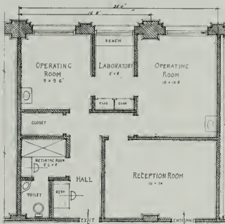
PLAN No. 3
