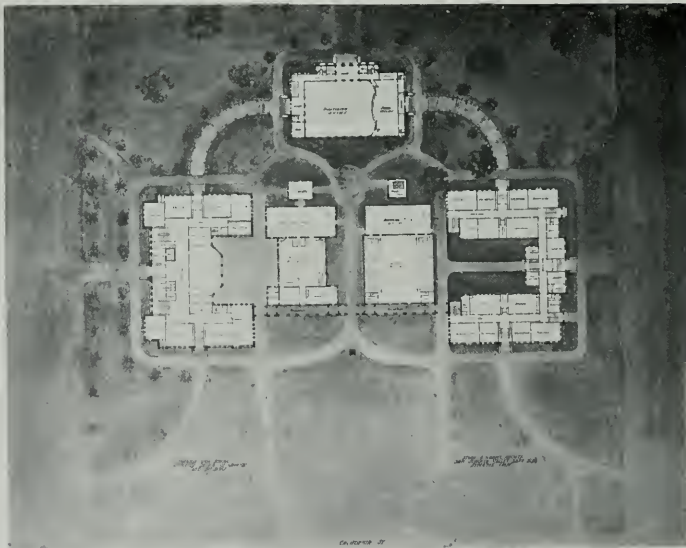
PLOT PLAN, HIGH SCHOOL GROUP, STOCKTON Stone & Wright, Architects
