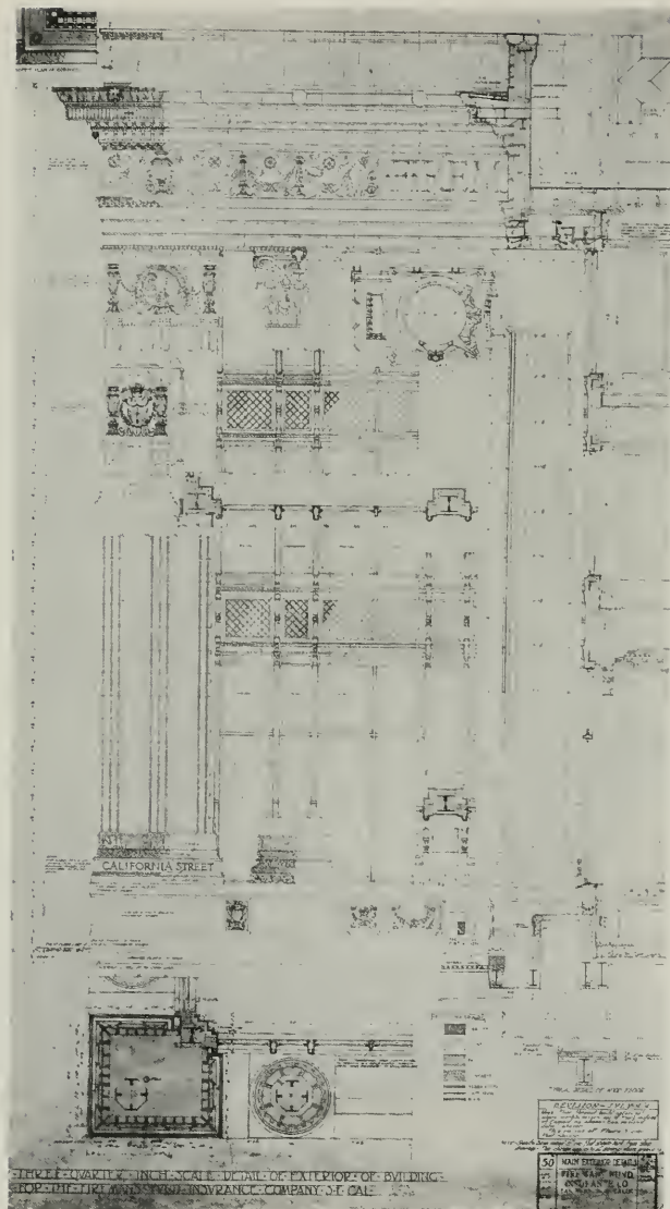
THREE-QUARTER INCH SCALE DETAIL OF EXTERIOR OF BUILDING. PROPERTY OF THE FIREMAN'S FUND INSURANCE COMPANY OF CALIF. ARCHITECT LEWIS P. HOBART.
