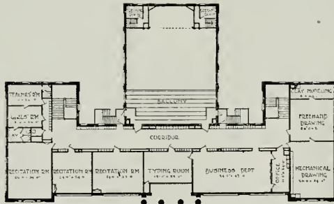
LODI HIGH SCHOOL—SECOND FLOOR PLAN STONE & WRIGHT, ARCHITECTS
