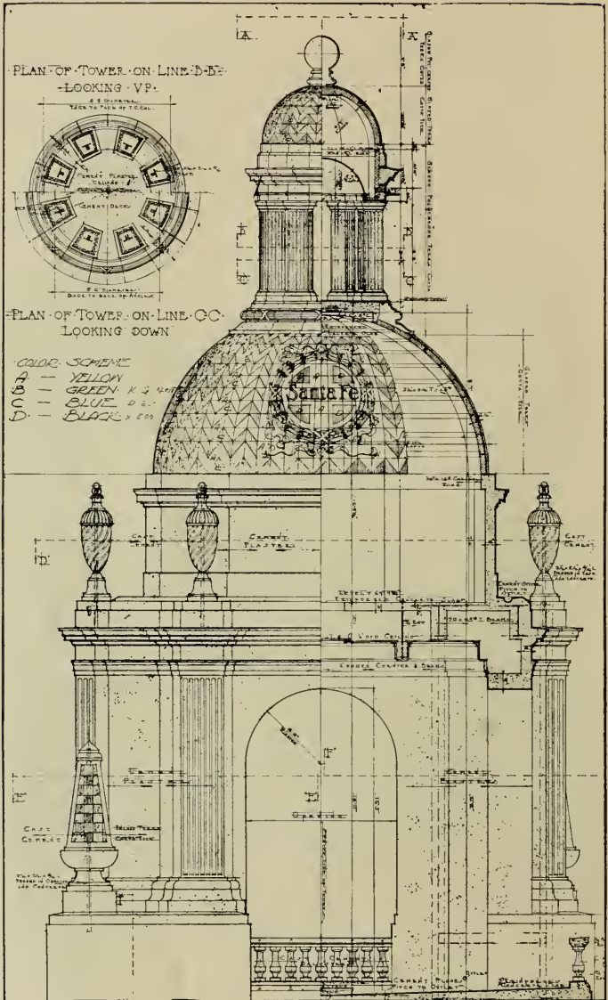
PLAN OF TOWER, SANTA FE STATION, SAN DIEGO
