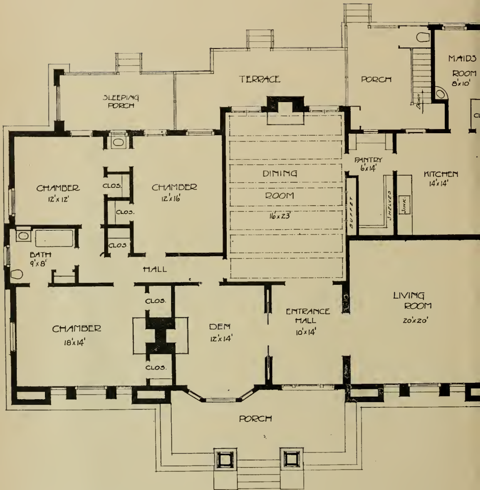
FLOOR PLAN, MISSION BUNGALOW TUCSON, ARIZONA
