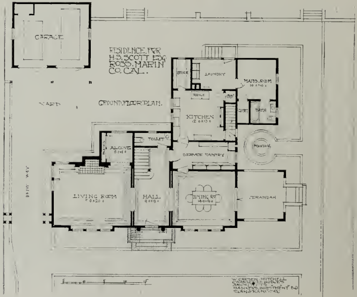
GROUND FLOOR PLAN, HOUSE FOR MR. H. S. SCOTT
