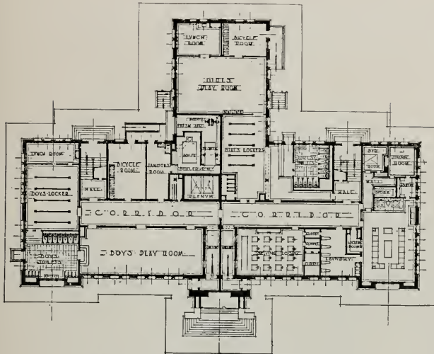
BASEMENT PLAN, WOODLAND HIGH SCHOOL
