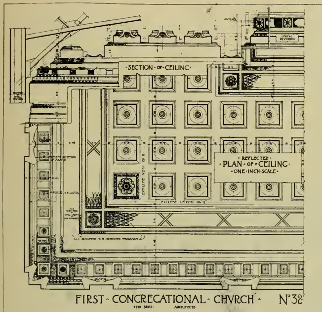
PLAN OF CEILING, FIRST CONGREGATIONAL CHURCH, SAN FRANCISCO Reid Bros., Architects
