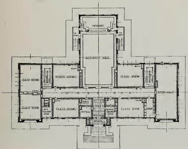
FIRST FLOOR PLAN, WOODLAND HIGH SCHOOL
