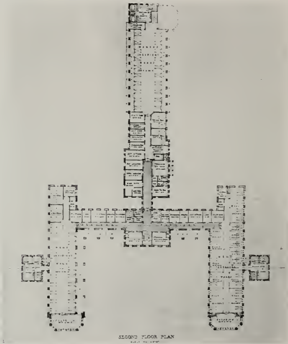
SECOND FLOOR PLAN, ADDITION TO SAN FRANCISCO CITY HOSPITAL Herman Barth, Architect
