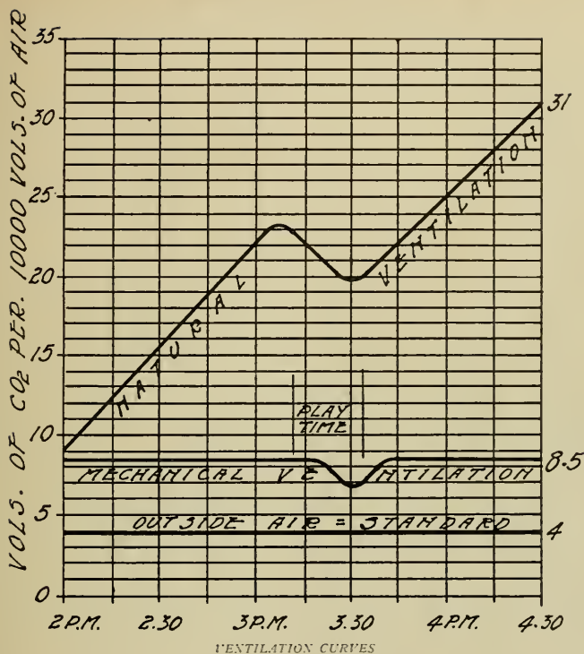
VENTILATION CURVES
