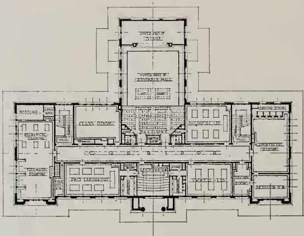
SECOND FLOOR PLAN, WOODLAND HIGH SCHOOL
