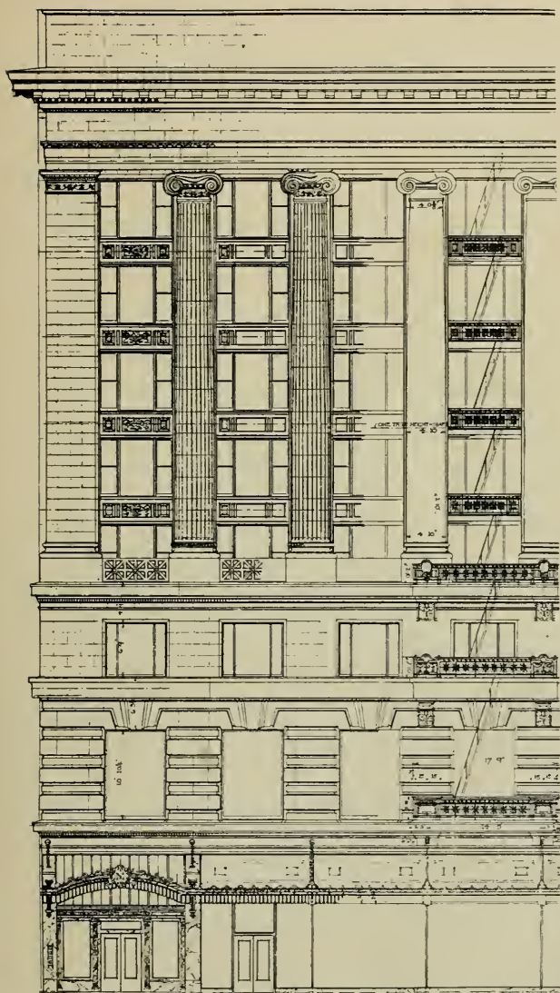
ELEVATION, MERRITT BUILDING, LOS ANGELES REID BROS., ARCHITECTS
