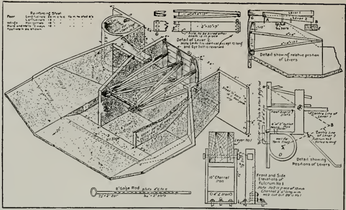
Fig. 1. Automatic Check Drop on Lateral of Turlock Irrigation District
