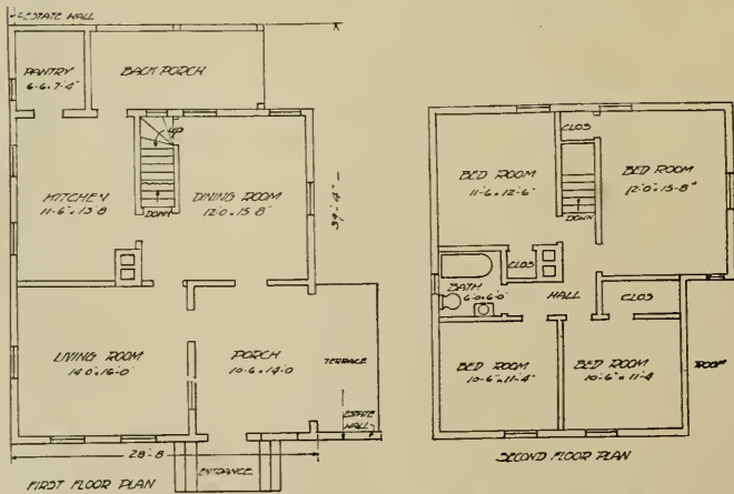
PLANS OF $2,700 COTTAGE WITH 8-IN. WALLS, NEAR MIDDLEBURG, VA.
