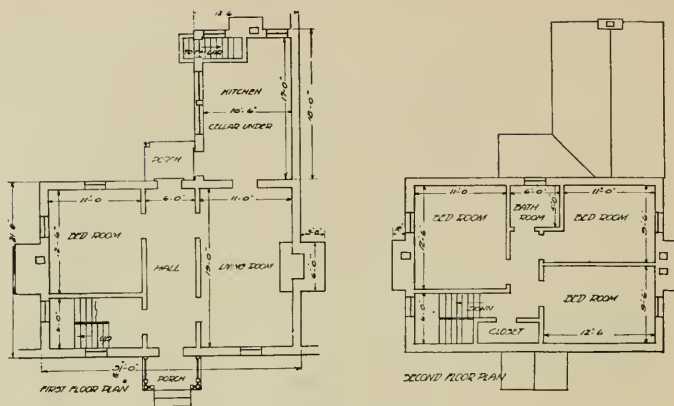
PLANS OF CONCRETE COTTAGE NEAR MIDDLEBURG, V.A.
