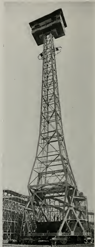
AEROSCOPE RAISED TO FULL HEIGHT
