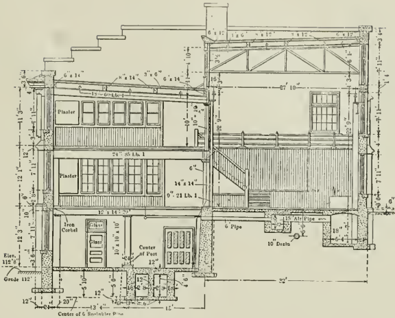
Fig. 4.—Cross-Section Through Machine Shop
