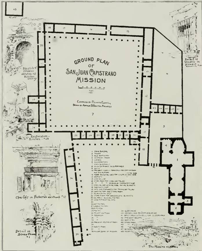
Ground Floor Plan, Restoration of Capistrano Mission Arthur B. Benton, Architect
