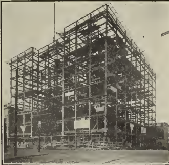
Steel Frame of Y. M. C. A. Building, San Francisco McDougall Bros. Architects
