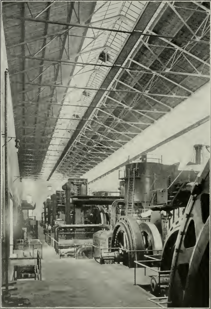
Interior Station 1, San Francisco Gas and Electric Company, Showing Roof Construction.
