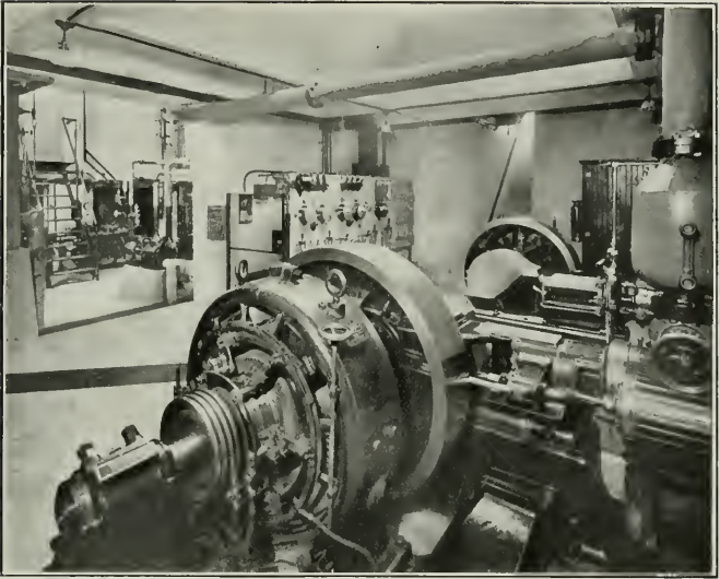
Power Plant, Pacific Union Club Building. This and Other Mechanical Features were Designed and Installed Under the Supervision of Mr. Geo. E. Atkins, Mechanical Engineer of the Firm of Willis Polk & Company
