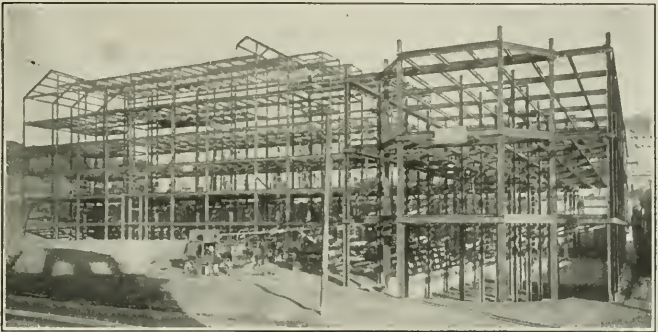
STEEL FRAME, ST. MARY'S HOSPITAL. WILLIS POLK & CO., Architects
