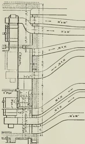
Fig. 2.—Plan of Heaters in Main Shop
