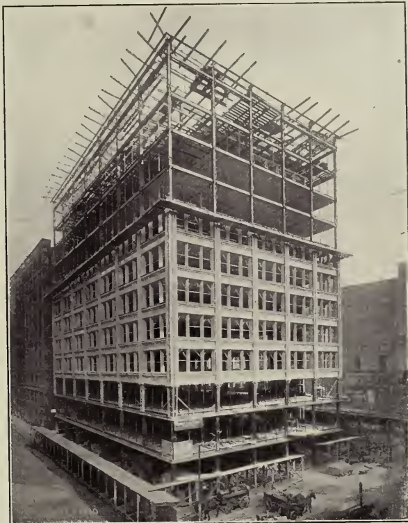
Safety Platforms at Top of Eighth Floor
