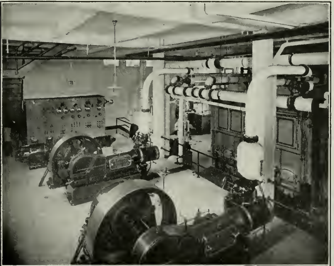
Mechanical Plant, St. Mory's Hospital, San Francisco, California
