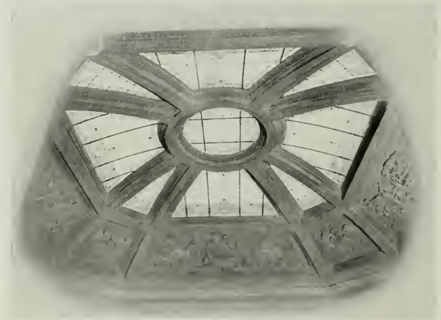
Central Court Dome Under Construction and Completed, Pacific Union Club Building. Designed by Mr. T. Ronneberg, Structural Engineer of the Firm of Willis Polk & Company
