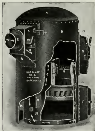
THE QUAKER FURNACE GILLEY-SCHMID CO., Agents
