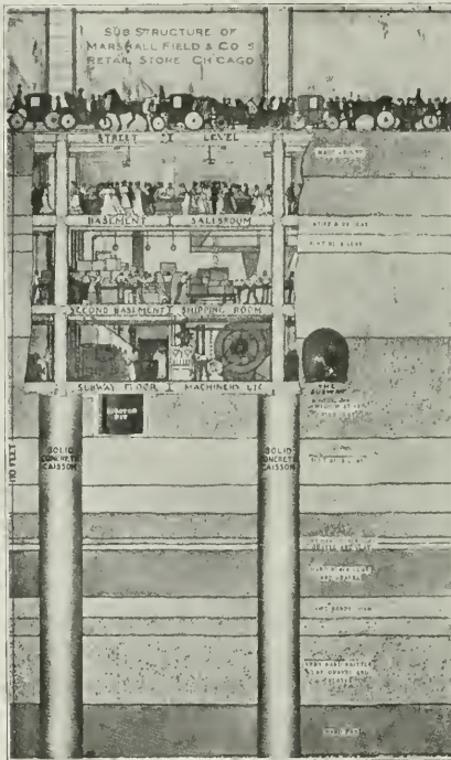
Sectional View Showing Foundation and Sub-Basements, Marshall Field & Co., Chicago (Courtesy of Rock Products)
