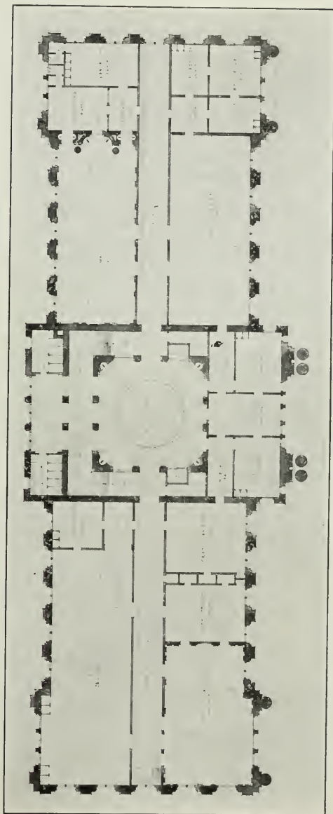
Third Floor Plan, Kern County Court House, Bakersfield, Cal. Frederick H. Meyer, Architect
