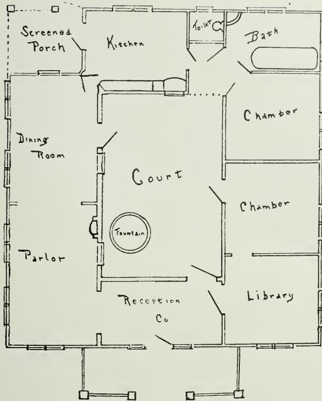
Floor Plan of Concrete House, Lodi, Cal.
