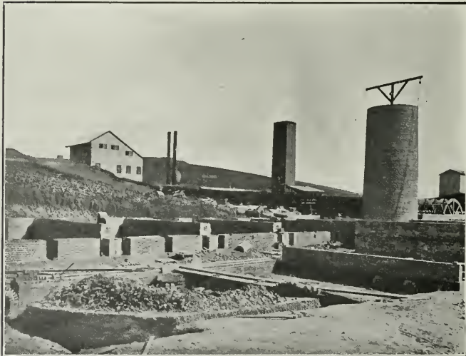
Foundation for a Sixteen Chamber Kiln
