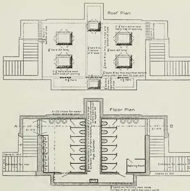
Plan of a Public Sanitary, Brookline, Mass. Alexis H. French, Engineer
