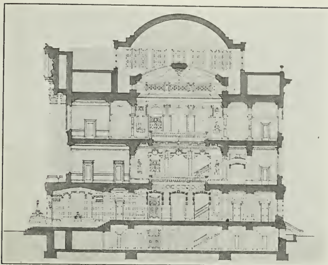
Sectional Elevation, Kern County Court House, Bakersfield, Cal. Frederick H. Meyer, Architect
