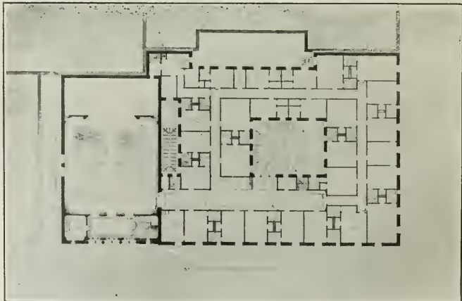
Second Floor Plan, Competitive Design for Bohemian Club Building Crim & Scott, Architects
