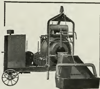
No. 0 Foote Batch Mixer with Power Loading Skip, Automatic Water Tank and Gasoline Engine.
