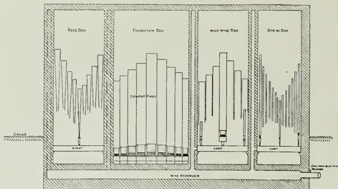
Sectional Elevation of Reinforced Concrete Organ at Ocean Grove Auditorium
