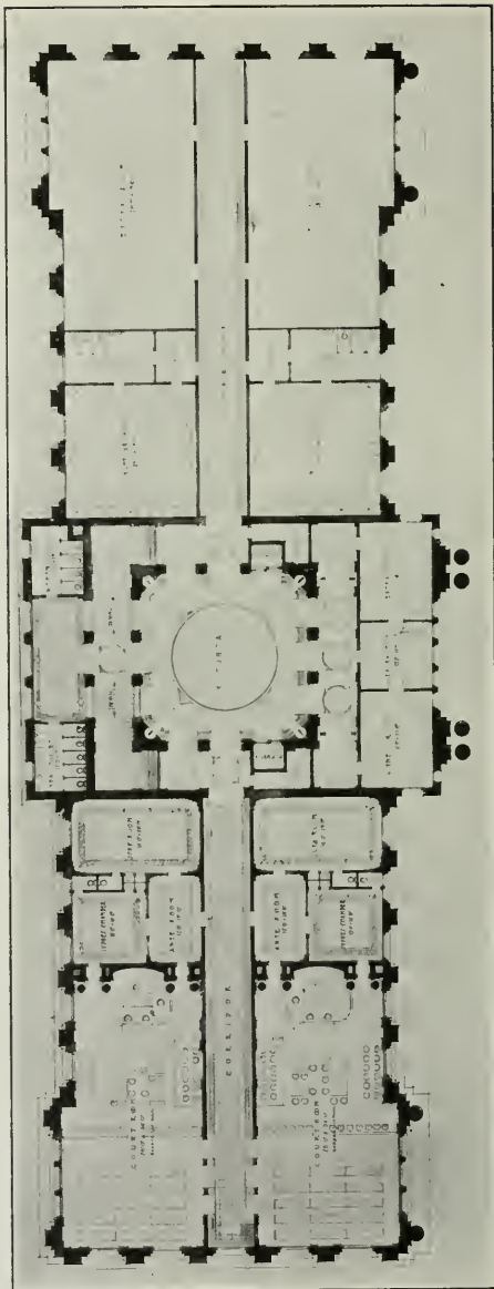
Second Floor Plan, Kern County Court House, Bakersfield, Cal. Frederick H. Meyer, Architect
