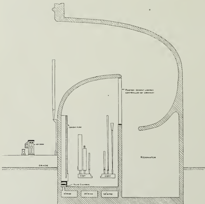
Sectional End Elevation of Reinforced Concrete Organ at Ocean Grove Auditorium.
