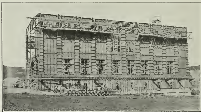
Showing Concrete Forms in Place, Transforming Station at Visitation, Cal.
