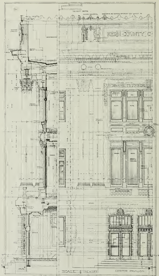
Detail of Center Pavilion, Kern County Court House, Bakersfield, Cal. Frederick H. Meyer, Architect
