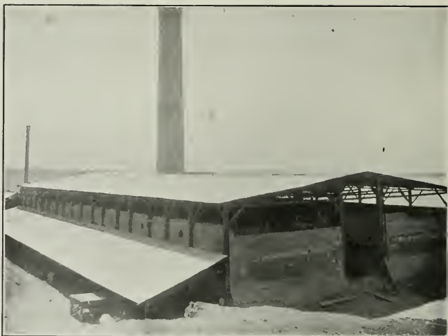
Sixteen Chamber Kiln in Operation
