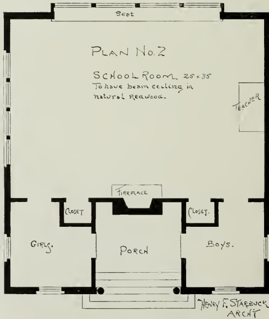
Perspective and Floor Plan for Country School House Henry F. Starbuck, Architect
