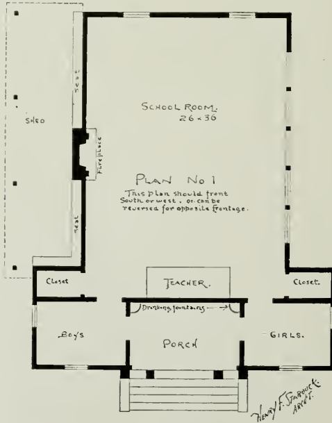
Perspective and Floor Plans for Country School House Henry F. Starbuck, Architect
