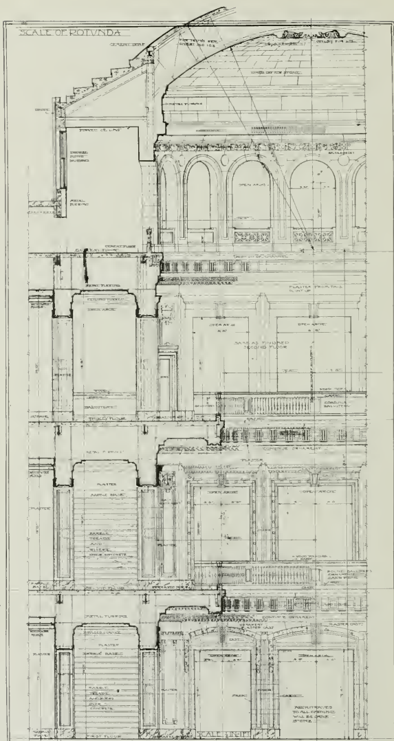
Detail of Rotunda and Dome, Kern County Court House, Bakersfield, Cal. Frederick H. Meyer, Architect
