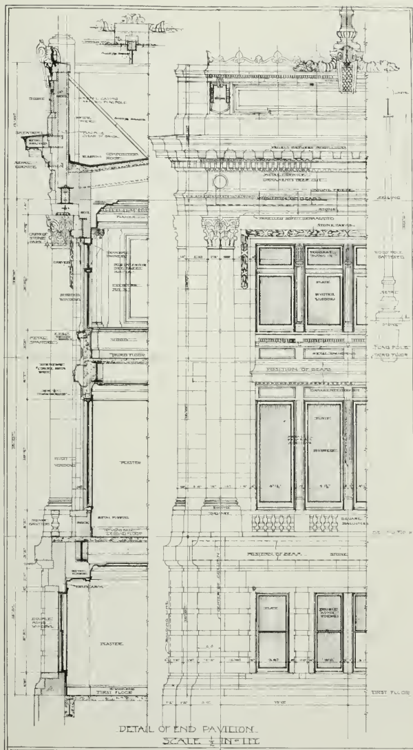
Detail of End Pavilion, Kern County Court House, Bakersfield, Cal. Frederick H. Meyer, Architect
