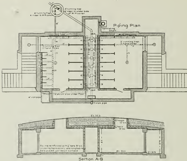
Plan of a Public Sanitary, Brookline, Mass. Alexis H. French, Engineer
