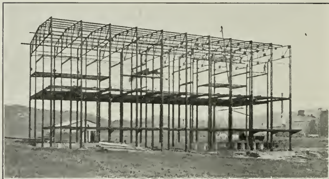
Steel Frame, Transforming Station, Visitation, Cal.
