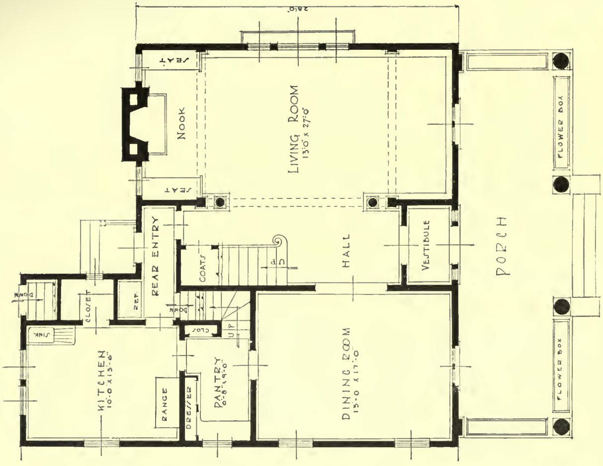
HOUSE OF JAMES WARBURTON, JR., EASTSIDE TERRACE. PATERSON, N. J. CHARLES H. BENJAMIN, ARCHITECT
