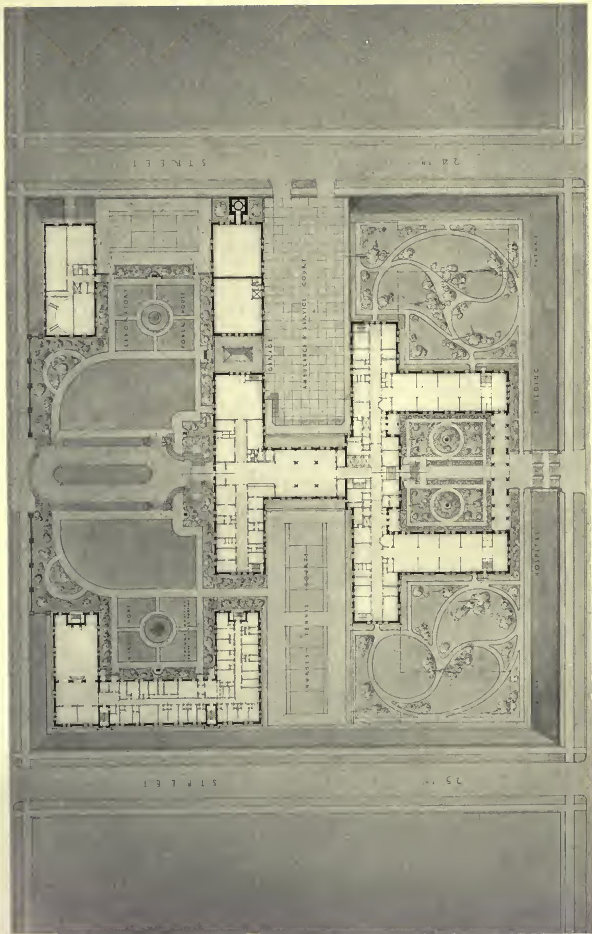
PLOT PLAN
