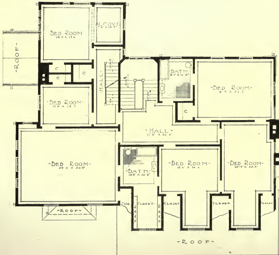
HOUSE OF GEORGE S. JOHNS, ST. LOUIS COUNTY, MO. T. P. BARNETT CO., ARCHITECTS
