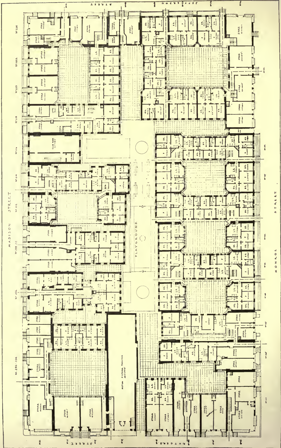
GROUND FLOOR PLAN SIBLEY & FETHERSTON, ARCHITECTS AWARDED FIRST PRIZE OF $1,000
