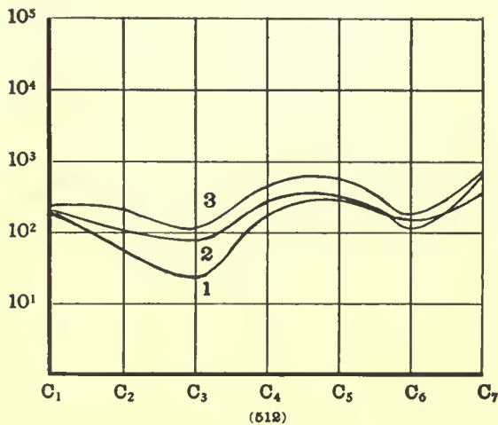
FIG. 3. Curve 1. Reduction produced by triplex glass. Curve 2. By 3/16" plate. Curve 3. By 1/4" plate.
