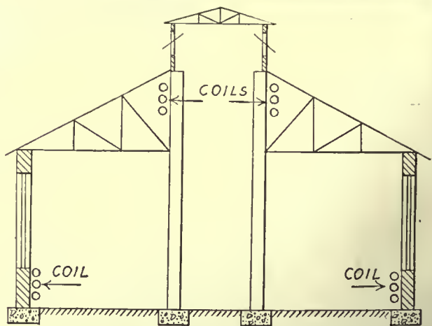
FIG. 2. ARRANGEMENT OF HEATING COILS FOR MONITOR ROOF CONSTRUCTION
