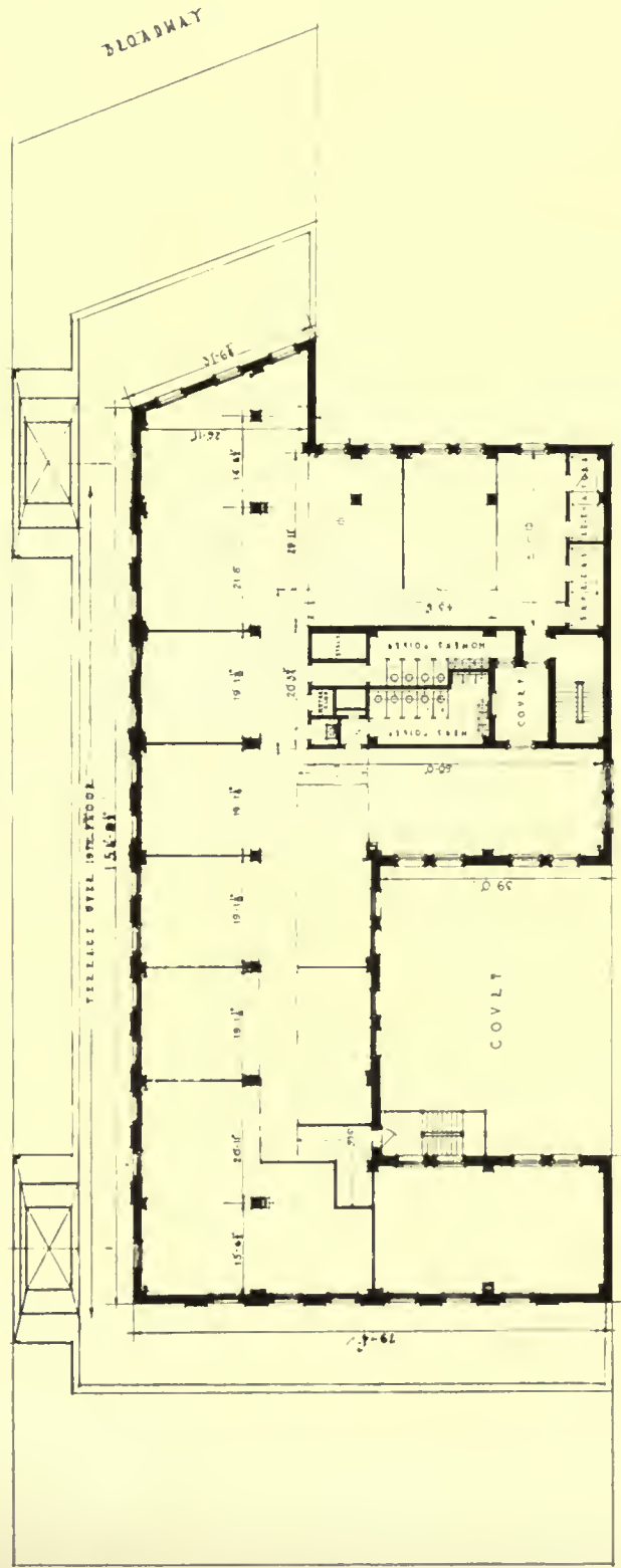
PLAN OF 20th TO 24th FLOORS.
