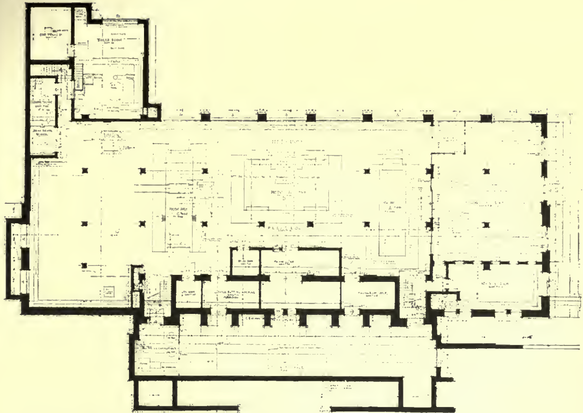
BASEMENT PLAN.
