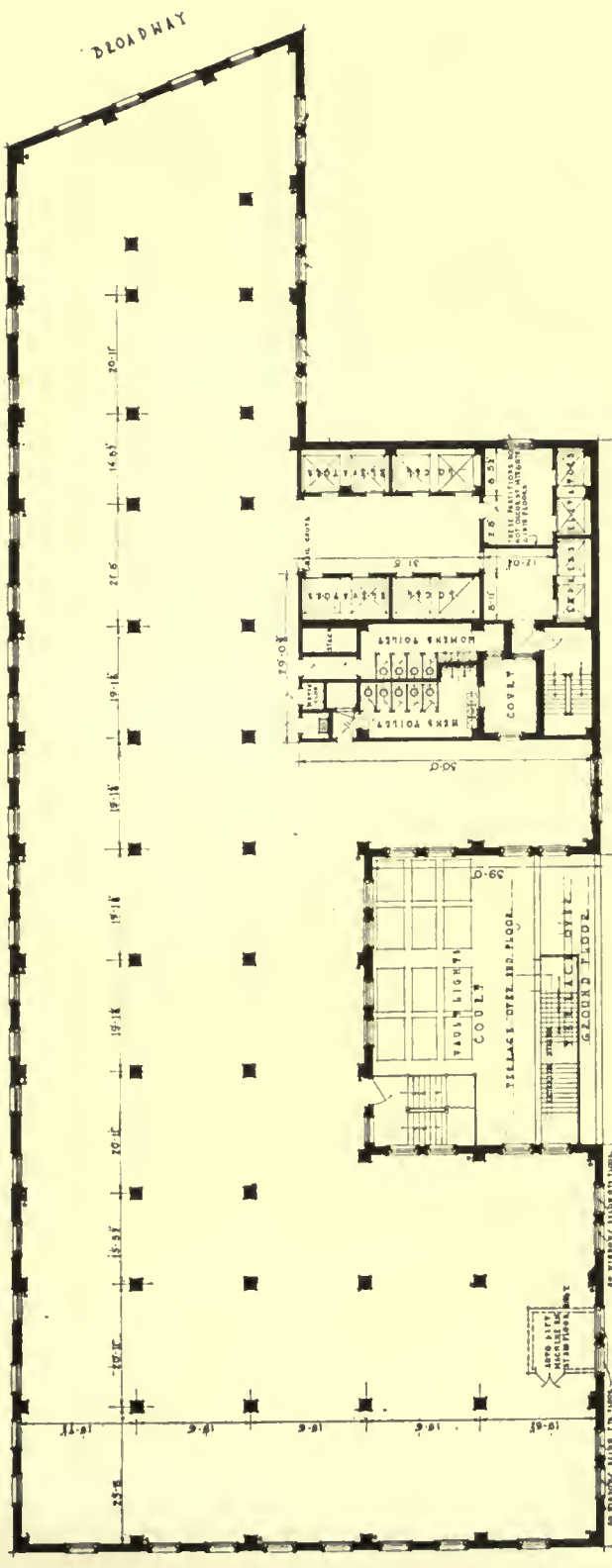
TYPICAL FLOOR PLAN
