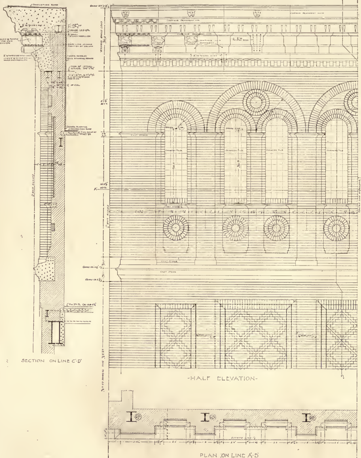
3/4 INCH SCALE DETAIL OF UPPER PART FRONT ELEVATION CHAUNCY STREET [21 ST ] STATION BOSTON FOR THE EDISON ELECTRIC ILLUMINATING COMPANY
