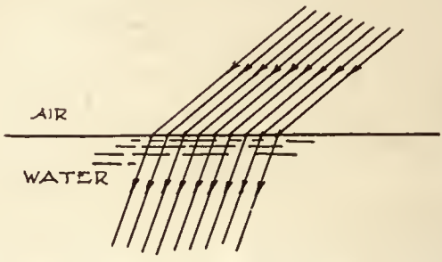
FIG. 5. REFRACTION. RAYS PASSING FROM ONE MEDIA TO ANOTHER OF DIFFERENT DENSITY ARE BENT
