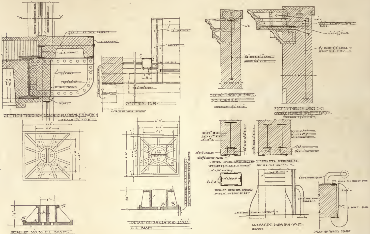
CONSTRUCTION DETAILS
