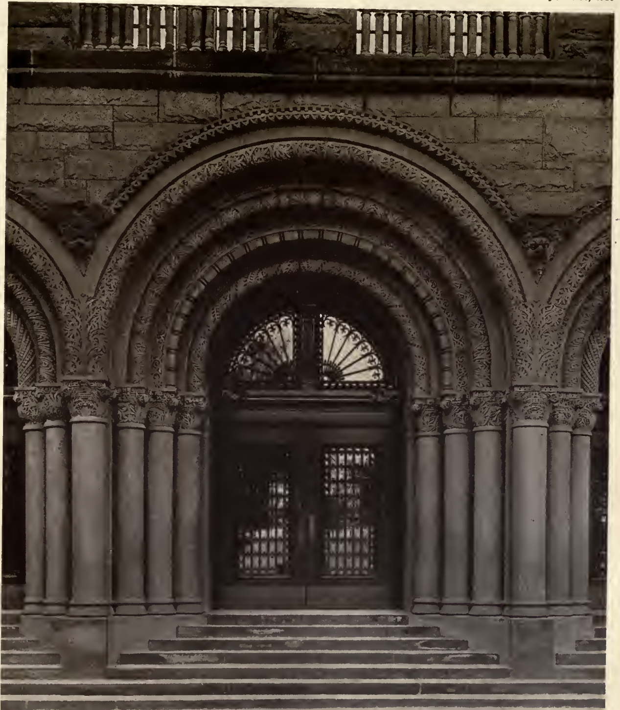
MAIN ENTRANCE DOORWAY, SHOWING ADDITION OF NEW GRILLES CITY HALL AT ALBANY, NEW YORK H. H. RICHARDSON, ARCHITECT OGDEN & GANDER, ASSOCIATE ARCHITECTS FOR THE ALTERATIONS
