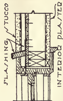
SECTION THRU WINDOW HEAD
