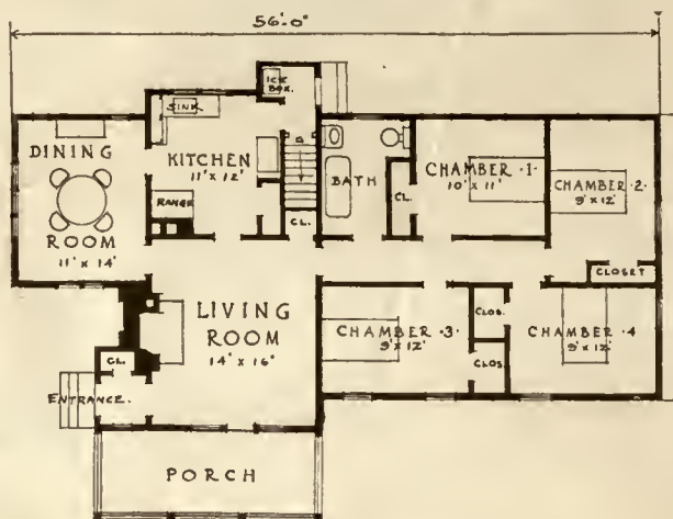
FOUR TEACHER COTTAGE
