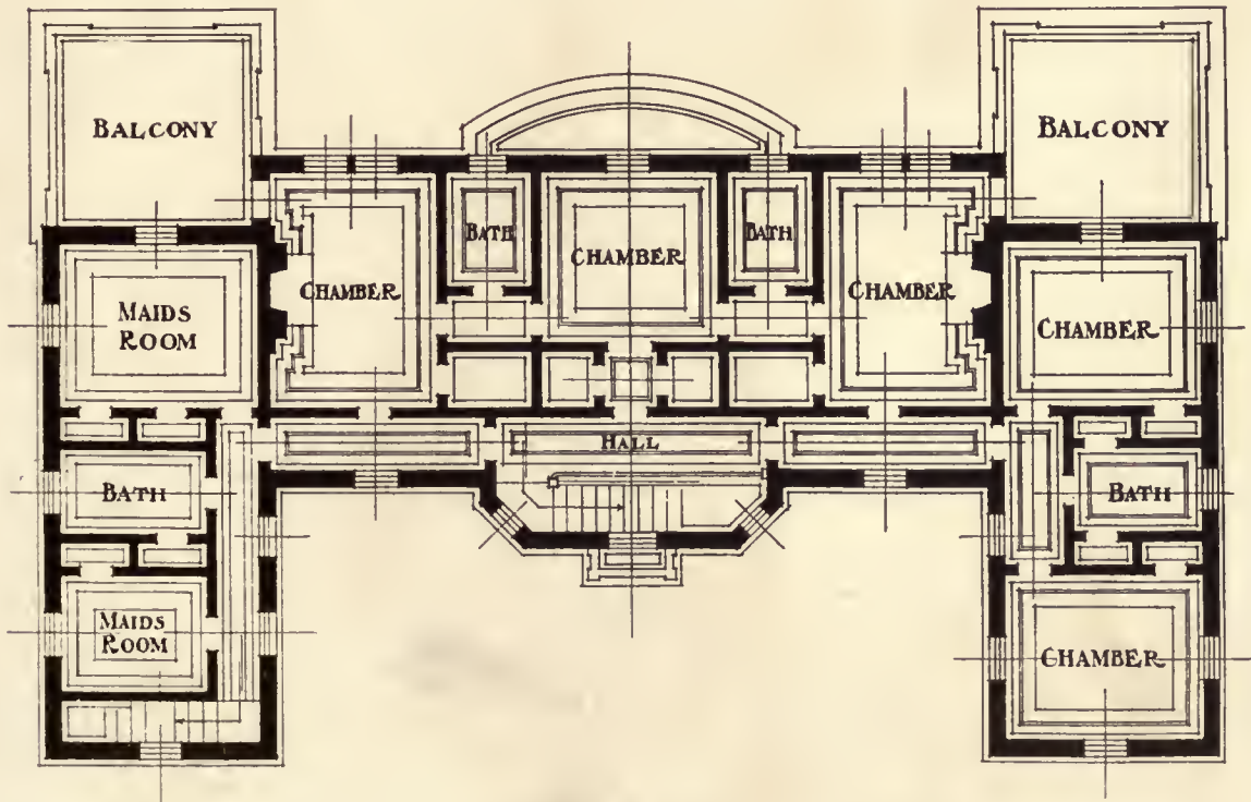
HOUSE OF GEORGE CROMPTON, POCASSET, MASS. JAMES PURDON, ARCHITECT
