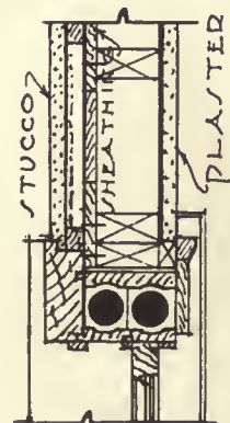
SECTION THRU WEIGHT BOX
