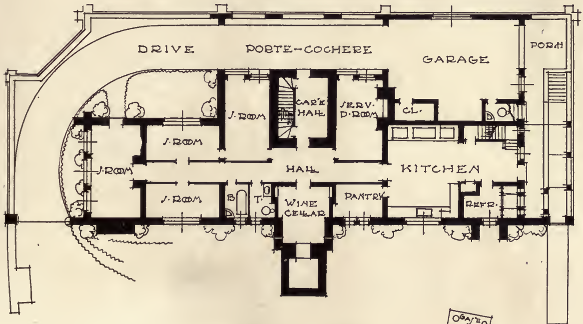
BASEMENT PLAN
