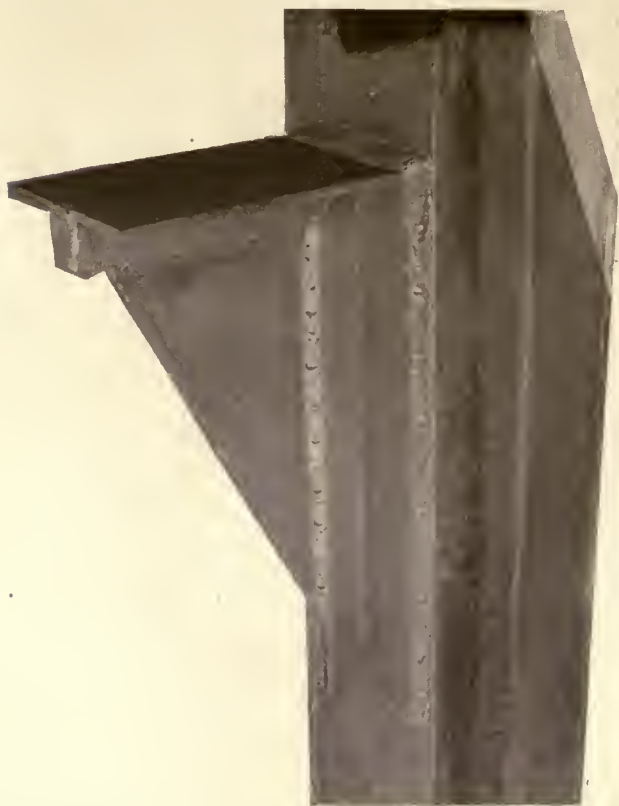
BRACKET SUPPORT FOR 5-TON CRANE RAIL, JOINED TO COLUMN BY ELECTRIC ARC WELDING
