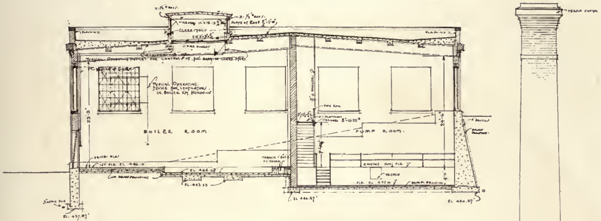
SECTION THRU BOILER & PUMP RMS. <
