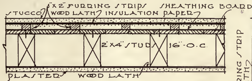
HORIZONTAL WALL SECTION
