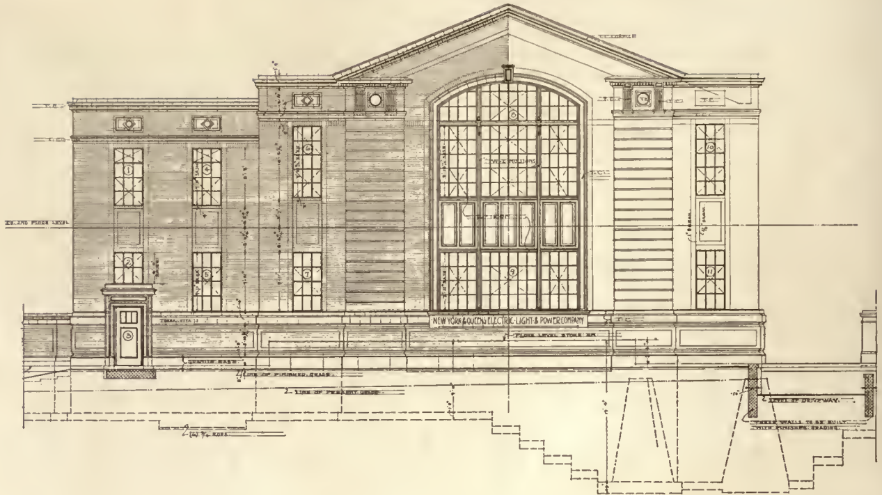
FRONT OR WESTERLY ELEVATION
