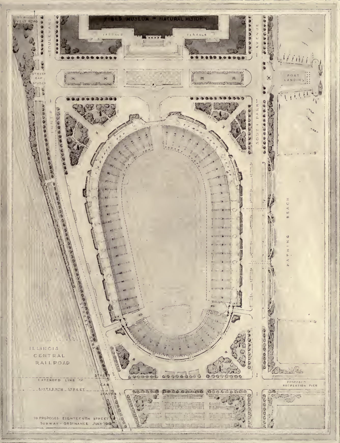
PLOT PLAN COMPETITION FOR A STADIUM ON THE LAKE FRONT, CHICAGO DESIGN SUBMITTED BY EDWARD D. BURNHAM AND WILLIAM W. PARSONS ARCHITECTS
