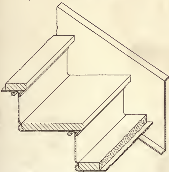
FIG. 7.—STEEL STAIRS WITH STONE TREAD
