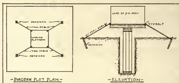
DIAGRAM SHOWING METHOD OF BRACING SOIL TESTING PLATFORM WITH STEEL CABLES OR WIRE GUYS TO PREVENT TILTING
