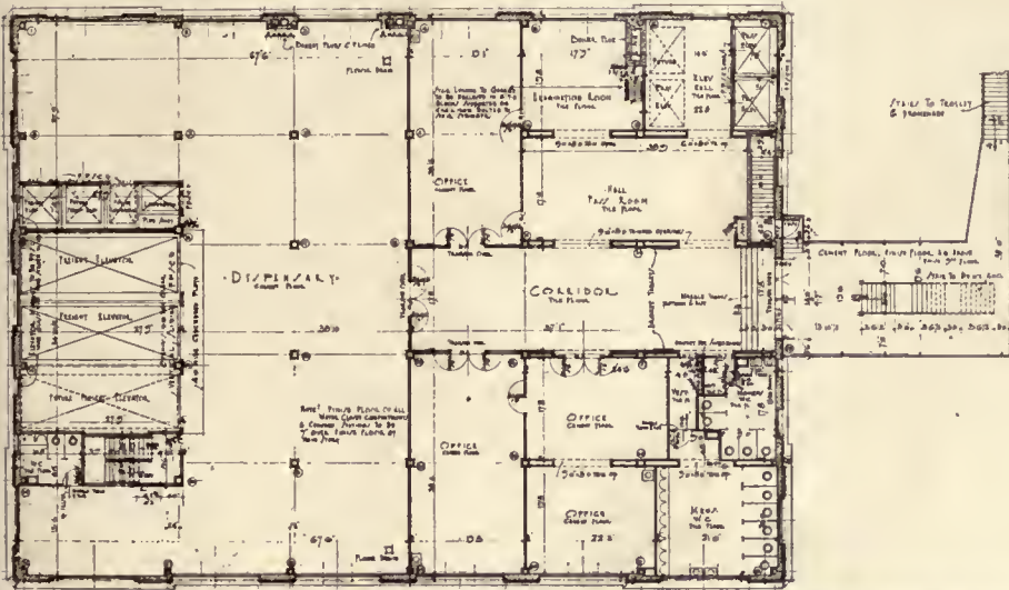
FIRST FLOOR PLAN—MAIN ENTRANCE AT RIGHT
