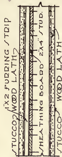
VERTICAL SECTION
