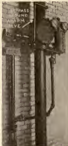
FIG 3. THE ARRANGEMENT OF VALVE HERE SHOWN IS IDENTICAL WITH REGULAR SYSTEM EXCEPT FOR THE BY-PASS.
