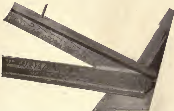
WELDED INTERSECTION OF UPPER AND LOWER TRUSS CHORDS
