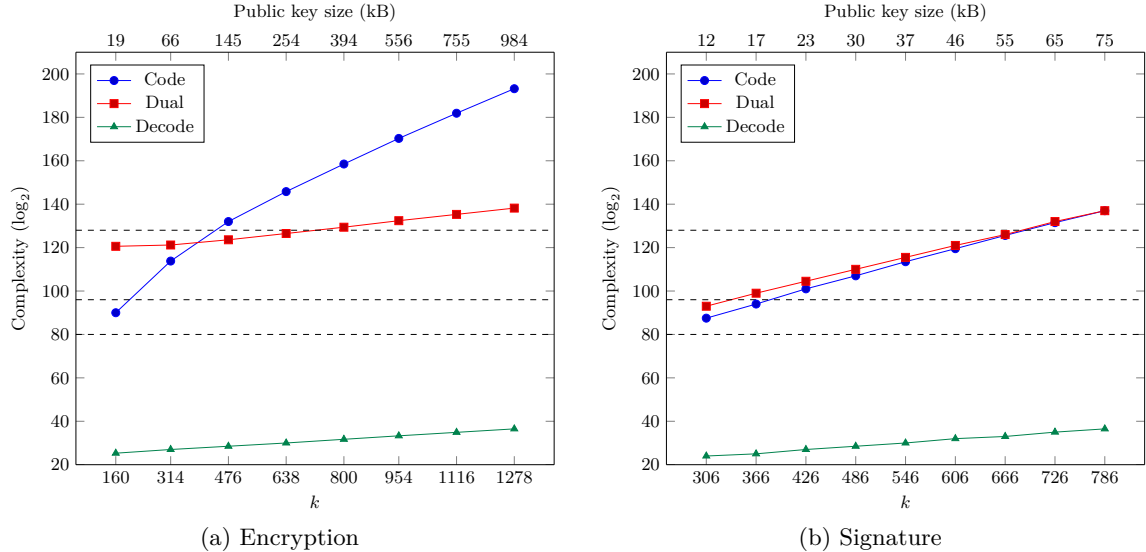
Fig. 3. Comparison between the complexity of decoding and the distinguishing attacks for encryption and signature. Dashed horizontal lines denote three security levels: 2^{80} , 2^{96} and 2^{128} .
