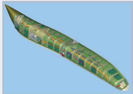
F-16 Conformal Fuel Tank Detailed Design & Production at Lahav
