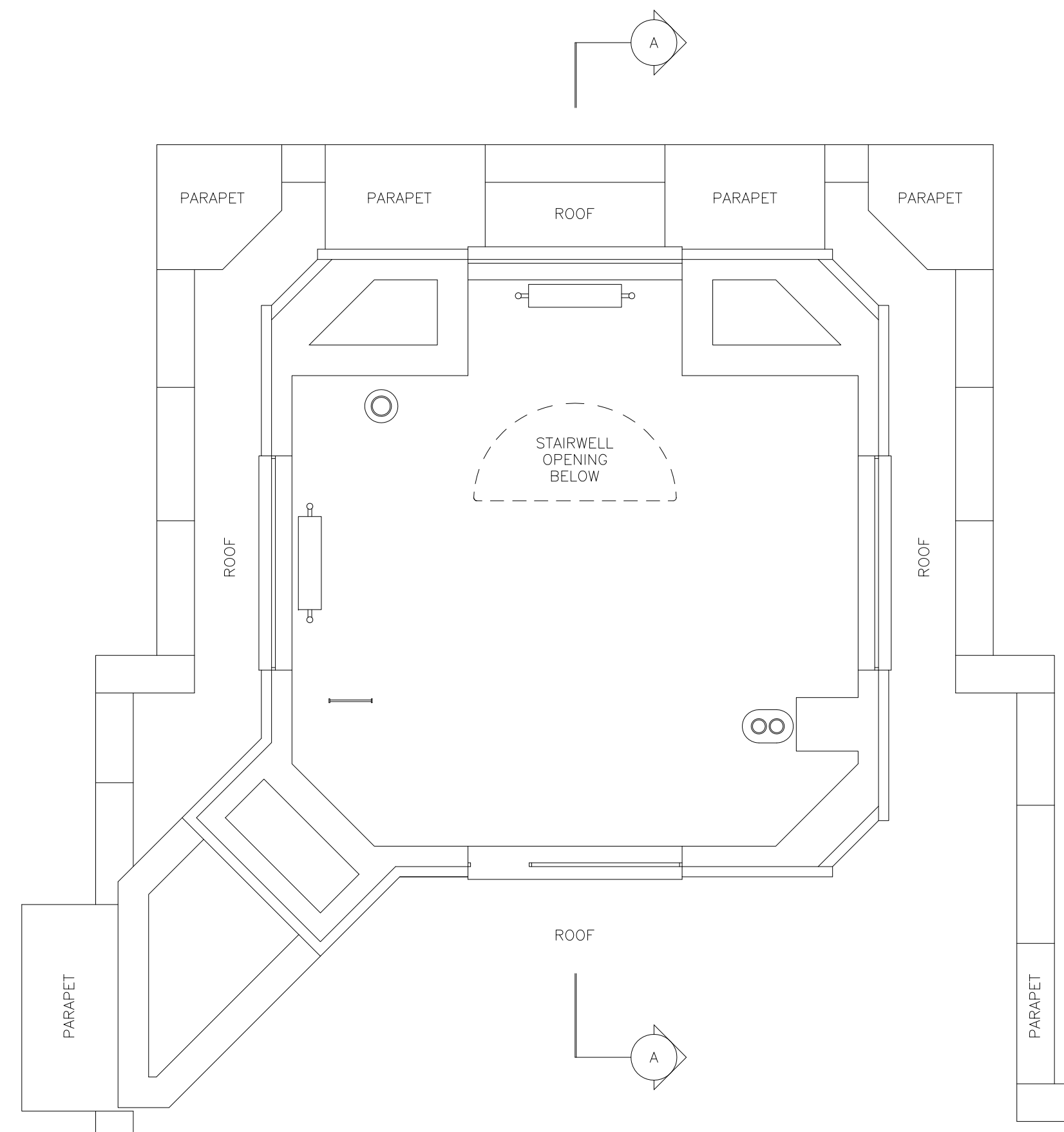
ROOF BULKHEAD PLAN BELOW HOUSE TANK
