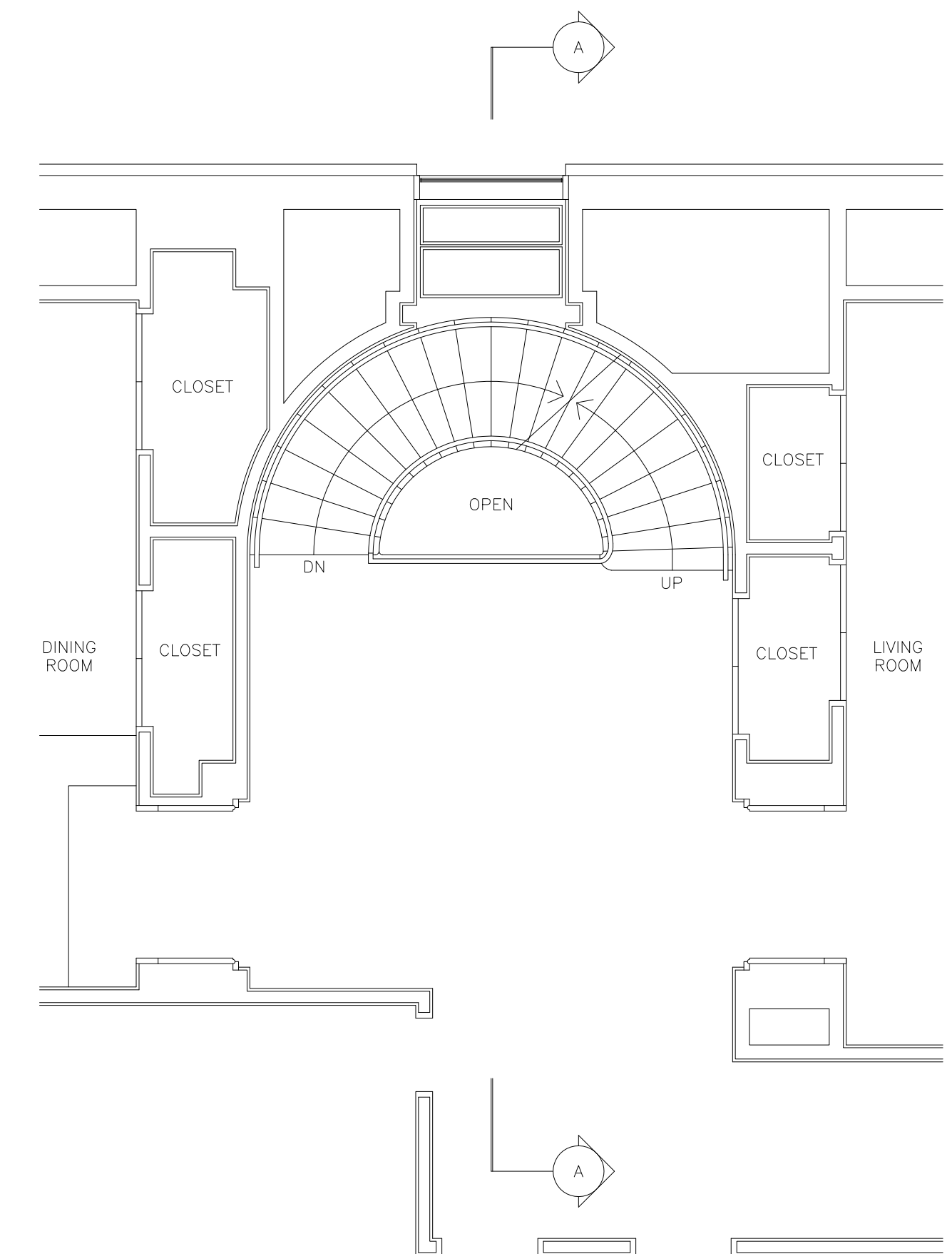
15TH FLOOR PLAN
