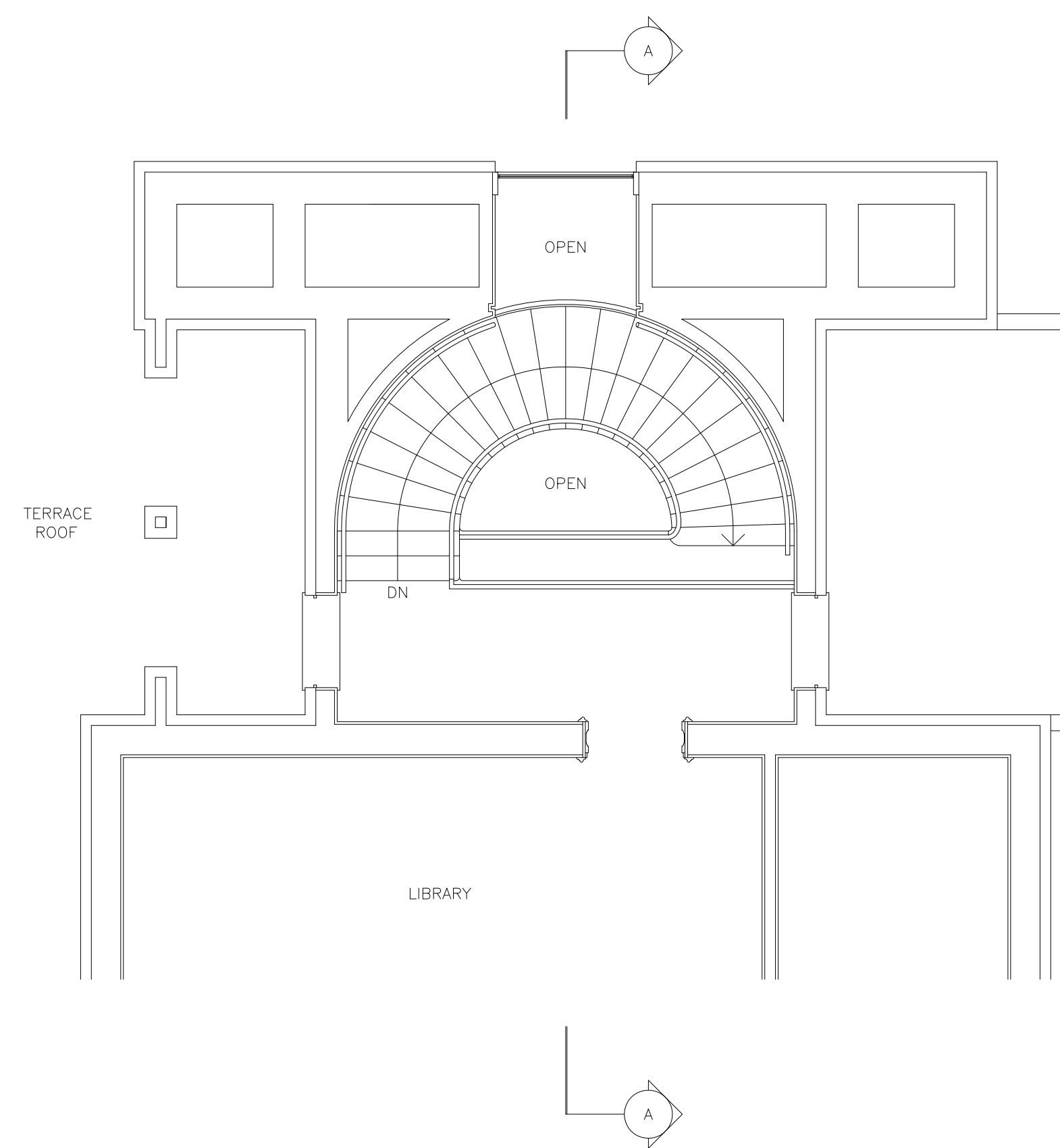
16TH FLOOR PLAN
