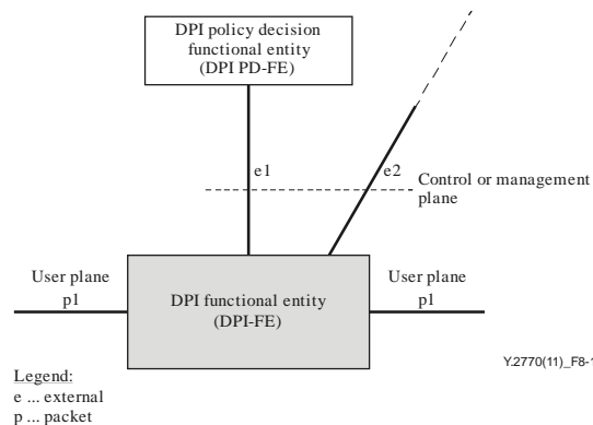
Figure 8-1 – External DPI-FE interfaces
