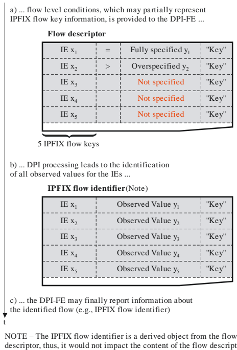
Figure A.2 – Flow Descriptor, IPFIX Flow Identifier and IPFIX Flow key example
