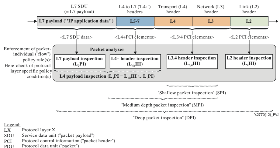
Figure V.1 – Packet Inspection – Illustration of Terminology
