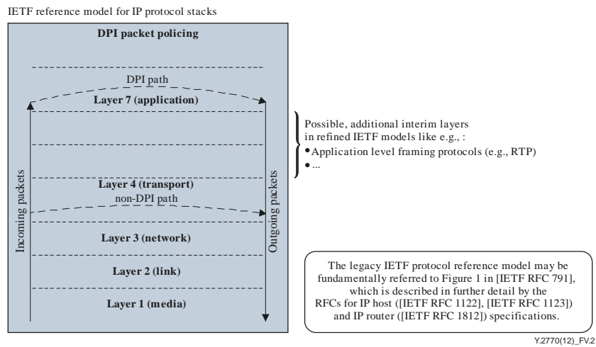
Figure V.2 – IETF (Basic and extended) Reference Model for IP
