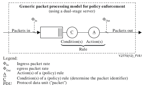
Figure VII.1 – Generic Model for Rule-oriented Packet Processing
