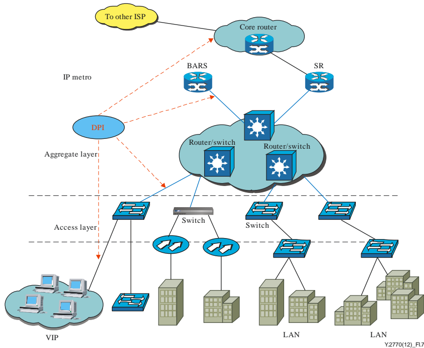
Figure I.7– Scenario of DPI's Deployment in packet-based network
