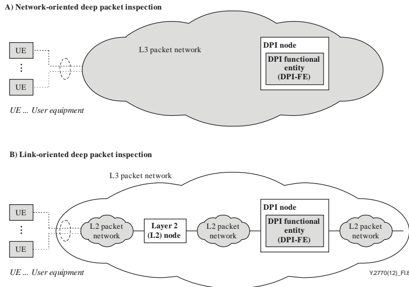
Figure I.8 – Network- vs. Link-oriented DPI
