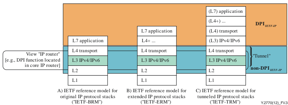
Figure V.3 – DPI examples for packets according other IETF reference models
