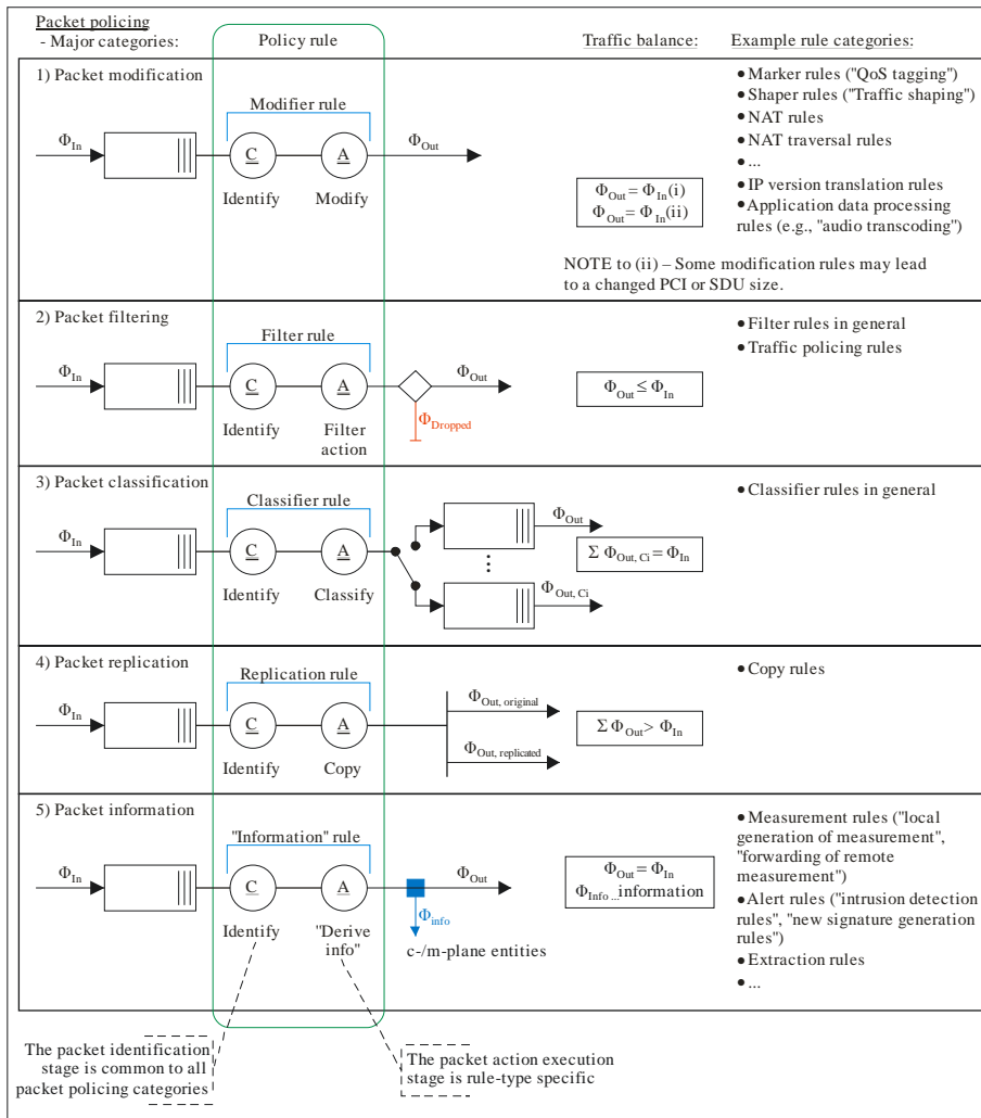
Figure VII.2 – Specific Models for the major categories of Packet Policing
