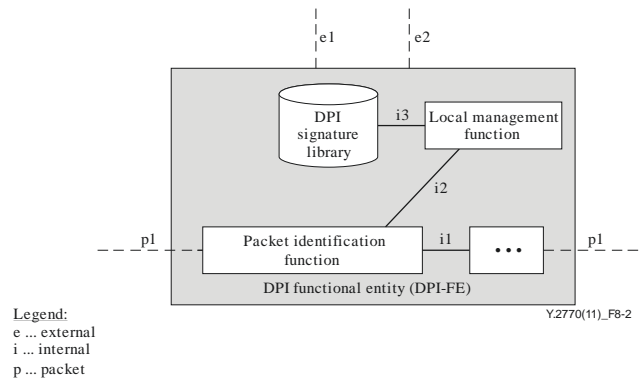
Figure 8-2 – Internal DPI-FE interfaces
