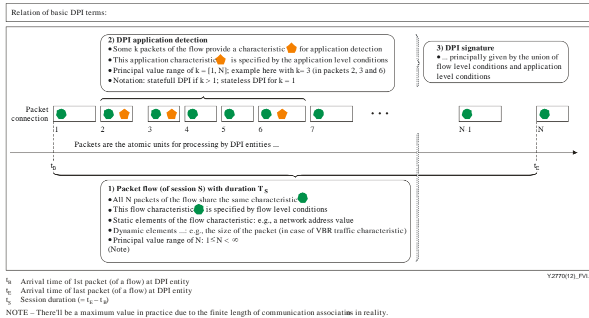
Figure VI.1 – Illustration of the three major terms flow descriptor , application descriptor and DPI signature
