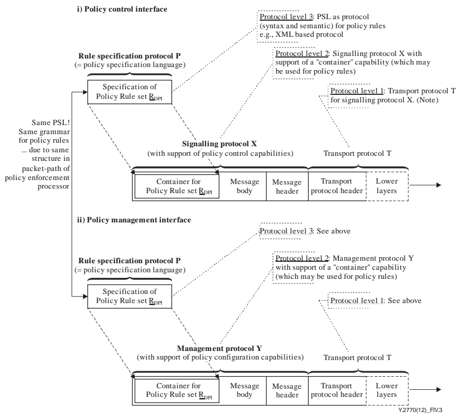
Figure IV.3 – Policy Specification Languages – Possible PSL Architecture Concept
