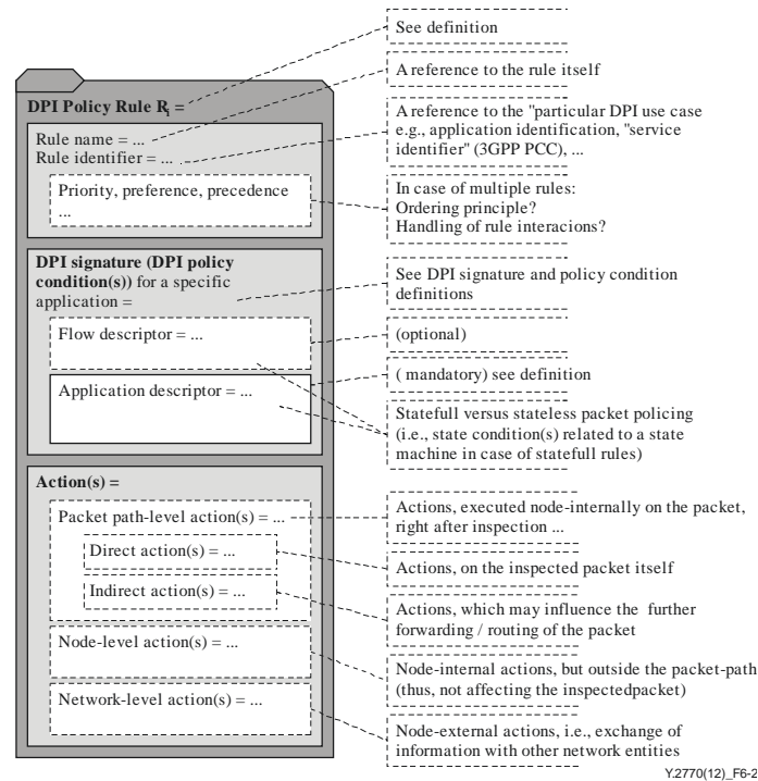
Figure 6-2 – An example of detailed Policy Rule format (in comparison to Figure 1-2/clause 1.2))
