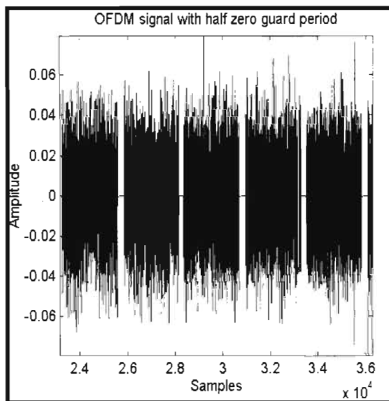
Fig. 3. OFDM Signal With Guard Period From Lawrey, Chapter 1.
