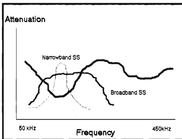
Fig. 4. Powerline Attenuation and Spread Spectrum. From Adaptive Networks.
