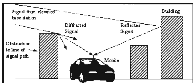
Fig. 2. Multipath Interference From Lawrey, Chapter 1.
