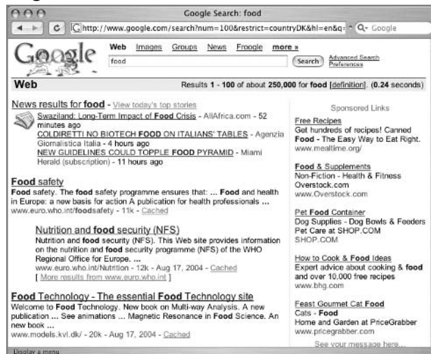
Figure 1.20 Using restrict to Narrow Results
