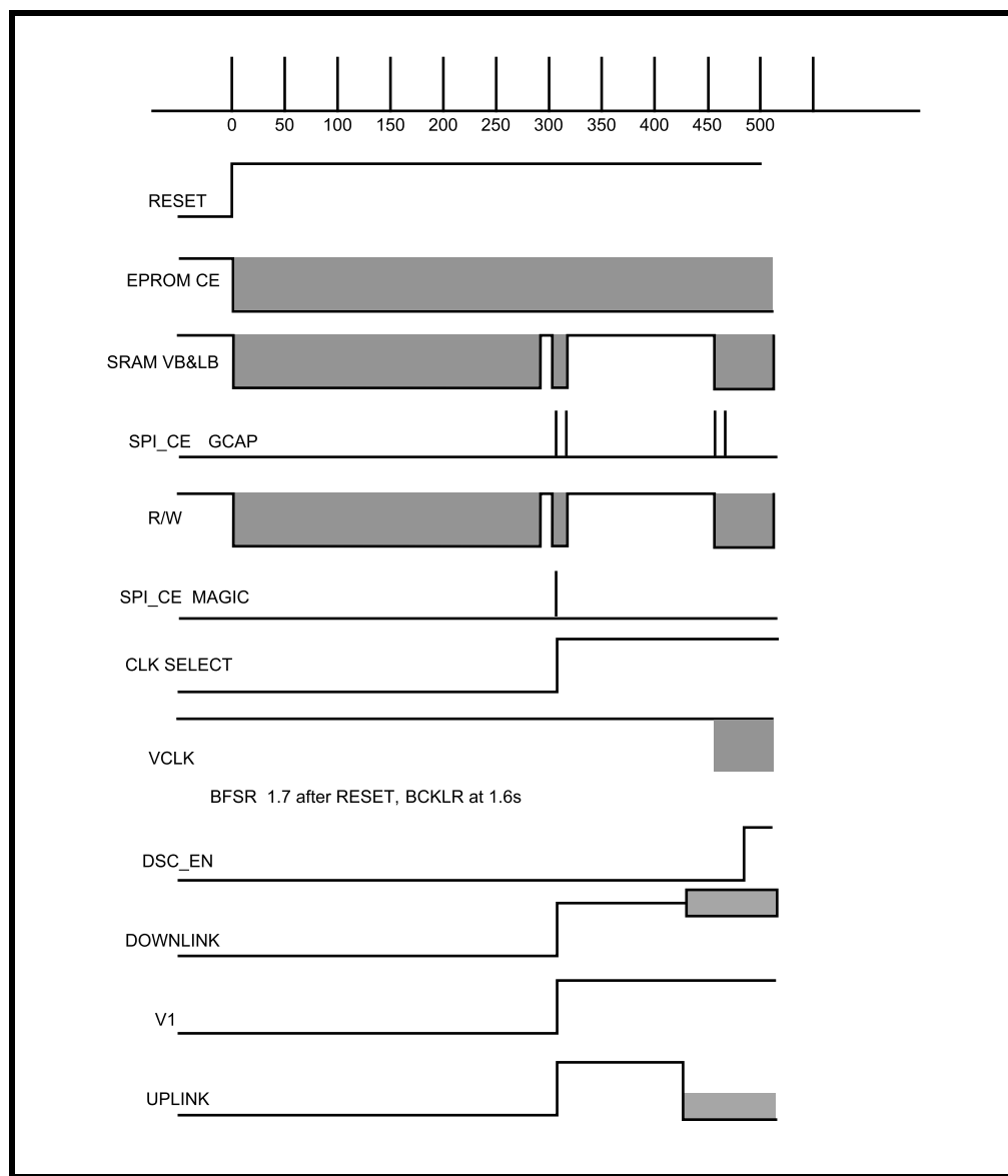
Figure 8. Power-up Sequence Timing Diagram
