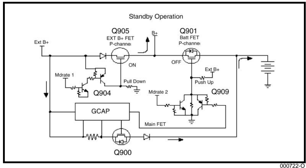
Figure 10. Standby Operation Battery Charging
