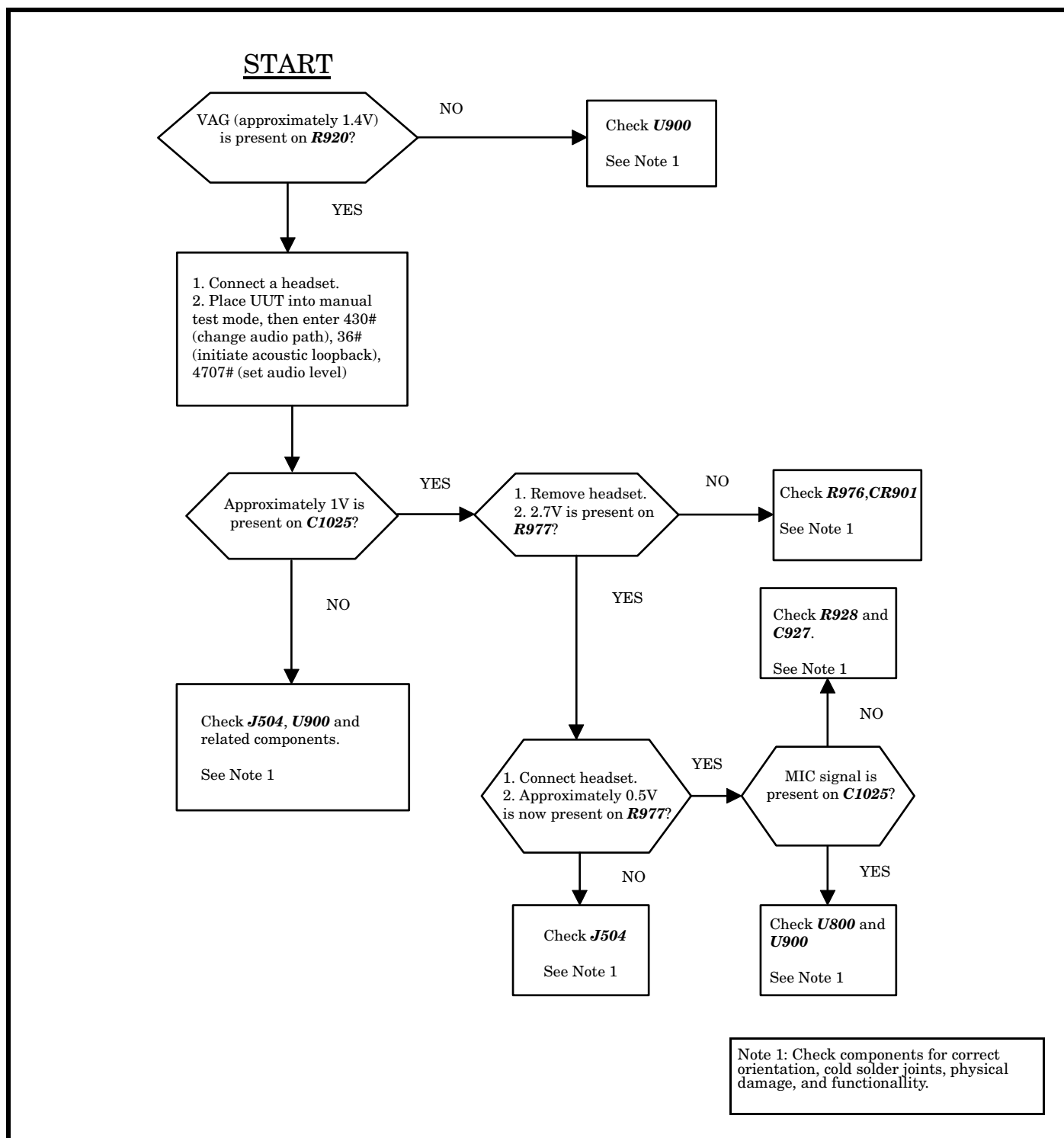
Figure 29. Headset Microphone Not Functioning
