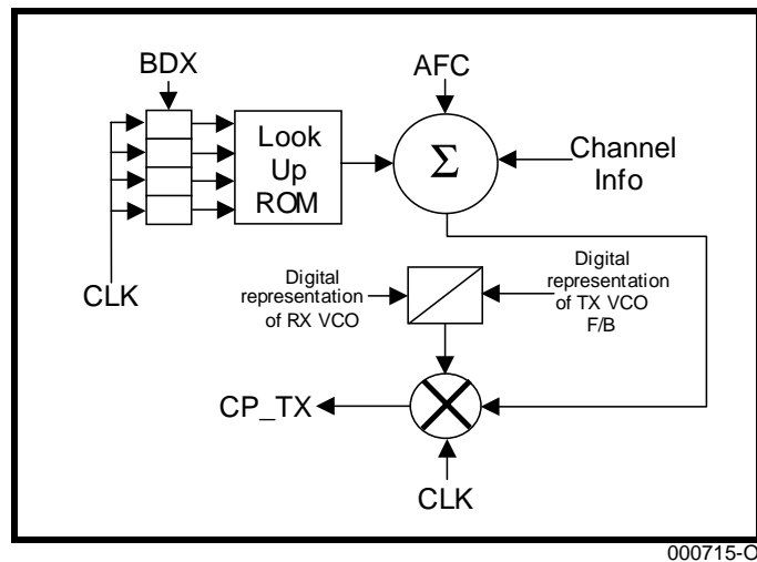
Figure 3. Magic IC Internal Transmit Path
