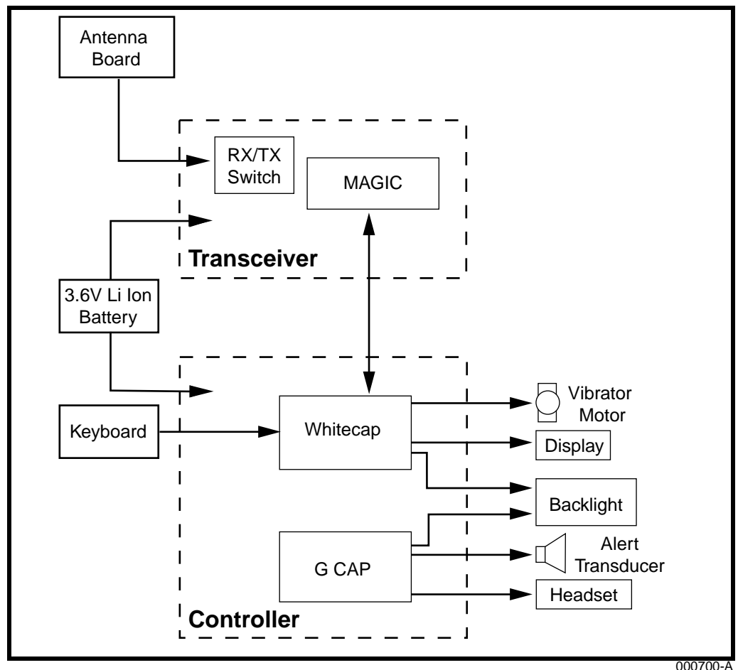
Figure 1. Simplified Functional Block Diagram
