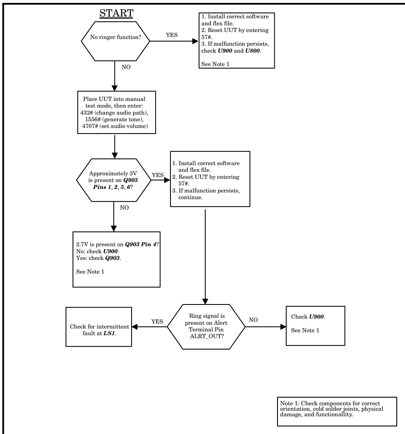
Figure 27. No Ring Tone
