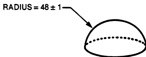
Figure 12. Hemispherical Anvil
