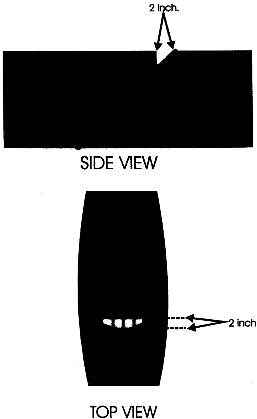
FIGURE 14 to part 227--Shortened Webbing Over the Escape Opening Complying With Requirement at 50 CFR 227.72(e)(2)(v)(A)(4)
