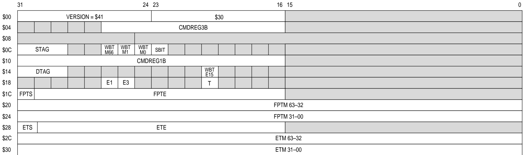
Figure B-22. MC68040 Unimplimented Instruction Stack Frame
