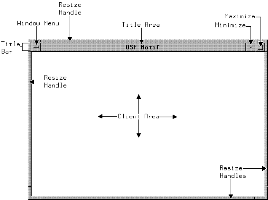
Figure 1 The Client Window Frame
