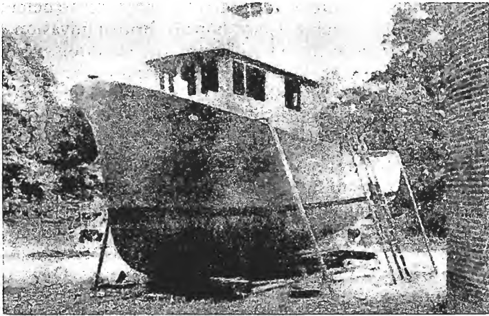
Atlantis II, the ferrocement ship built by Operation Atlantis, shortly before launching (from Atlantis News).
