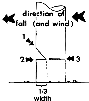
Chainsaw felling; note sequence of cuts.
