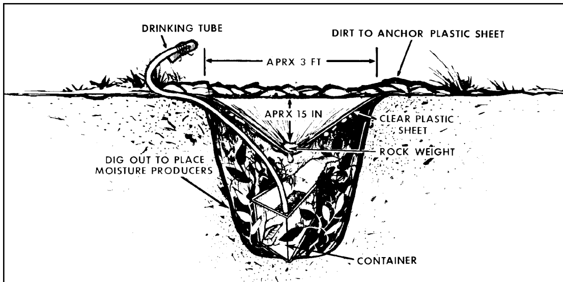
Figure VII-7. Solar Still
