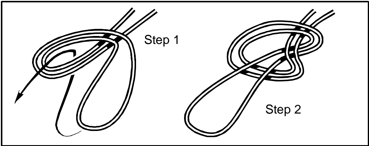
Figure IV-3. Fixed Loop
