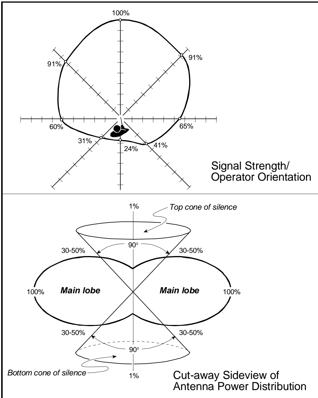
Figure III-1. Radio Transmission Characteristics
