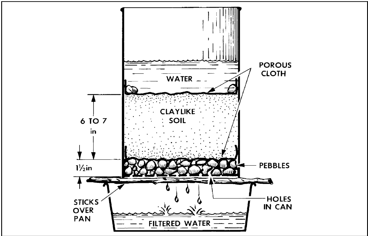
Figure IX-4. Filtration Systems, Filtering Water
