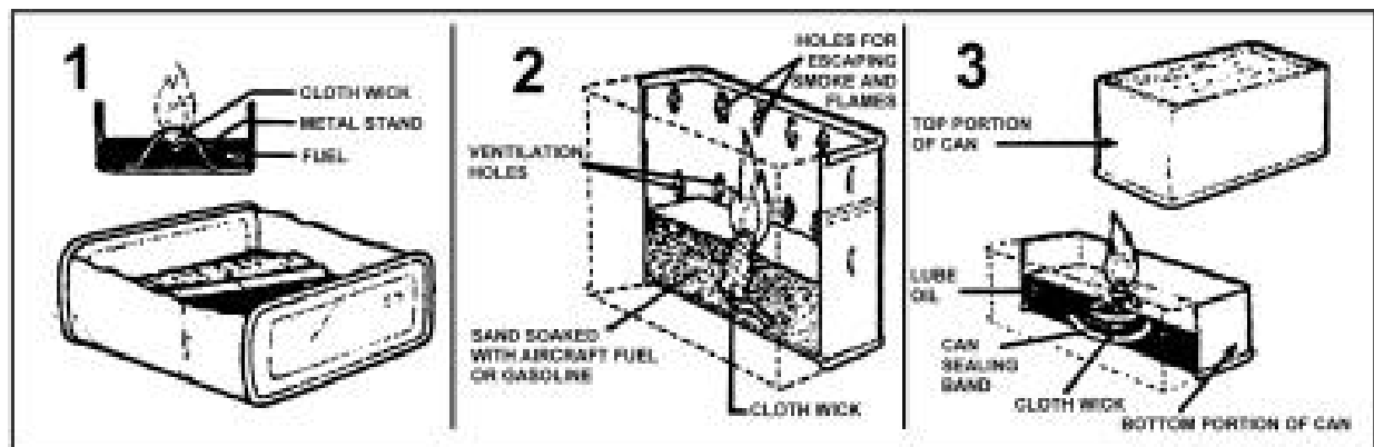
Figure VI-16. Improved Stove
