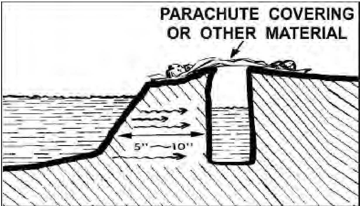
Figure IX-5. Filtration Systems, Settling Water
