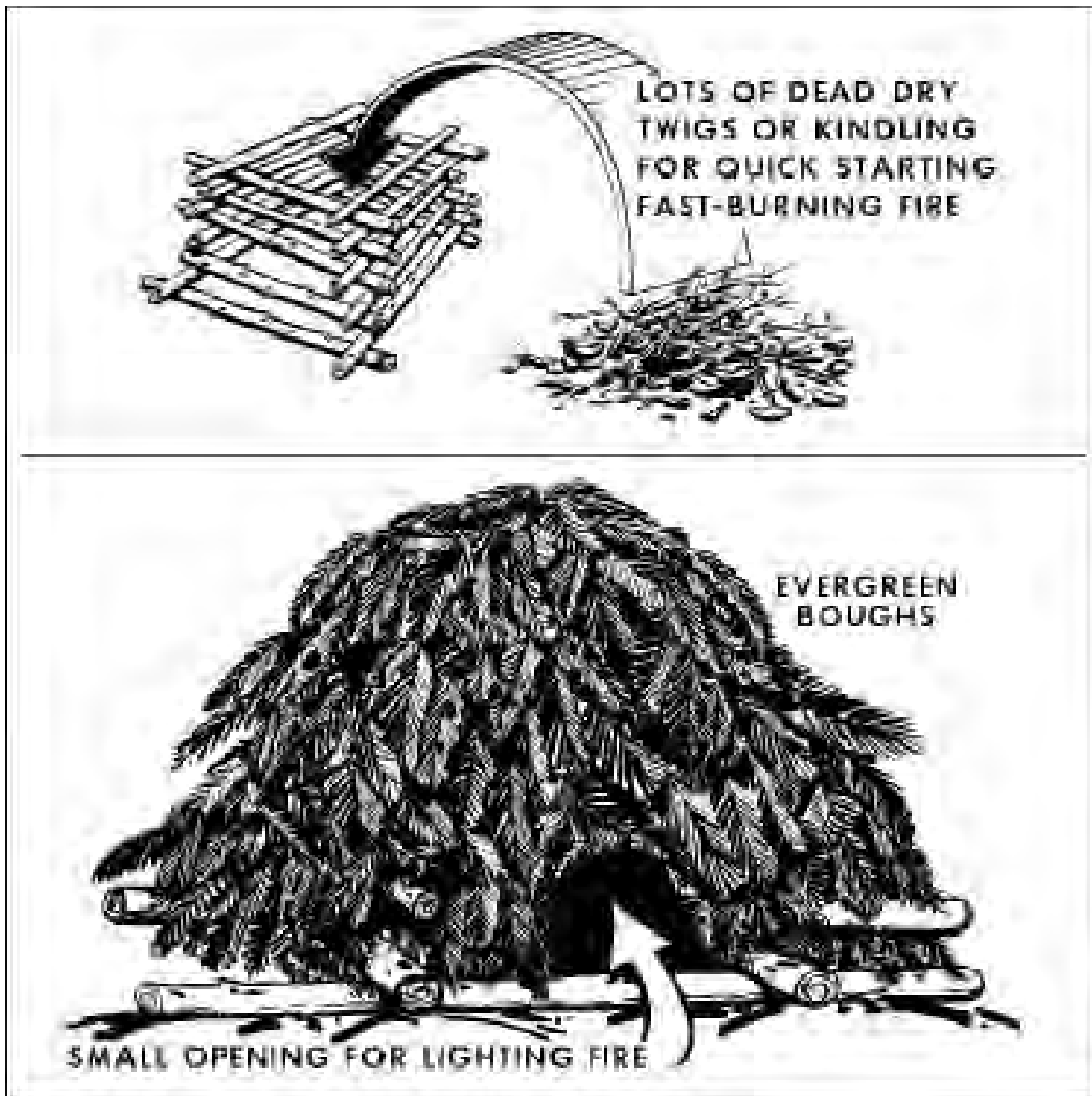
Figure III-5. Smoke Generator
