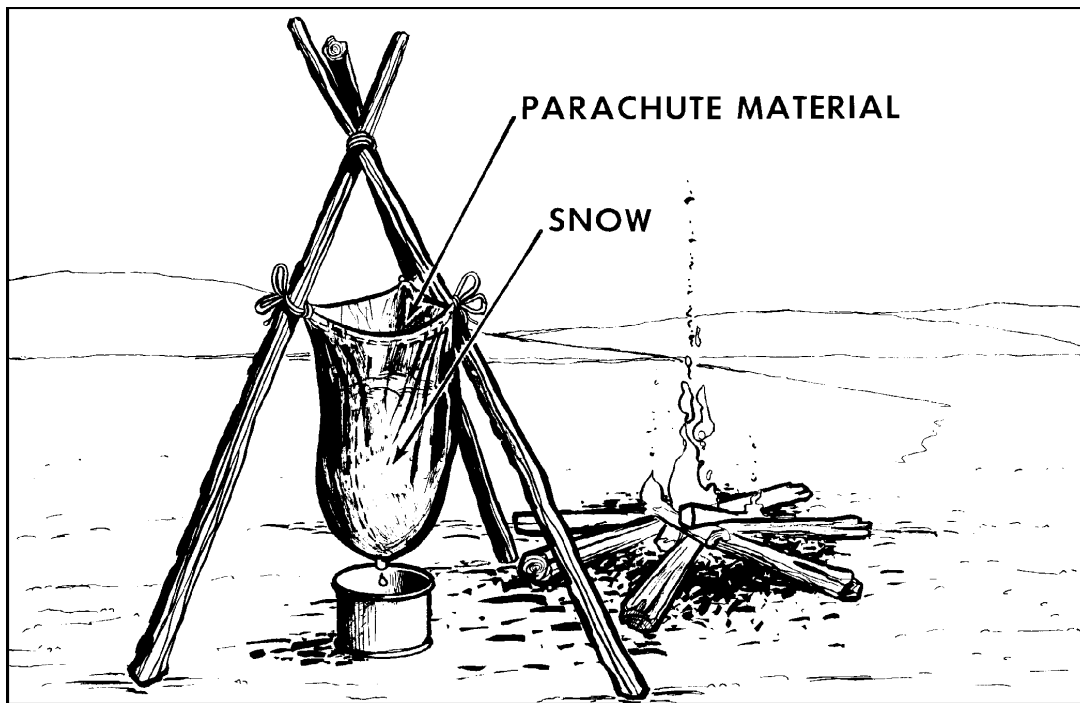
Figure VII-3. Water Generator
