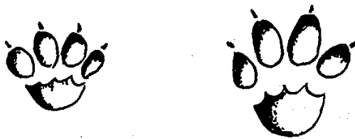
The typical pug marks of flesh-eating mammals. In Australia these are usually made by the wild dingo and the ferral cat.
