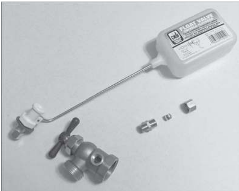
An evaporative cooler float valve can be repurposed to automatically top up an aquaponics tank.
