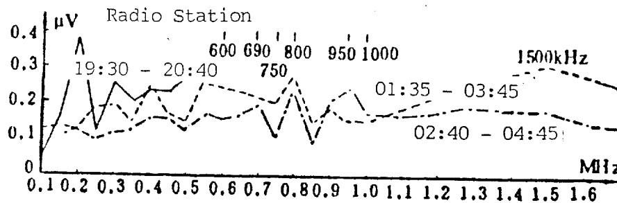
Figure 5. Experimental curves from an unshielded room where electro-magnetic waves were received by the metal needle.
