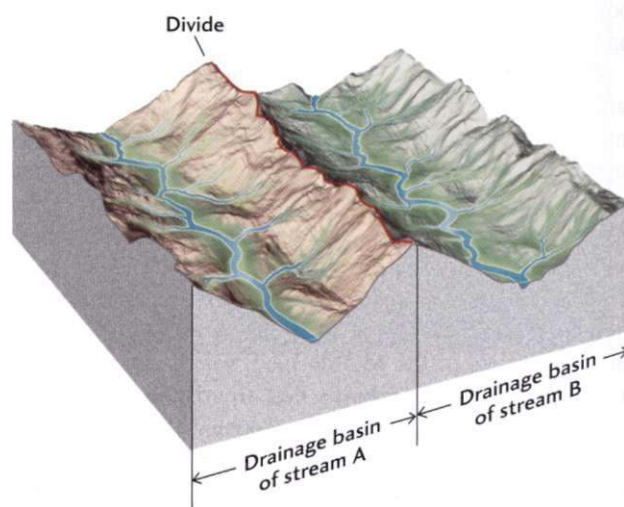
Figure 18.5 Stream valleys and drainage basins are separated by divides, which may be ridges, gentle uplands, or mountain ranges.
