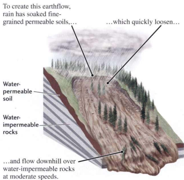
Figure 16.22 An earthflow is a movement of relatively fine grained materials that travel as fast as a few kilometers per hour. Earthflow, Hogan Creek, Denali National Park, Alaska. [Steve McCutcheon/Visuals Unlimited.]
