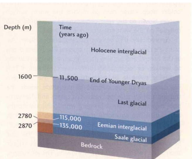
Comparison of ice depths and time before the present for recent glacial and interglacial intervals. [After J. W. C. White, "Don't Touch That Dial." Nature 364 (1993): 186.]
