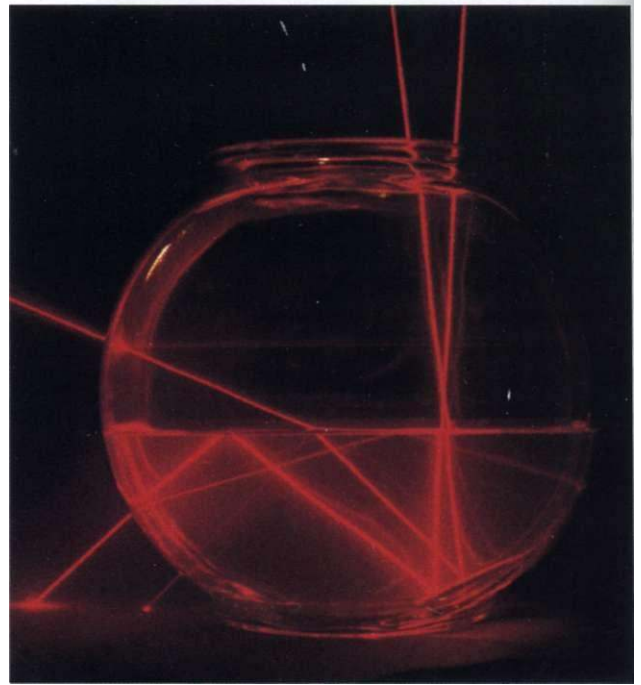
Figure 14.1 In this experiment, two beams of laser light enter a bowl of water from the top. Both beams are reflected from a mirror on the bottom of the bowl. One is then reflected at the water-air interface and passes through the bowl to make a bright spot on the table. Most of the energy from the other beam is bent downward (refracted) as it passes from the water to the air, although a small amount is reflected to form a second spot on the table. You can also trace the paths of other beams reflected by the interfaces. [Susan Schwartzberg/The Exploratorium.]
