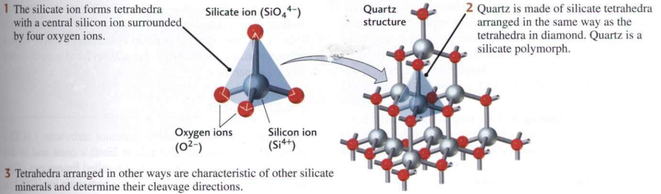
Key Figure 3.9 Common silicate minerals are polymorphs of silicate ions and often other elements.
