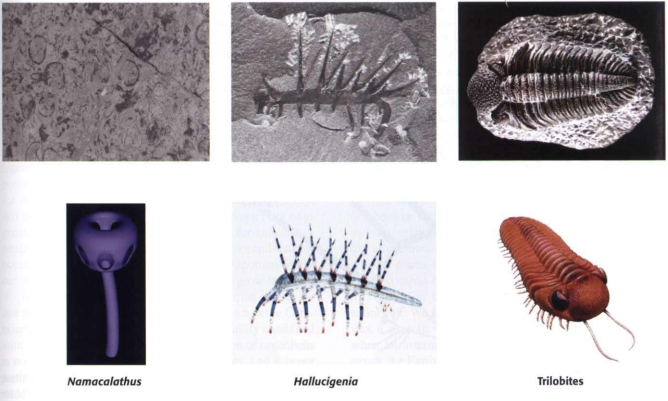
Figure 11.18 Fossils that record the Cambrian explosion include Precambrian calcified fossils (left) that were the first organisms to use calcite in making shells. These, along with other organisms, became extinct at the Precambrian–Cambrian boundary, which helped pave the way for a strange new group of organisms, including Hallucigenia (center) and the more familiar trilobites (right). Both of these organisms formed weak shells
