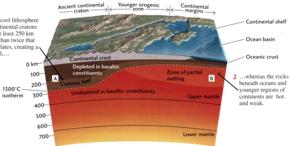
Key Figure 10.24
