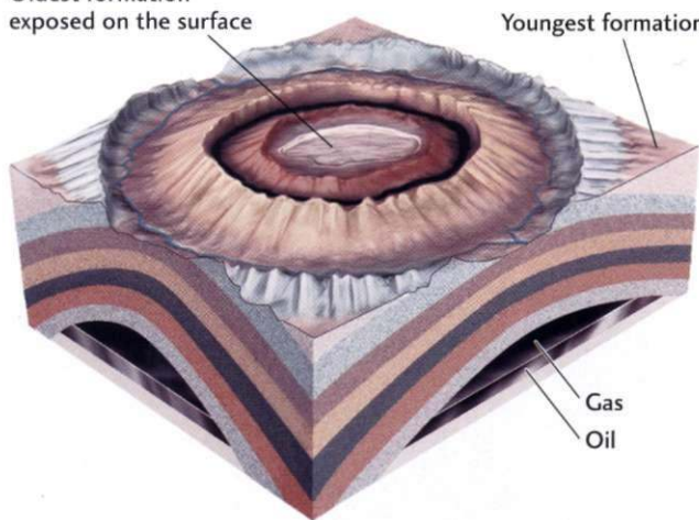
Figure 7.12 Sinclair dome, an eroded dome in strata 10 km east of Rawlins, Wyoming. The highway and railroad at the lower right suggest the dome's dimensions. The characteristic circular outcrop pattern of a dome and the extension to the subsurface are shown in the diagram. The oldest bed is in the core; the flanking formations are successively younger and dip away from the core. [Photo by John S. Shelton.]
