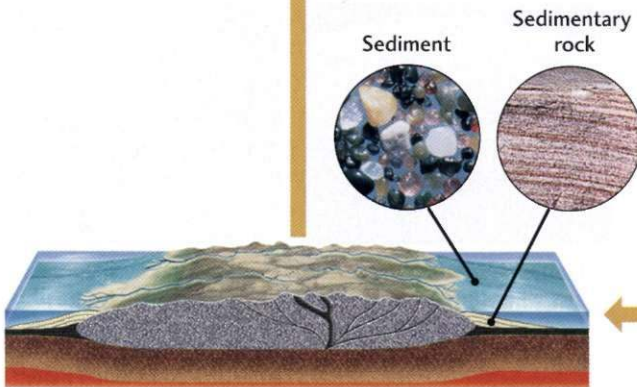
Sedimentary rock
