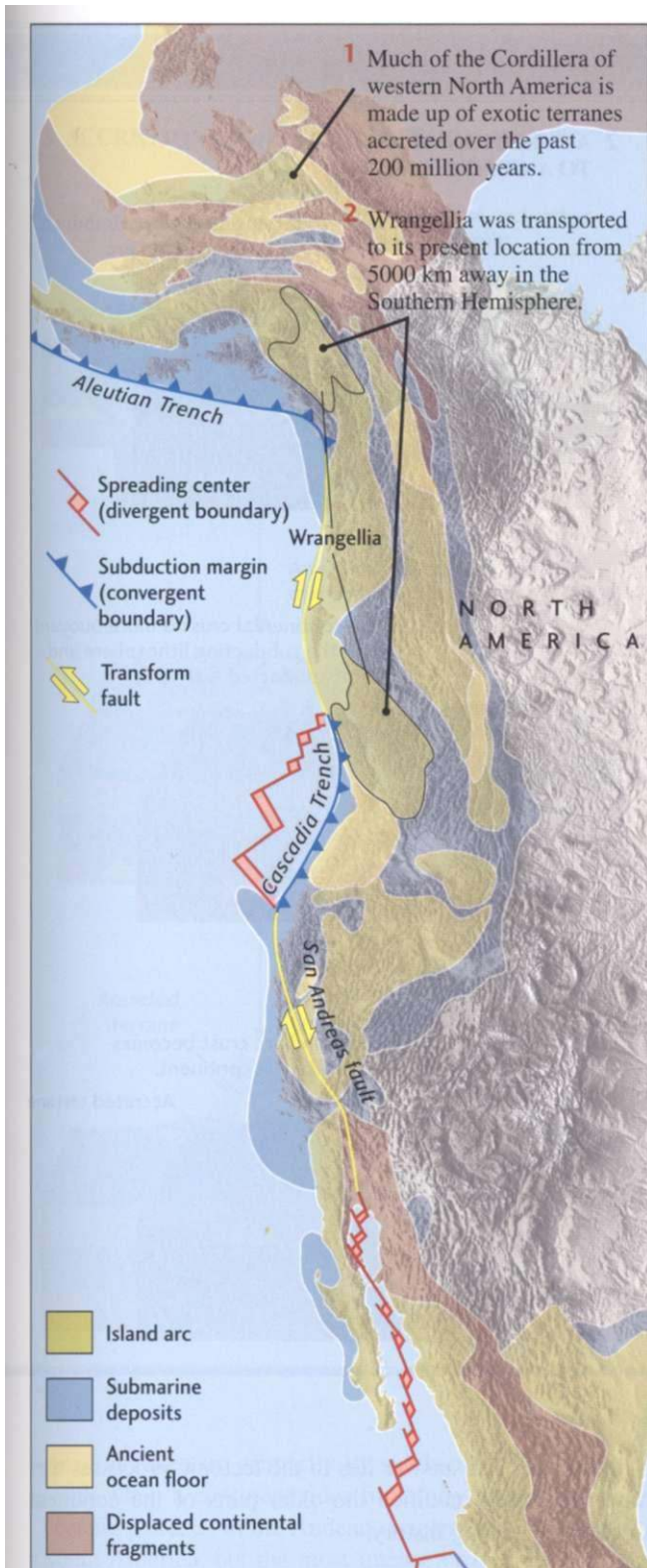
Figure 10.1 Terranes accreted to western North America in the past 200 million years. They are made up of island arcs, ancient seafloor crust, continental fragments, and submarine deposits. [After D. R. Hutchison, "Continental Margins." Oceanus 35 (Winter 1992–1993): 34–44; modified from work of D. G. Howell, G.W. Moore, and T.J. Wiley.]
