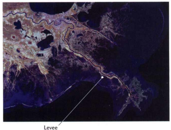
Figure 18.4 The formation of natural levees by river floods. Natural levees along the main channel of the Mississippi River near South Pass, Louisiana. [USGS National Wetlands Research Center.]
