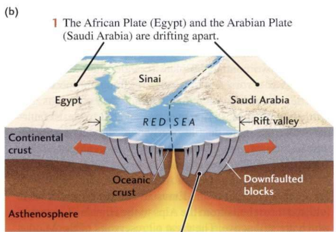
2 Tensional forces have created a rift valley—the result of downfaulted blocks—filled by the Red Sea.
