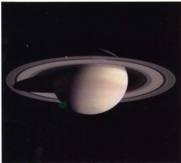
Figure 9.28 (a) Saturn and its rings completely fill the field of view in this natural color image taken by the Cassini spacecraft on March 27, 2004. Color variations in the rings reflect differences in the composition of materials that make them up, such as ice and rock. Cassini scientists will investigate the nature and origin of the rings as the mission progresses. (b) The surface of Titan is strewn with rocks of ice composed of frozen methane and other carbon-containing compounds. [Images from NASA/JPL/SSI/ESA/University of Arizona.]
