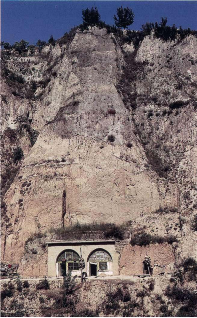
Figure 19.14 Comfortable dwelling caves hand-carved into steep cliffs of loess in central China. These deposits of windblown dust accumulated in the past 2.5 million years, reaching a thickness of as much as 400 m. [Stephen C. Porter]
