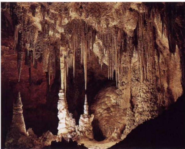
Figure 17.17 Chinese Theater, Carlsbad Caverns, New Mexico. Stalactites from the ceiling and stalagmites from the floor have joined to form a column. [David Muench.]
