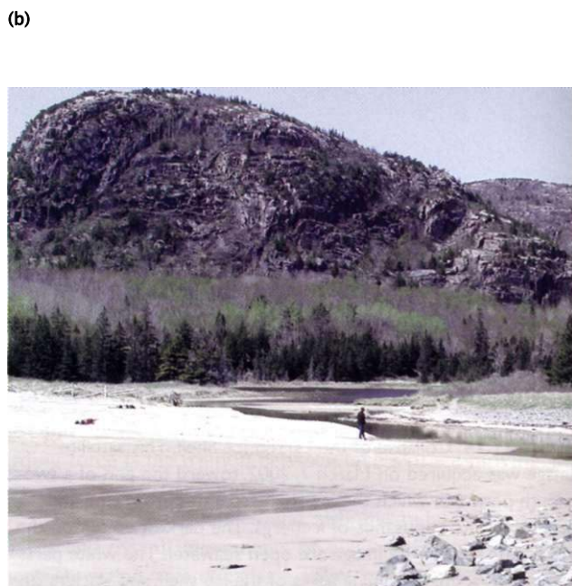
cracks, (b) A roche moutonnée known as The Beehive rises above Sand Beach at Acadia National Park in Maine. [Robert E. Nelson, Colby College.]
