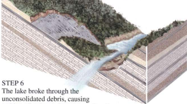
Figure 16.27 The 1925 Gros Ventre slide. [After W. C. Alden, "Landslide and Flood at Gros Ventre, Wyoming." Transactions of the American Institute of Mining, Metallurgical, and Petroleum Engineers (1928): 345–361.] The Gros Ventre landslide, Grand Teton National Park, Wyoming. [Steven Dutch.]
