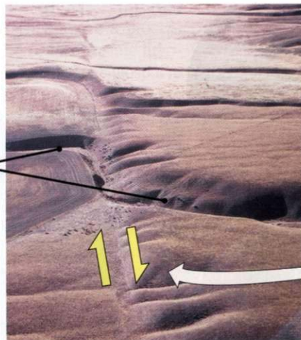
Figure 2.9 The view northwest along the San Andreas fault in the Carrizo Plain of central California. The San Andreas is a transform fault, forming a portion of the sliding boundary
