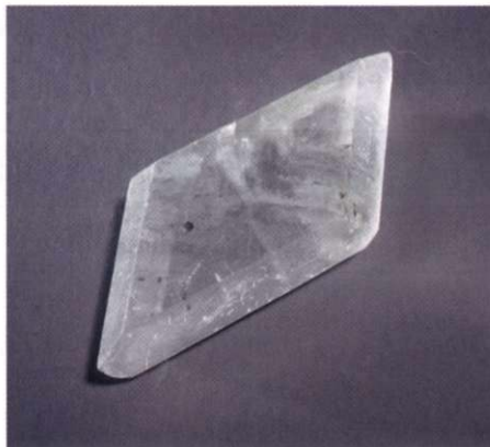
(b) Gypsum
