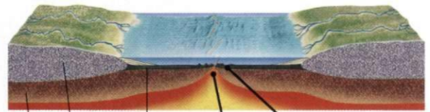
Oceanic crust Continental crust Continental lithosphere
