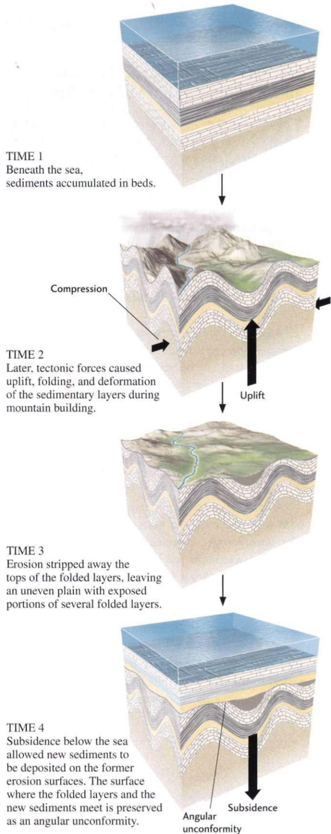
Figure 8.8 An angular unconformity is a surface of erosion that separates two sets of layers having bedding planes that are not parallel. This sequence shows how such a surface can form.
