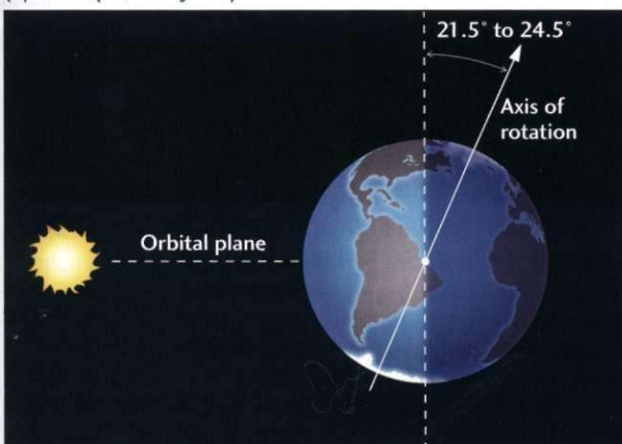
(b) Tilt (41,000 years)
