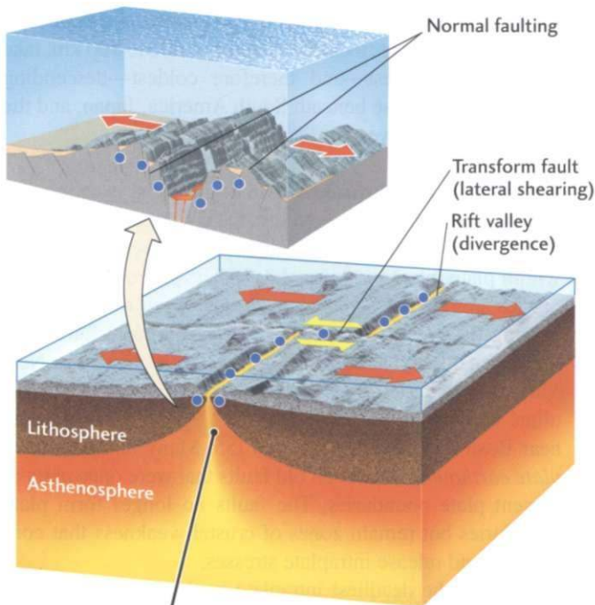
Mid-ocean ridge (divergence)
