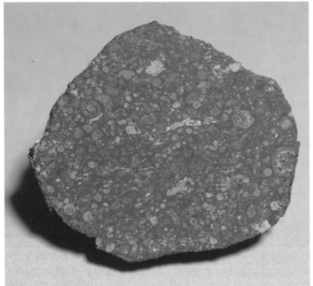
Figure 11.24 The Allende meteorite is full of organic compounds, some of which may have helped in the origin of life. This meteorite fell to Earth near Allende, Mexico, in 1969. [John Grotzinger/Ramon Rivera-Moret/Harvard Mineralogical Museum.]
