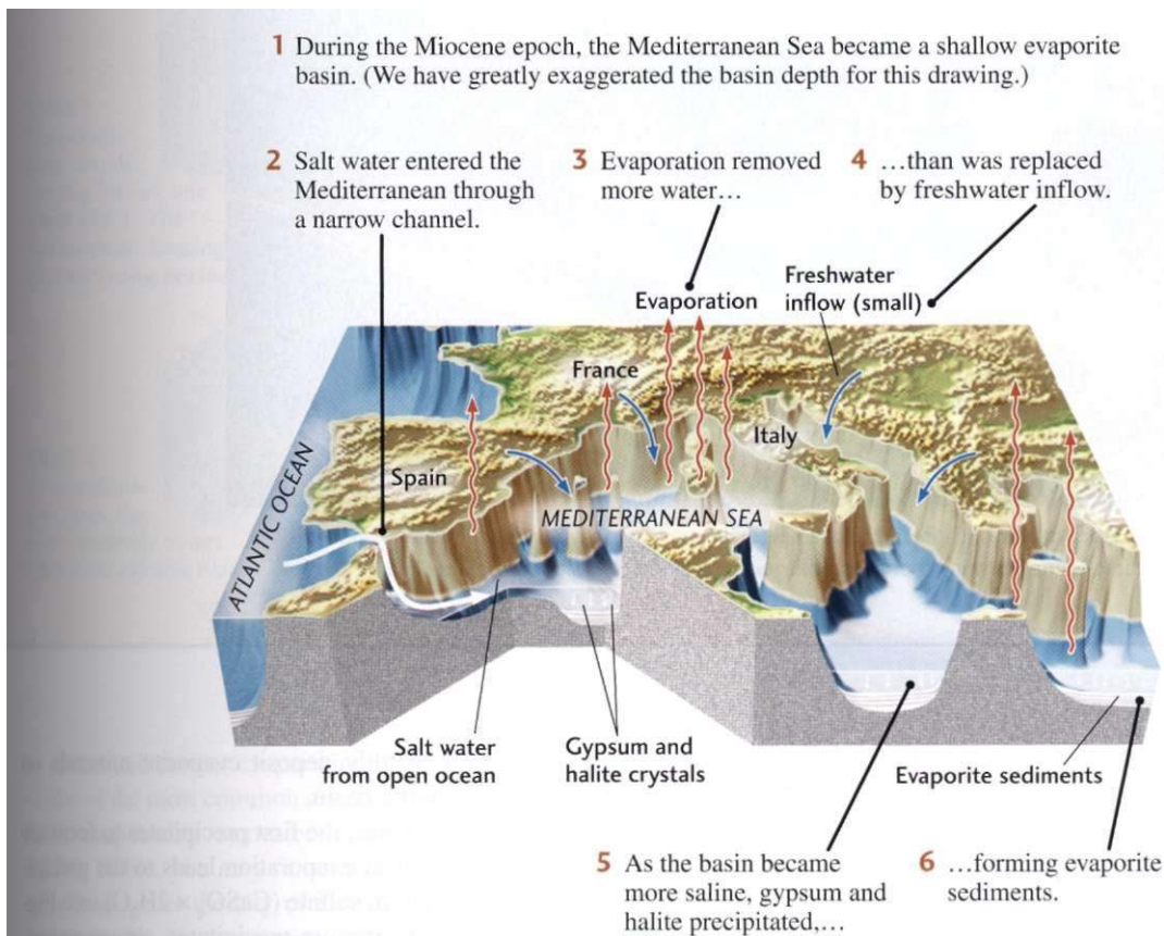
Figure 5.20 A marine evaporite environment. When seawater evaporated in a shallow basin, such as in the Mediterranean Sea, with a restricted connection to the open ocean, gypsum formed
