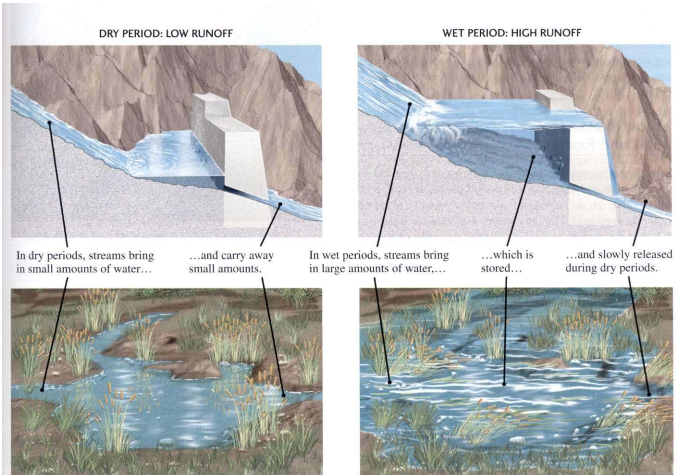
Figure 17.5 Like a natural lake or an artificial reservoir behind a dam, a wetland (such as a swamp or marsh) stores water
