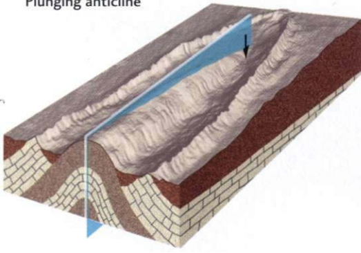
Plunging anticline
