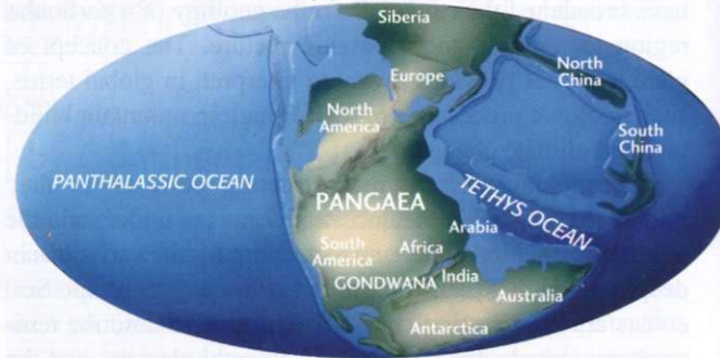
PANGAEA (a) Early Triassic, 237 Ma
