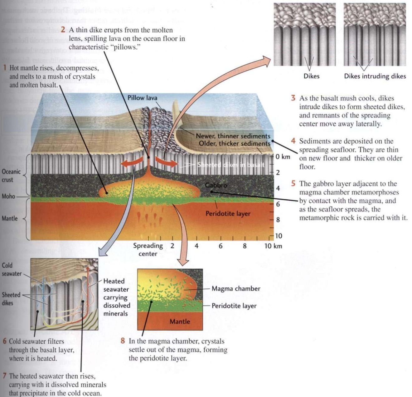
Key Figure 4.13 Decompression melting creates a magmatic geosystem at seafloor spreading centers.
