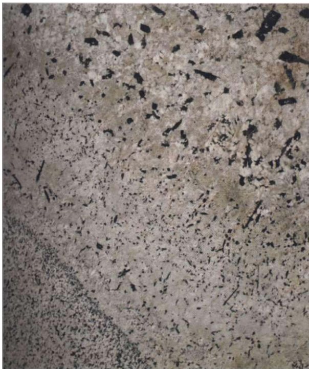
Figure 4.10 A granite pegmatite dike. The center of the intrusion (upper right) cools more slowly and developed coarser crystals. The margin of the intrusion (lower left) has finer crystals due to more rapid cooling. [John Grotzinger/Ramón Rivera-Moret/Harvard Mineralogical Museum.]
