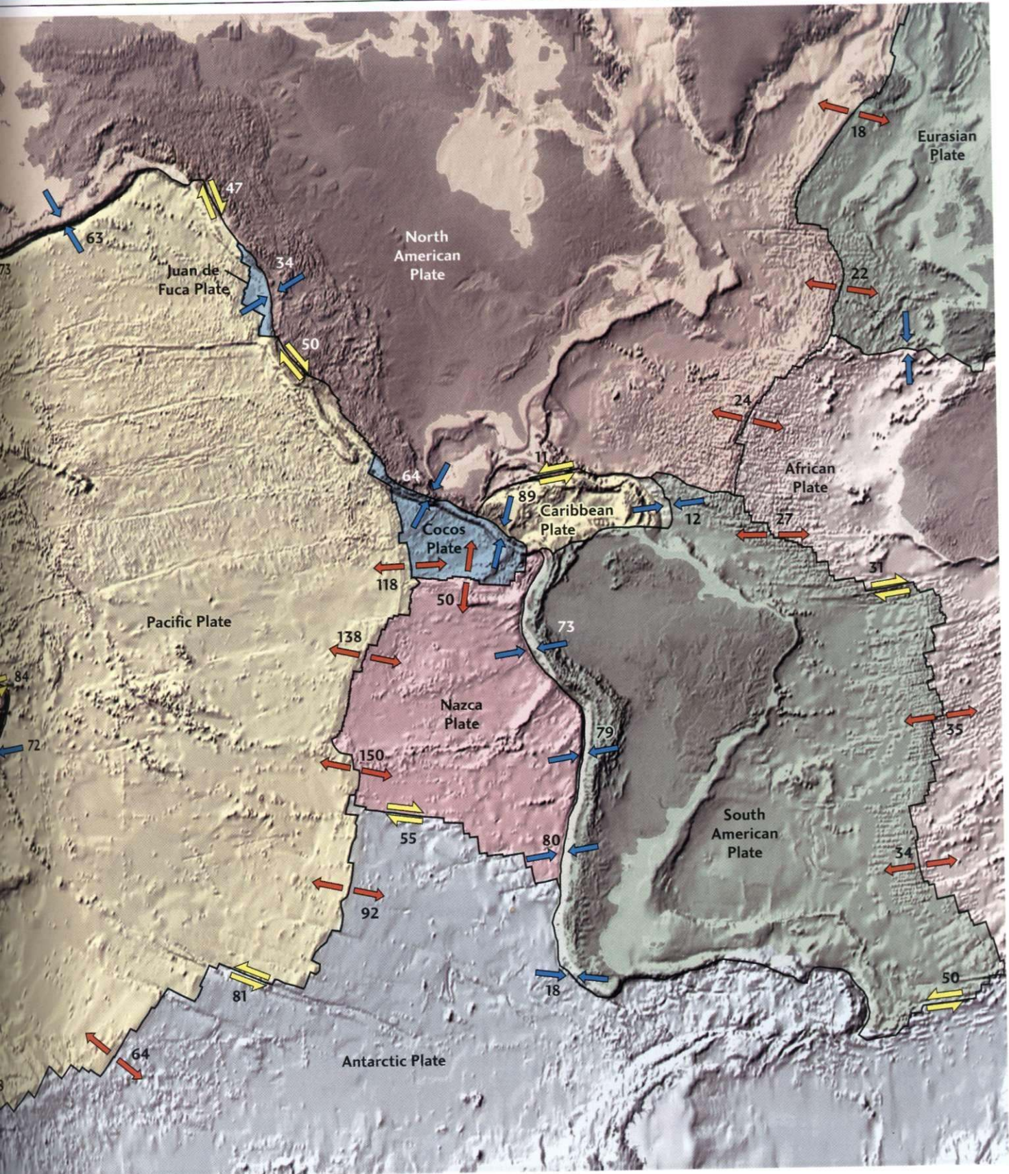
Plate boundaries by Peter Bird, UCLA
