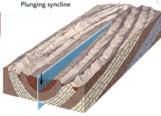
Figure 7.11 The geometry of plunging folds. Note the converging pattern of the layers where they intersect the surface, which you can also see in Figure 7.4.
