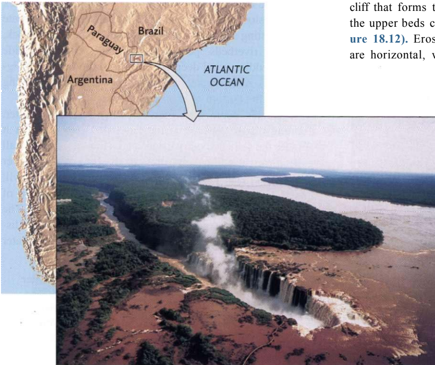
Figure 18.12 This waterfall on the Iguacu River, Brazil, is retreating upstream as falling water and sediment pound the cliff's base and undercut it. From the center to the upper left, one can see steep walls, the remnants of the waterfall's retreat upstream. [Donald Nausbaum.]
