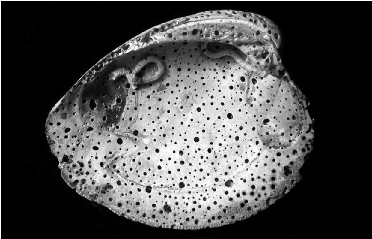
Fig. 4.13a Sponge borings (Entobia made by the genus Cliona) and encrusters on a shell of the modern hard clam, Mercenaria mercenaria , from North Carolina. This encrustation and boring happened after the death of the clam when the shell was empty. Image credit: ©Mark A. Wilson (Department of Geology, The College of Wooster).
