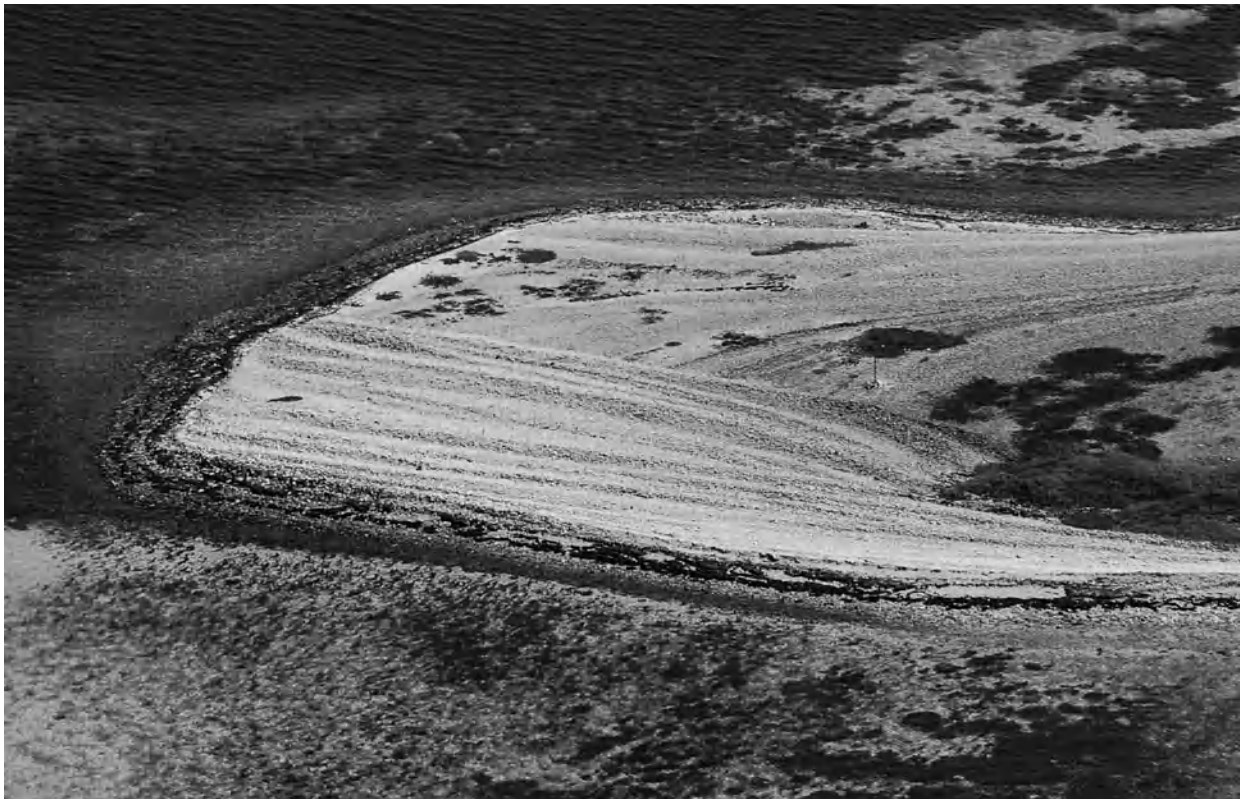
Fig. 5.70a,b Beach ridge systems composed of coarse coral rubble in the Abrolhos archipelago off Western Australia. (Photo credit: A. Scheffers).
