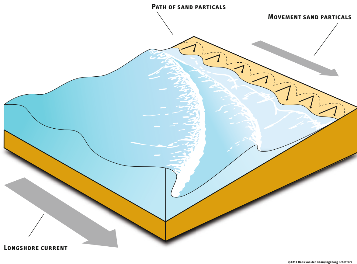
Fig. 8.32 The process of longshore drift by waves approaching with an angle to the coastline. If groynes or other obstacles are present, we normally find an accumulation at the luvward side and leeward erosion. If the coastlines set back, longshore drift may form a spit.
