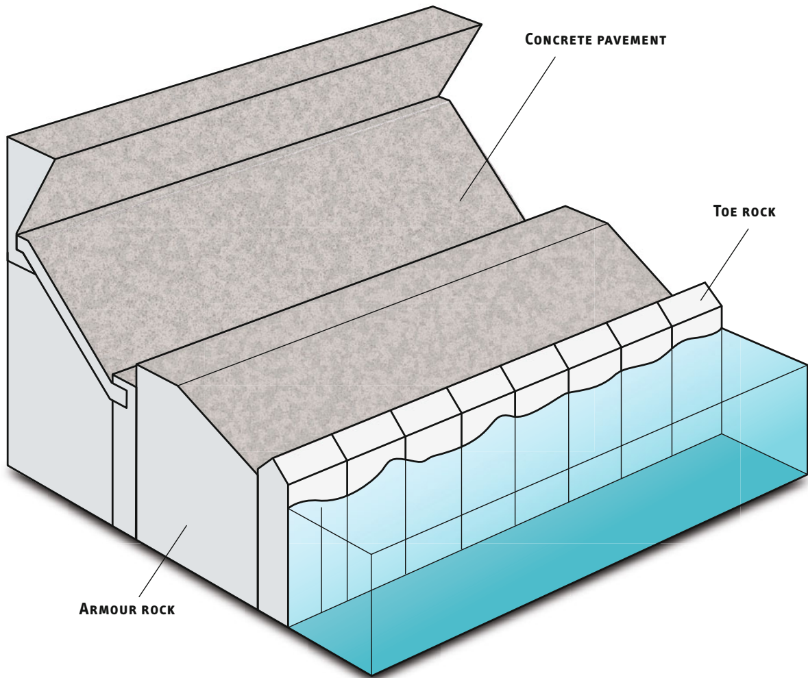
Fig. 8.35 Coastal protection techniques along the German North Sea coast.
