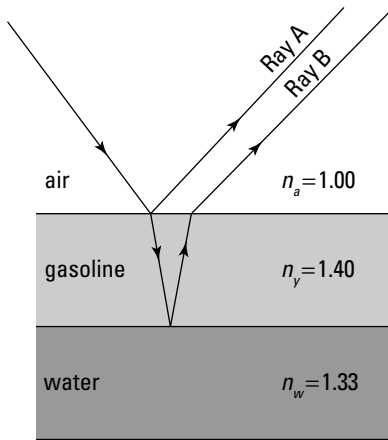
Figure 11-6: Refraction and reflection produce two parallel rays of light that interfere with each other.
