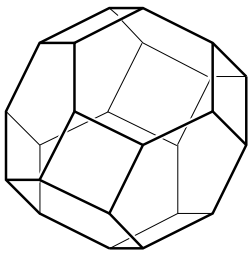
The permutahedron has 24 vertices, 36 edges and 14 facets.
