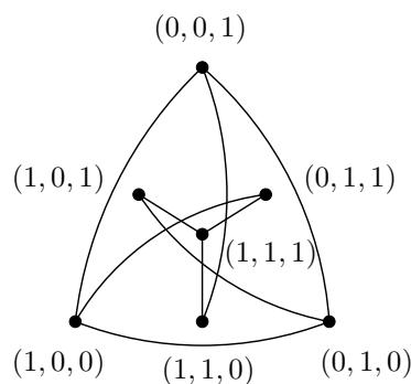
The graph G_2 : its vertices are all seven nonzero triples (x, y, z) .
