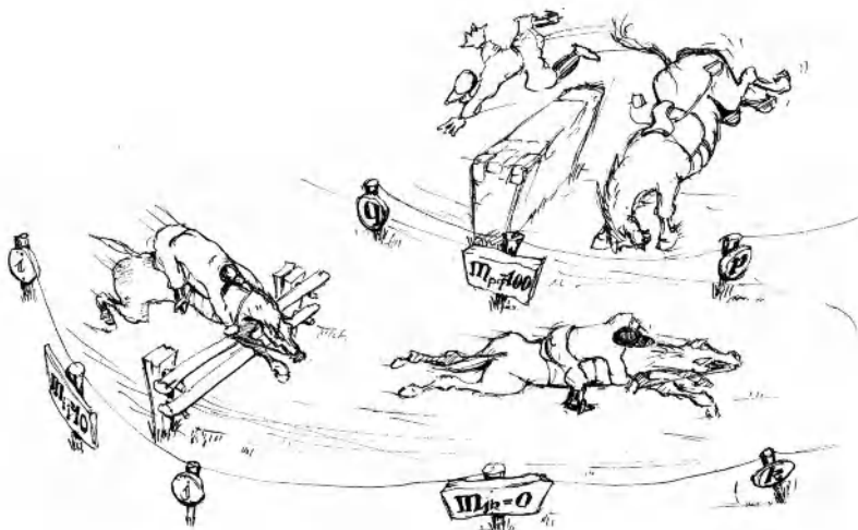
“Lattice paths”
