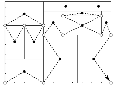
Here the bipartite graph G is drawn with vertices in C white, vertices in T black, and dashed edges.
