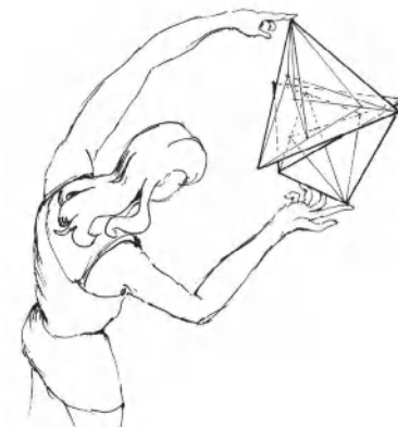
“Touching simplices”
