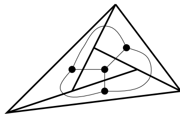
f(2) \geq 4
