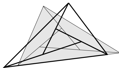
f(3) \geq 8
