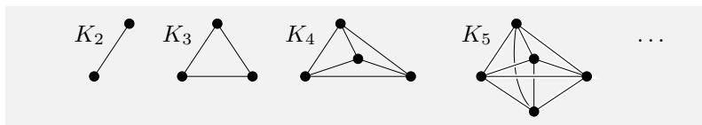
The complete graphs K_n on n vertices and \binom{n}{2} edges
