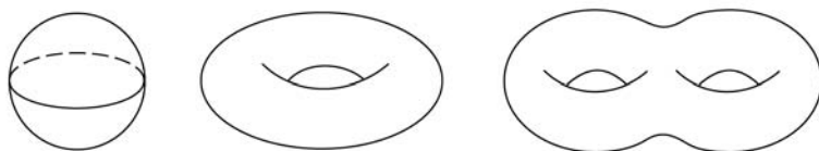
FIGURE 1. Sketches of smooth surfaces of genus 0, 1, and 2.
