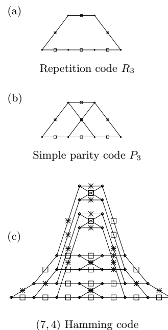
Figure 25.1. Examples of trellises. Each edge in a trellis is labelled by a zero (shown by a square) or a one (shown by a cross).
