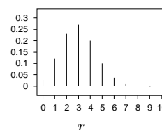
Figure 1.1. The binomial distribution P(r | f = 0.3, N = 10) .
