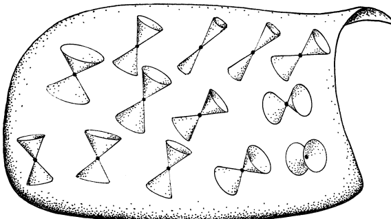
Fig. 17.17 Einsteinian spacetime \mathcal{E} of general relativity. This generalization of Minkowski’s \mathbb{M} is similar to the passage from \mathcal{G} to \mathcal{N} (Figs. 17.12, 17.3, 17.7a, respectively). As with \mathbb{M} , the Lorentzian (+ - - -) pseudo-metric g defines the physical measure of time.
