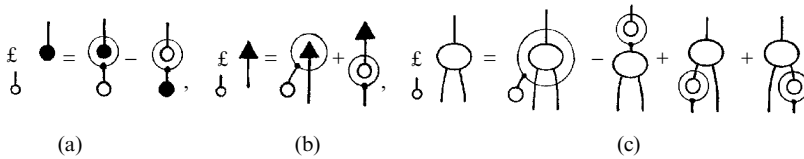
Fig. 14.17 Diagrams for Lie derivative (a) of a vector \eta: (\mathfrak{L}_\xi \eta)^a = \zeta^a \nabla_a \eta^b - \eta^a \nabla_a \zeta^b ; (b) of a covector \alpha: (\mathfrak{L}_\xi \alpha)_a = \zeta^b \nabla_b \alpha_a + \alpha_b \nabla_a \zeta^b ; and (c) of a \begin{bmatrix} 1 \\ 2 \end{bmatrix} -valent tensor Q: \mathfrak{L}_\xi Q_{ab}^c = \zeta^u \nabla_u Q_{ab}^c + Q_{ub}^c \nabla_a \zeta^u + Q_{au}^c \nabla_b \zeta^u - Q_{ab}^u \nabla_u \zeta^c .
