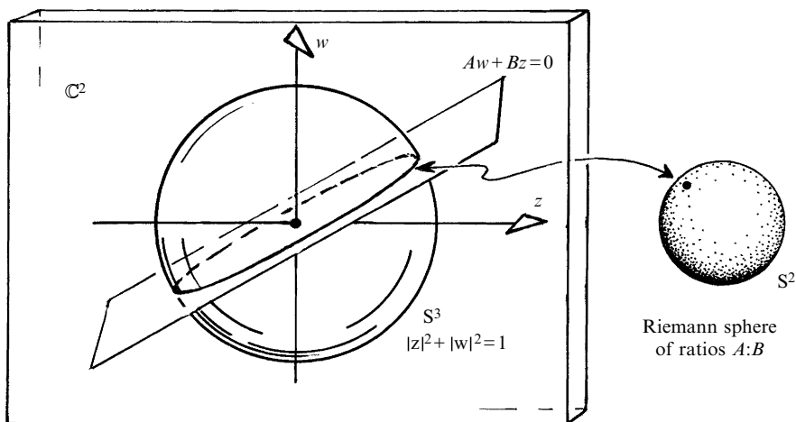
Fig. 15.8 The Clifford bundle. Take \mathbb{C}^2 with coordinates (w,z) , containing the 3-sphere \mathcal{B} = S^3 given by |w|^2 + |z|^2 = 1 . Each fibre \mathcal{V} = S^1 is the unit circle in a complex straight line through the origin Aw + Bz = 0 (complex 1-dimensional vector subspace of \mathbb{C}^2 ), and is determined by the ratio A:B . The Riemann sphere S^2 of such ratios is the base space \mathcal{B} .
