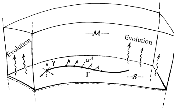
Fig. 32.1 Ashtekar's original canonical variables, defined on a spacelike 3-surface \mathcal{S} in spacetime \mathcal{M} , takes the ‘position’ parameters \boldsymbol{\Gamma} to be the components of the 4-space spin-connection, restricted to \mathcal{S} (for spinors \alpha^A , indicated by half-arrows). The ‘momentum’ parameters are basically the components of the (inverse) intrinsic metric \boldsymbol{\gamma} of \mathcal{S} (expressed as 2-forms and referred to an orthonormal basis at each point of \mathcal{S} ).
