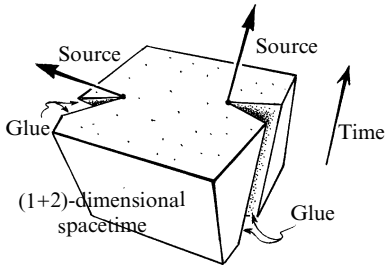
Fig. 32.9 ‘General relativity’ in 2 + 1 dimensions demands flat spacetime whenever there are no sources (since the Ricci tensor vanishes there, and the Weyl tensor always vanishes in 3 dimensions). But a source worldline provides a ‘glitch’ in the flat spacetime (a conical singularity) reminiscent of the ‘cosmic string’, whose spatial 3-geometry is illustrated in Fig. 28.4, §28.2. The source worldlines are always straight, classically, but this is relaxed in the quantum version of this theory—an example of a topological quantum field theory.
