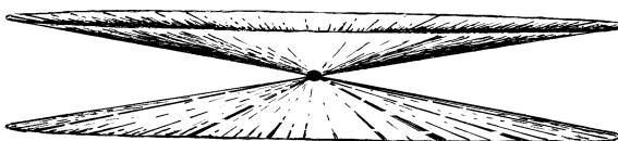
Fig. 17.14 The null cone redrawn so that the space and time scales are just slightly closer to those of normal experience.
