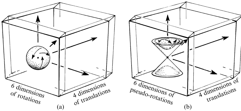
Fig. 18.3 (a) The group of Euclidean motions of \mathbb{E}^4 is 10-dimensional, the symmetry group with fixed origin being the 6-dimensional rotation group O(4) and the group of translations of the origin, 4-dimensional. (b) For the symmetries of \mathbb{M} , we get the 6-dimensional Lorentz group O(1,3) (or O(3,1) ) for fixed origin and 4-dimensions of translations, giving the 10-dimensional Poincaré symmetry group.
