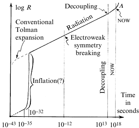
Fig. 28.12 A commonly described ‘history of the universe’, as a logarithmic plot, including an inflationary phase. Here \log R(t) is plotted against \log t .
