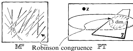
Fig. 33.14 We can obtain a ‘real’ picture of a non-null twistor Z^z by first passing to its complex conjugate Z_\alpha , thus defining a complex projective plane in \mathbb{P}^T . This plane is fixed by its intersection with \mathbb{P}\mathbb{N} , which is a 3-real-dimensional locus. This locus defines a 3-parameter family of light rays in \mathbb{M}^\# called a Robinson congruence.
