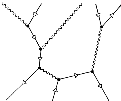
Fig. 26.8 A tree graph contains no loops. The internal momenta are consequently fixed by the external momenta, so no integration is involved. Tree graphs reproduce the classical theory.
