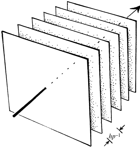
Fig. 21.6 Planes of a given phase, for a momentum eigenstate with spacing \hbar p^{-1} , where p is the magnitude of the spatial 3-momentum. (Compare Fig. 21.2.)
