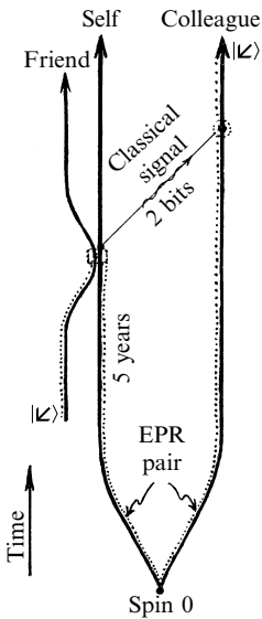
Fig. 23.7 ‘Quantum teleportation’, demonstrating the acausal propagation of quanglement. A space-time diagram illustrates the process whereby the unknown quantum state ( |\Psi\rangle ) of spin \frac{1}{2} , given to me by my friend, can be conveyed to my colleague on Titan by the mere transmission of 2 bits of classical information, provided that my colleague and I already share an EPR pair. The acausal quanglement link is depicted as a dotted path.
