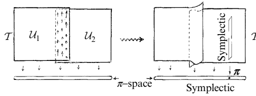
Fig. 33.25 Apply the idea of Fig. 33.24 in case of the twistor description of anti-self-dual gravity (with two patches). The vector field is (\partial f/\partial\omega^0)\partial/\omega^1 - (\partial f/\partial\omega^1)\partial/\omega^0 , with f homogeneous of degree 2. We get a curved twistor space (portion) \mathcal{T} . There is a global projection of \mathcal{T} to the \pi -space. Each fibre of this projection is a complex symplectic 2-space, as is the \pi -space itself.
