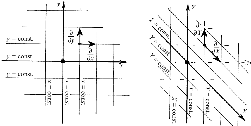
Fig. 10.7 Second fundamental confusion of calculus is illustrated: \partial/\partial X \neq \partial/\partial x despite X = x , and \partial/\partial Y \neq \partial/\partial y despite Y = y , for the coordinate change X = x , Y = y + x . The interpretation of partial differential operators as ‘arrows’ pointing along coordinate lines clarifies the geometry ( x = \text{const.} agree with X = \text{const.} , but y = \text{const.} disagree with Y = \text{const.} ).
