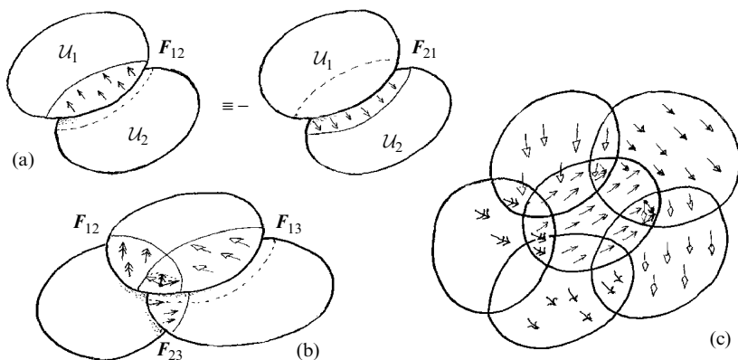
Fig. 33.18 The vector fields F_{ij} are subject to certain requirements. (a) On the intersection of \mathcal{U}_j with \mathcal{U}_i , we have F_{ji} = -F_{ij} . This is illustrated as the movement of \mathcal{U}_1 over \mathcal{U}_2 , as shown by the vector F_{12} on \mathcal{U}_1 . But the same relative movement is achieved by the negative of this on \mathcal{U}_2 . (b) The triple overlap condition F_{ij} + F_{jk} = F_{ik} is illustrated. On the triple intersection of \mathcal{U}_1, \mathcal{U}_2 , and \mathcal{U}_3 , the motion F_{12} of \mathcal{U}_1 over \mathcal{U}_2 is the sum of the motion F_{13} of \mathcal{U}_1 over \mathcal{U}_3 and the motion F_{32} of \mathcal{U}_3 over \mathcal{U}_2 . (c) If all the patches are shunted individually in their entirities, this has no effect (except for a coordinate change in each patch). This illustrates that the overall shunt F_{ij} = H_i - H_j counts for nothing and must be ‘factored out’.
