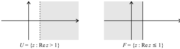
FIGURE 1.5. Open and non-open sets.
