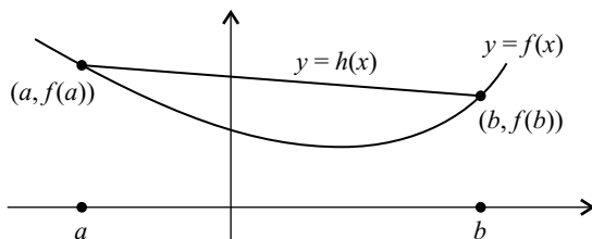
FIGURE 7.2. A convex function.
