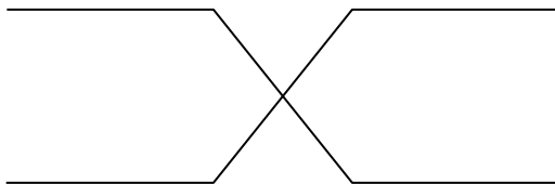
FIGURE 9.12. Idealized picture of a Riemann surface.
