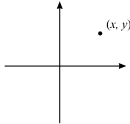
FIGURE 1.1. The plane \mathbb{R}^2 .
