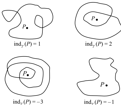
FIGURE 4.5. The concept of index.
