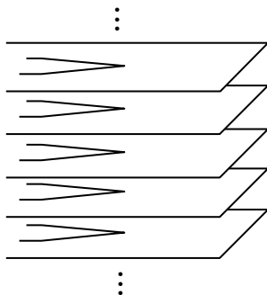
FIGURE 9.14. The Riemann surface for the logarithm.
