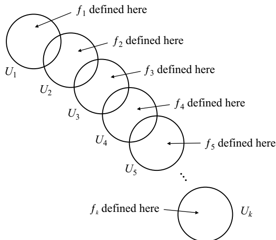
FIGURE 9.6. Analytic continuation of a function element.
