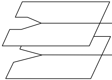
FIGURE 9.11. Forming a Riemann surface.
