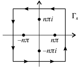
FIGURE 4.12. The contour in Subsection 4.5.7.
