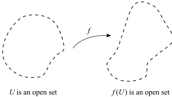
FIGURE 5.3. The open mapping principle.
