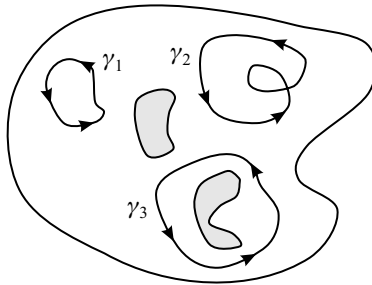
FIGURE 2.5. Deformation of curves.
