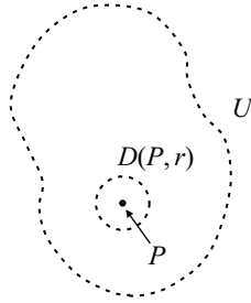
FIGURE 1.4. An open set.
