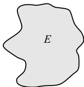
FIGURE 3.1. A compact set.
