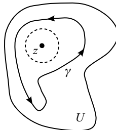
FIGURE 2.4. General form of the Cauchy formula.
