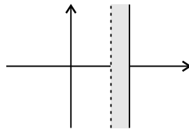
FIGURE 1.6. A set that is neither open nor closed.
