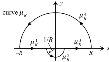
FIGURE 4.9. An altered contour for the integral in Subsection 4.5.4.
