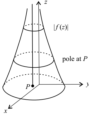
FIGURE 4.3. A pole.
