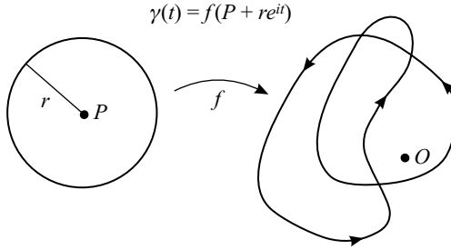
FIGURE 5.2. The argument principle.
