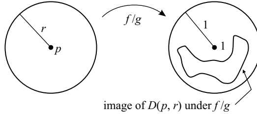
FIGURE 5.4. Rouché's theorem.
