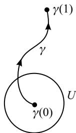
FIGURE 9.7. Analytic continuation along a curve.
