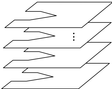
FIGURE 9.13. The Riemann surface for \sqrt[n]{z} .
