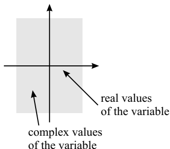
FIGURE 3.4. Principle of persistence of functional relations.
