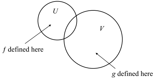
FIGURE 9.5. Direct analytic continuation.
