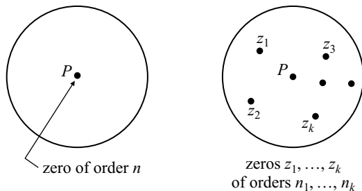
FIGURE 5.1. Counting the zeros of a holomorphic function.
