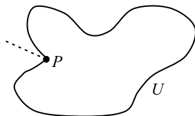
FIGURE 7.3. The concept of a barrier.
