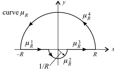
FIGURE 4.8. The contour in Subsection 4.5.4.
