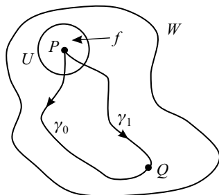
FIGURE 9.10. The concept of monodromy.
