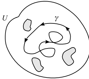
FIGURE 2.3. General form of the Cauchy theorem.
