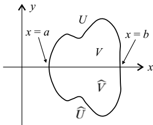
FIGURE 7.1. Schwarz reflection.
