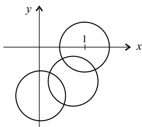
FIGURE 9.4. Analytic continuation in the other direction.
