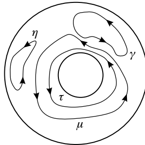
FIGURE 9.9. The concept of homotopy.
