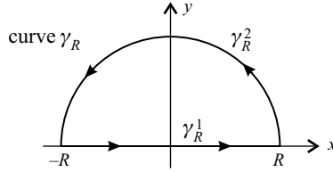
FIGURE 4.6. The contour in Subsection 4.5.2.
