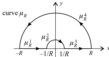
FIGURE 4.10. The contour in Subsection 4.5.5.
