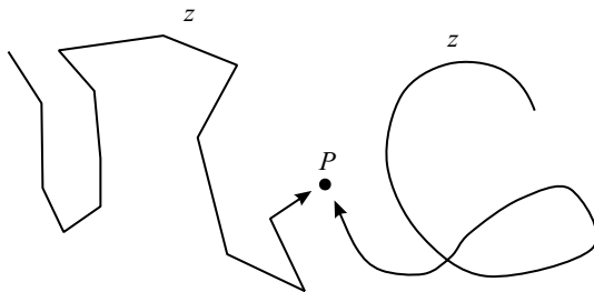
FIGURE 1.12. The limit from any direction.
