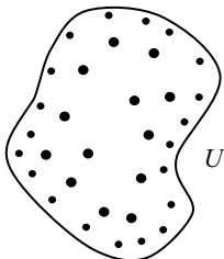
FIGURE 8.1. Any domain in \mathbb{C} is a domain of holomorphy.
