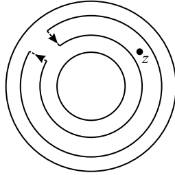
FIGURE 4.2. The Cauchy integral on an annulus.
