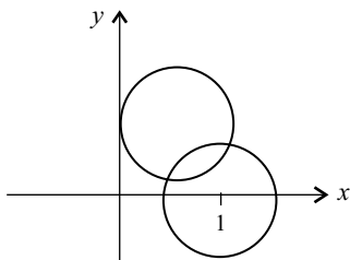
FIGURE 9.1. Analytic continuation to a second disc.
