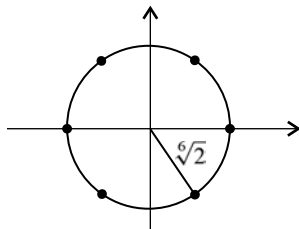
FIGURE 1.10. The sixth roots of 2.
