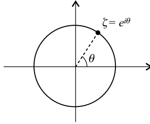
FIGURE 1.9. Polar representation of a complex number of modulus 1.
