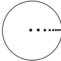
FIGURE 3.3. Zeros accumulating at a boundary point.
