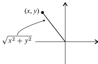
FIGURE 1.2. Euclidean distance (modulus) in the plane.
