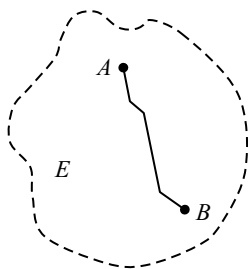
FIGURE 1.7. The concept of connectivity.
