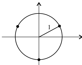
FIGURE 1.11. The third roots of i .
