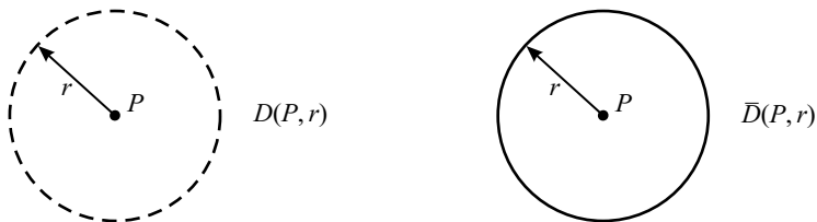
FIGURE 1.3. Open and closed discs.
