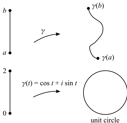
FIGURE 2.1. Curves in the plane.
