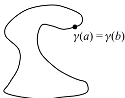
FIGURE 2.2. A simple, closed curve.
