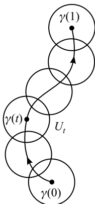
FIGURE 9.8. Direct analytic continuation.
