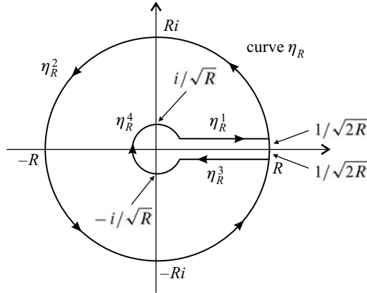
FIGURE 4.11. The contour in Subsection 4.5.6.
