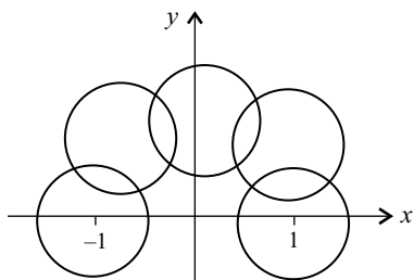
FIGURE 9.3. Analytic continuation of the square root function.
