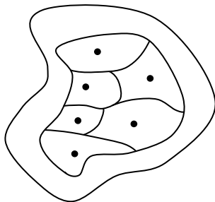
FIGURE 4.4. Reduction to simpler curves.
