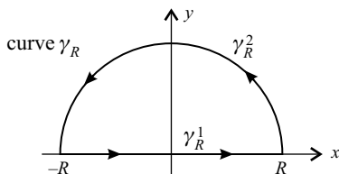
FIGURE 4.7. The contour in Subsection 4.5.3.
