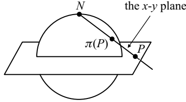
FIGURE 6.1. Stereographic projection.
