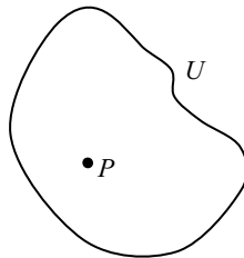
FIGURE 4.1. An isolated singularity.
