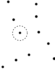
FIGURE 3.2. A discrete set.
