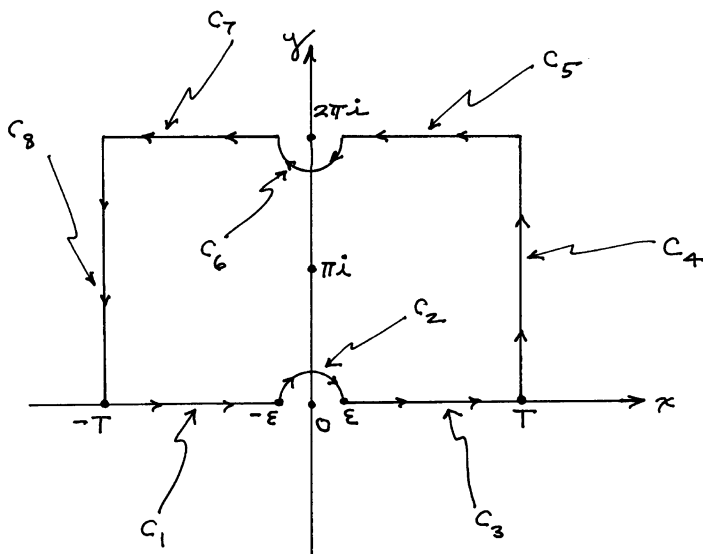
Fig. 8.6.3 A curious contour
