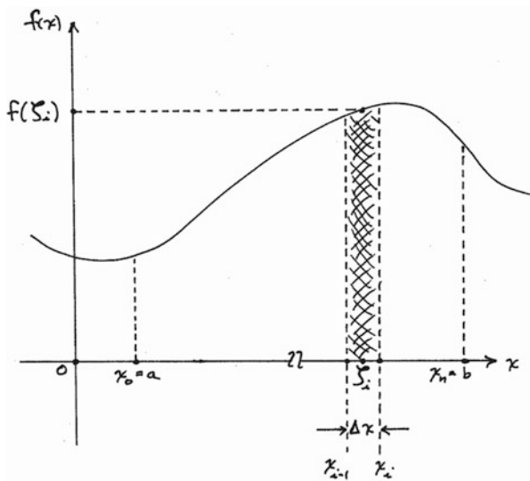
Fig. 1.1.2 Approximating the 'area under the curve'
