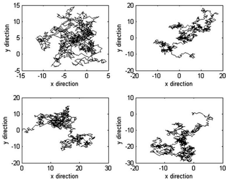
Fig. 1.8.2 Typical paths of two-dimensional Brownian motion (each 1,000 steps)
