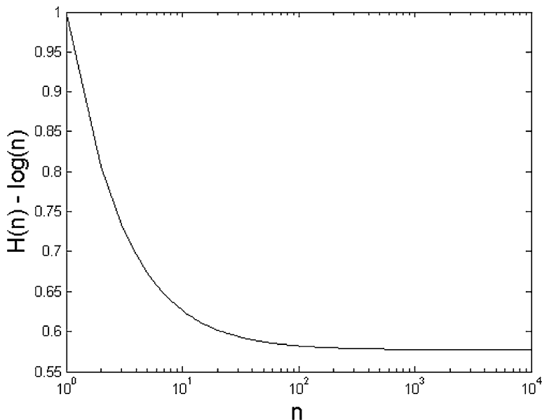
Fig. 5.4.1 Euler's constant as a limit
