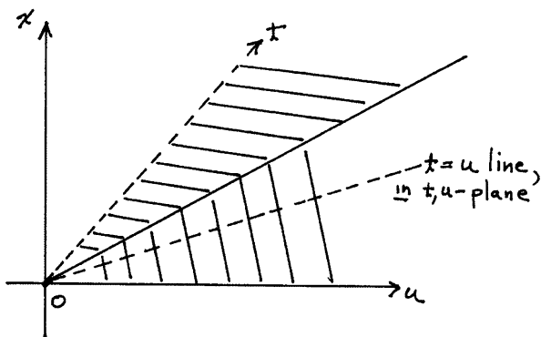
Fig. 6.4.3 The foot of the wedding cake at the origin
