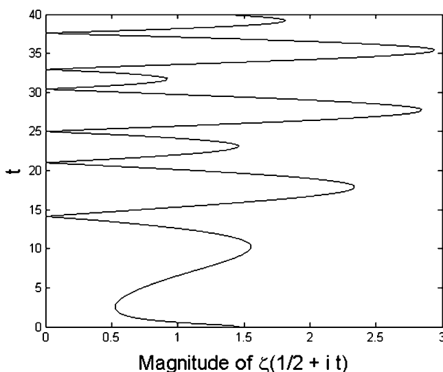
Fig. 9.1.2 The first six non-trivial zeros of \zeta(\frac{1}{2} + it)
