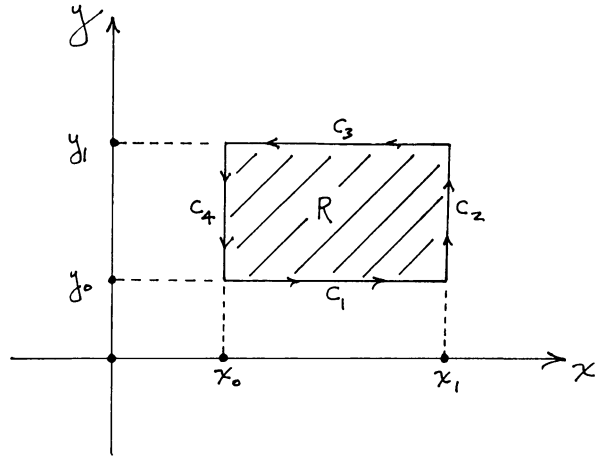
Fig. 8.5.2 When R is a rectangle
