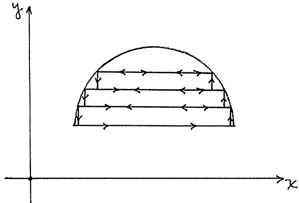
Fig. 8.5.3 Making a half-disk out of many thin rectangles
