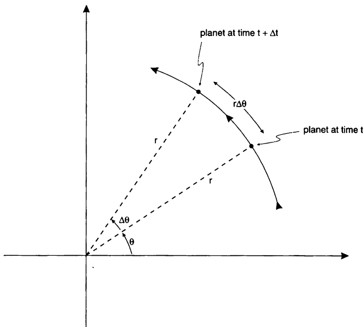
Fig. 8.3.1 Interpreting r^2 \frac{d\theta}{dt}
