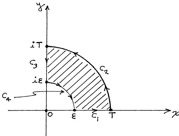
Fig. 8.6.1 A contour that avoids a singularity at the origin
