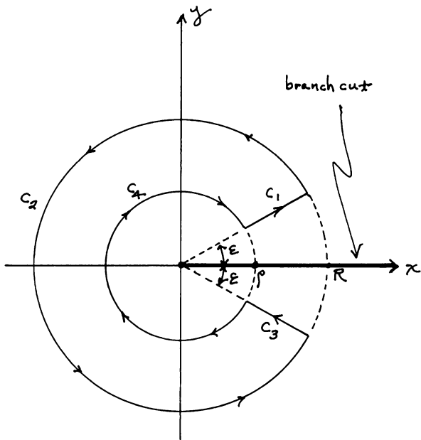
Fig. 8.9.1 A closed contour that avoids crossing a branch cut
