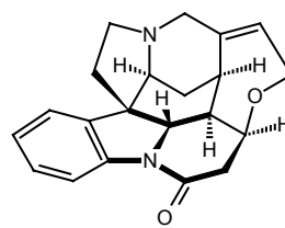
Strychnine (Woodward, 1954)
