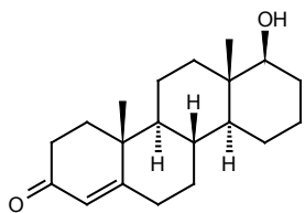
D-Homotestosterone
