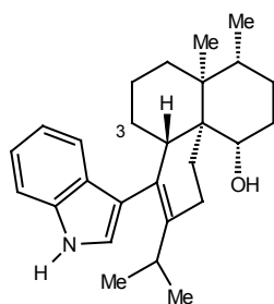
3-Desmethylaflavinine
