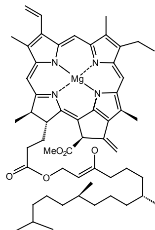
Chlorophyll (Woodward, 1960)
