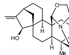
Veatchine
