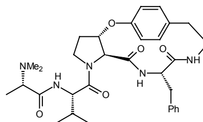
Dihydropauritine A
