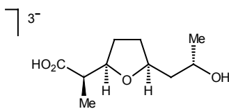
(-)-Nonactic Acid
