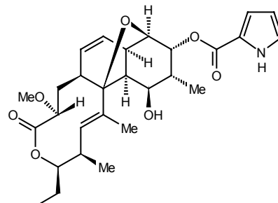
(+)-18-Deoxynargenicin A 1
