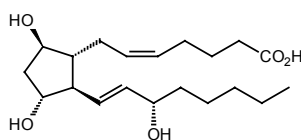
PGF 2β
