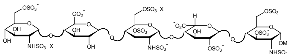
Heparin-Like Pentasaccharide
