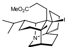
(+)-Methyl Homodaphniphyllate
