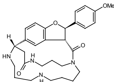
O-Methylorantine
