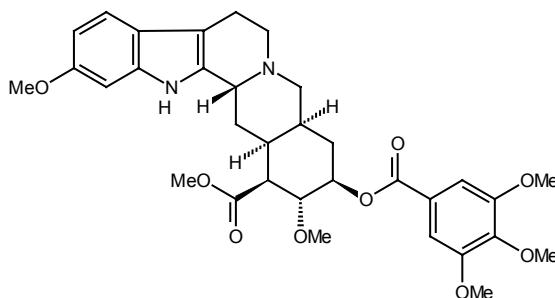
Reserpine (Woodward, 1956)
