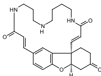
Lunarine
