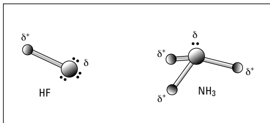
Figure 6-11: Polar covalent bonding in HF and \text{NH}_3 .
