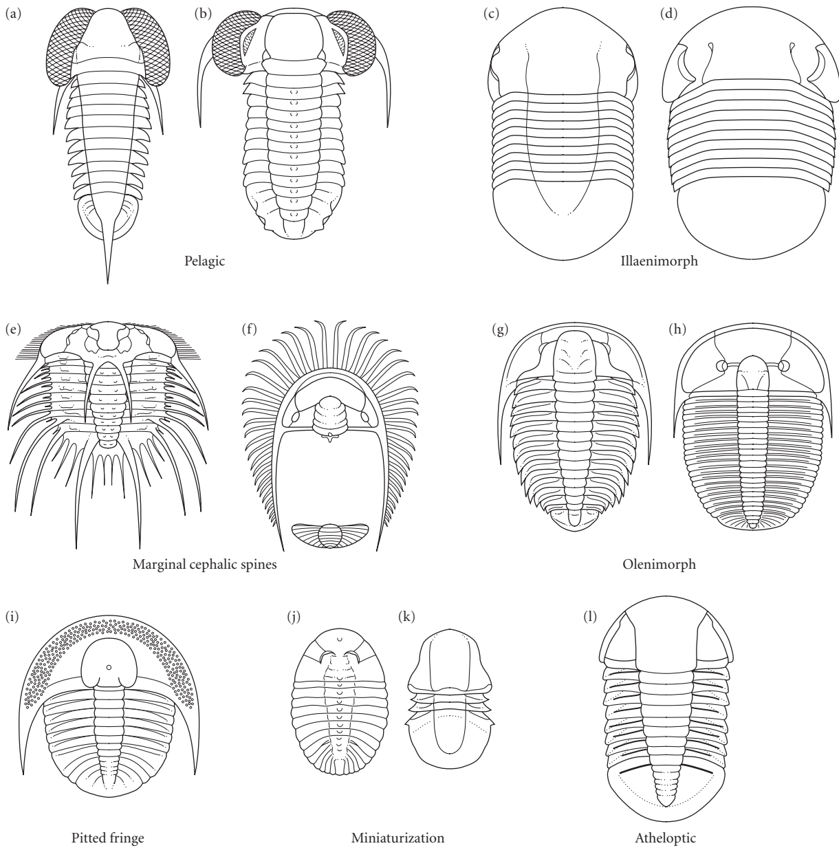
Figure 14.8 Trilobite ecomorphs: pelagic (a, b), illaenomorph (c, d), marginal cephalic spines (e, f), olenimorph (g, h), pitted fringe (i), miniature (j, k) and atheloptic (blind) (l) morphotypes. (Based on Fortey & Owens 1990.)
