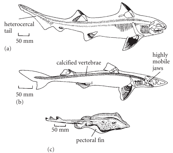
Figure 16.11 Sharks and rays, ancient and modern: (a) the Jurassic shark Hybodus ; (b) the modern shark Squalus ; and (c) the modern ray Raja . (Based on various sources.)
