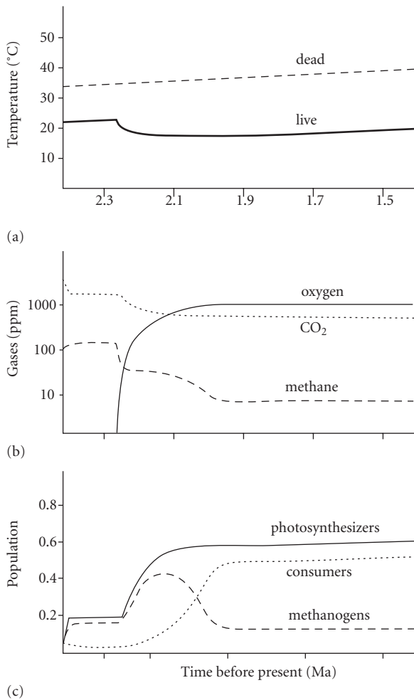
Figure 4.28 Precambrian Gaia and evolution of the biosphere. (a) Changes in climate in a live and lifeless world; there is a sharp fall in temperature when oxygen appears. (b) The changing abundance in atmospheric gases. (c) Changes in the composition of ecosystems: both the photosynthesizers and methanogens increase initially when oxygen appears but the methanogens eventually decline to a much lower level of abundance. (Population is the proportion of the total population in tenths.) (From Lovelock 1998.)
