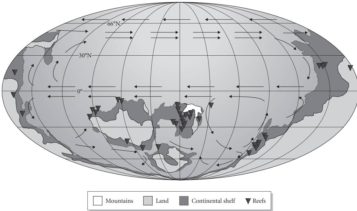
Figure 11.13 Paleogeographic range of Early Cambrian archaeocyathid reefs. (Replotted from Debrenne 2007.)
