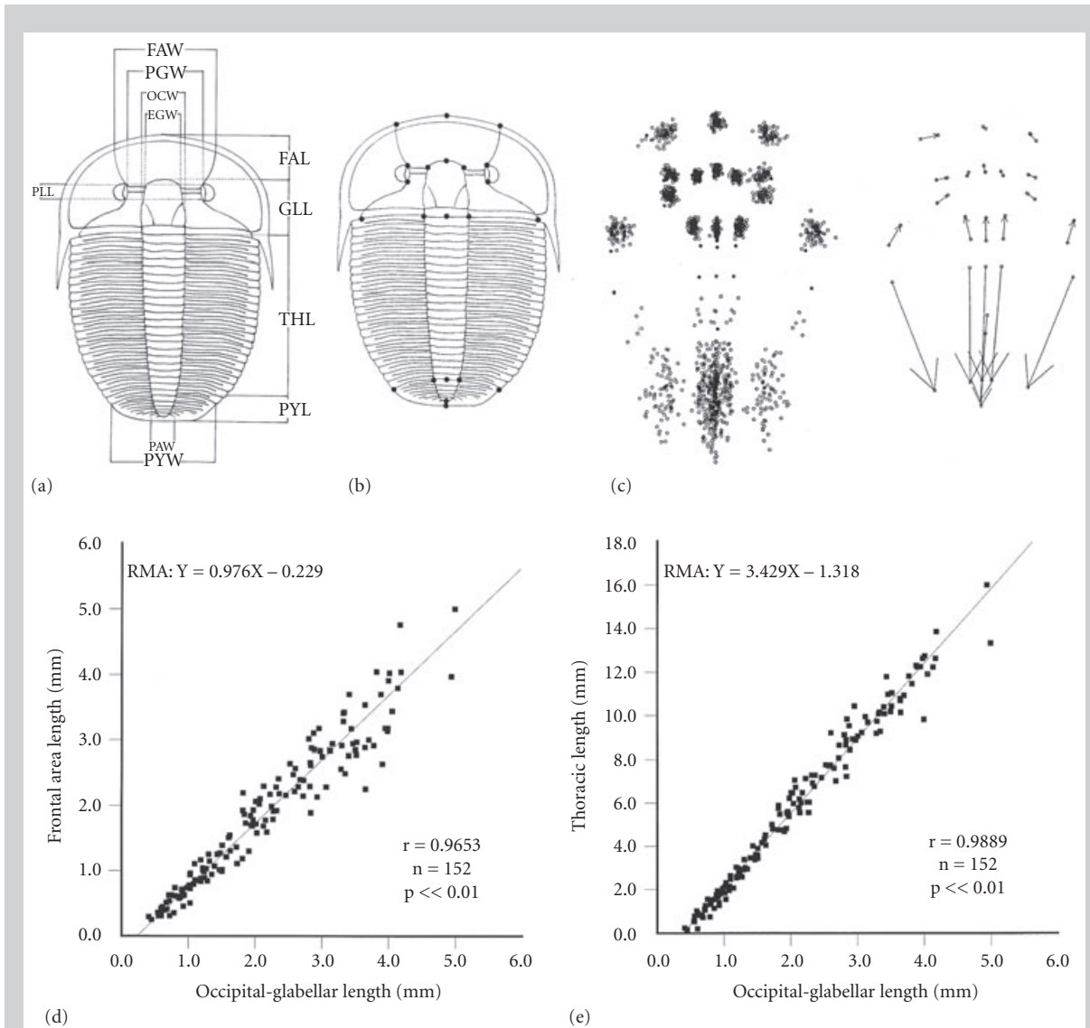
Figure 14.12 Landmark analysis of Aulacopleura . (a) Measurements, (b) landmarks, (c) plot of landmarks, (d) bivariate plot of occipital–glabella length versus frontal area length, and (e) bivariate plot of occipital–glabella length versus thoracic length. FAW, width of frontal area; PGW, OGW, width of occipital glabella; EGW, FAL, length of frontal area; PLL, GLL, THL, length of thorax; PYL, length of pygidium; PAW, PYW, width of pygidium; RMA, reduced major axis. (Courtesy of Nigel Hughes.)
